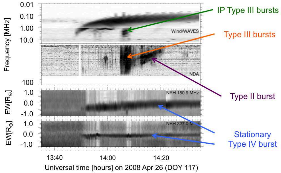
FIGURE 2.10: Dynamic spectra and 1D images of the event on 2008 April 26 showing the three types of radio bursts more relevant in space weather. Two bottom panels are 1D images projected onto the solar east-west direction at 150 and 327 MHz (y axis graded in solar radii from the eastern to the western limb). Two top panels show the dynamic spectra between 70 MHz and 10 kHz.
