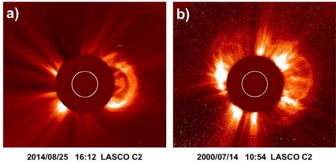
FIGURE 1.2: Snapshot images by LASCO C2 showing a) a partial halo CME and b) a halo CME. Images from SoHO LASCO CME catalog 2 .
