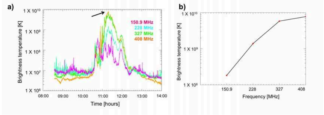
FIGURE 3.23: a) Brightness temperature profile as a function of time within the region where the radio sources were observed. The colours represent the different frequencies. b) Brightness temperature spectrum at the peak marked by the black arrow in a).
