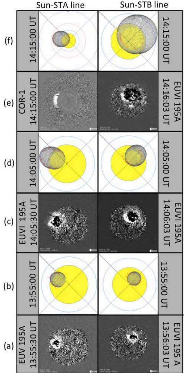
Fig. 7. Comparison of running-difference images (rows a ), c ), e ) of the eruptive event observed by STA (left hand-column) and STB (right hand column) with the results of applying the fitting technique (rows b ), d ), f ) developed by Rouillard et al. (2016). The images are all from the EUVI instruments, except the left-hand image shown in row f ) obtained by COR1-A. Red crosses superposed on the fitted ellipsoids show the contour of the propagating front observed in the running difference images and are used to constrain the extent and location of the ellipsoid at each time.
