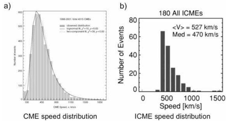
FIGURE 4.8: Distributions of CME speeds and ICME speeds. a) Distribution of the observed speeds of 4315 CMEs with a bin size of 70 \text{ km s}^{-1} . Figure adapted from Yurchyshyn et al. [2005] . b) Distributions of 180 ICMEs with a bin size of 100 \text{ km s}^{-1} . Figure adapted from Gopalswamy [2010] .
