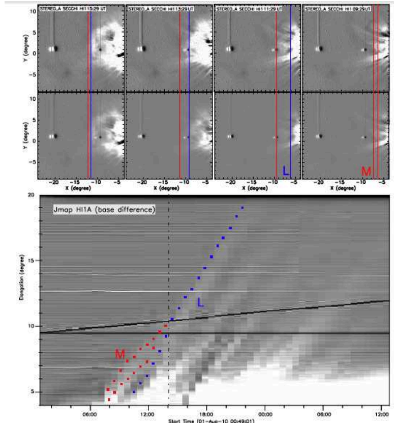
FIGURE 4.10: Top: base difference images from HI-A showing the evolution of two CMEs (denoted as M and L) in a distance range of 20-40 R_{\odot} . The fronts of M and L are indicated by red and blue lines respectively. Bottom: J-map constructed from base difference images and overplotted tracks of both CMEs (squares). Figure from Temmer et al. [2012] .
