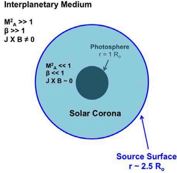
FIGURE 4.6: Schematic regions of the corona and the values of M_A and \beta in each region. The source surface is plotted as a contour in blue. Figure adapted from Cravens [1997].
