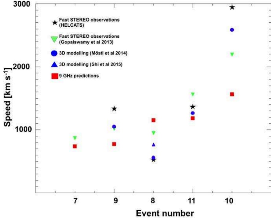
Fig. 5. Observed and predicted CME speeds. The black stars represent the higher of the two CME speeds derived from a geometric fit of observations from each of the two STEREO spacecraft (HELCATS catalogue). The green inverted triangles show the higher of the two CME speeds measured in the STEREO/COR2 images by Gopalswamy et al. (2013) . The blue circles and blue triangles are the speeds resulting from multi-spacecraft modeling by Möstl et al. (2014) and Shi et al. (2015) . The red filled squares denote the speeds found from the microwave fluence by using least squares (LS) fitting.
