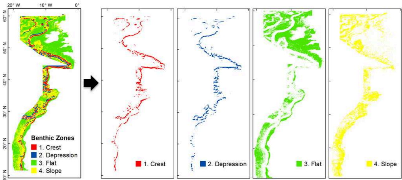
Figure 3-11: Benthic Zones.
