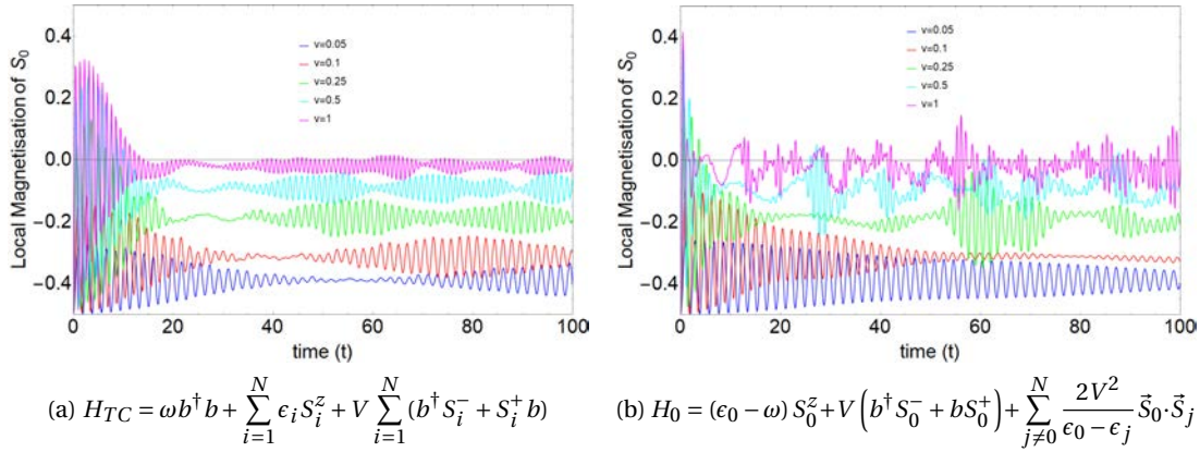
Figure 5.3: Evolution of the local magnetisation S_0^z as a function of the time for a variety of coupling constants V governed either by H_{TC} or H_0 . The initial state is |\downarrow\uparrow\downarrow\downarrow\downarrow\downarrow\downarrow\rangle and the bosonic mode is set at \omega = 2.99 in every case.
