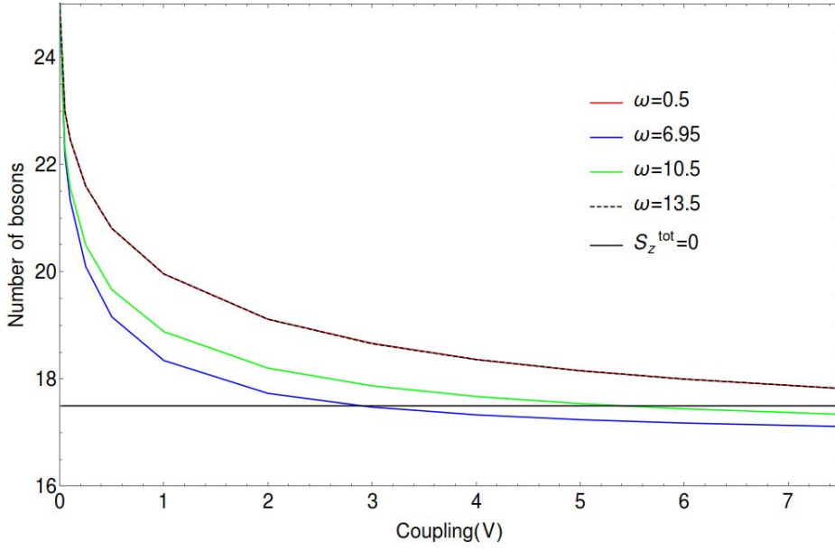
Figure 4.6: Bosonic occupation in steady states for the initial state: |25; \downarrow\downarrow\downarrow\downarrow\downarrow\downarrow\downarrow\downarrow\downarrow\downarrow\downarrow\downarrow\rangle for a variety of coupling constants V . The total number of excitations is M = 25 and the bosonic frequency are set to \omega = 0.5, 6.95, 10.5, 13.5 .
