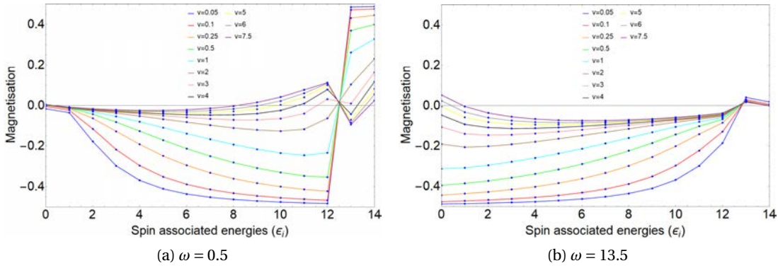
Figure 4.10: Local magnetisation in steady-states for two initial states for a variety of coupling constants V : |\downarrow 23; \downarrow \downarrow \downarrow \downarrow \downarrow \downarrow \downarrow \downarrow \downarrow \downarrow \downarrow \downarrow \downarrow \downarrow \uparrow \uparrow \rangle in both case but for two different bosonic frequencies. The total number of excitations is M = 25 .
