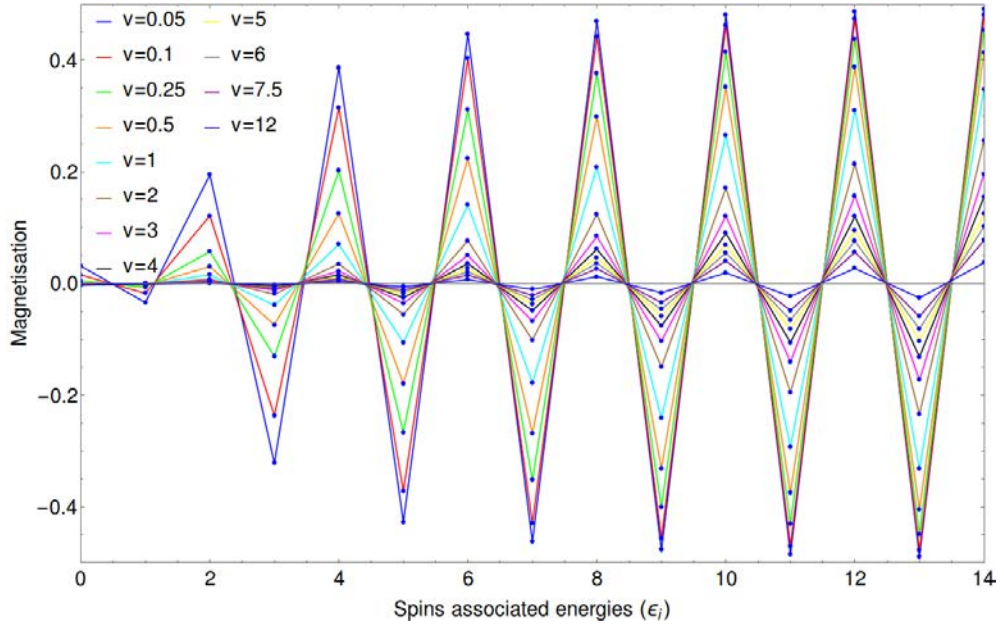
Figure 4.7: Local magnetisation in the steady state for the initial state: |\uparrow\downarrow\uparrow\downarrow\uparrow\downarrow\uparrow\downarrow\uparrow\downarrow\uparrow\downarrow\uparrow\downarrow\rangle for a variety of coupling constants V . The total number of excitations is M = 25 and the bosonic frequency is set to \omega = 0.5 , near an edge of the energy band.
