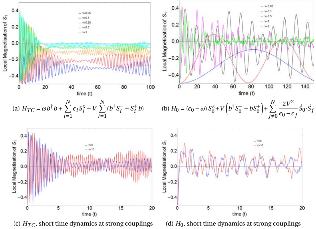
Figure 5.4: Evolution of the local magnetisation S_1^z as a function of the time for a variety of coupling constants V governed either H_{TC} or H_0 . The initial state is |13; \downarrow\downarrow\downarrow\downarrow\downarrow\rangle and the bosonic mode is set at \omega = 2.99 in every case.
