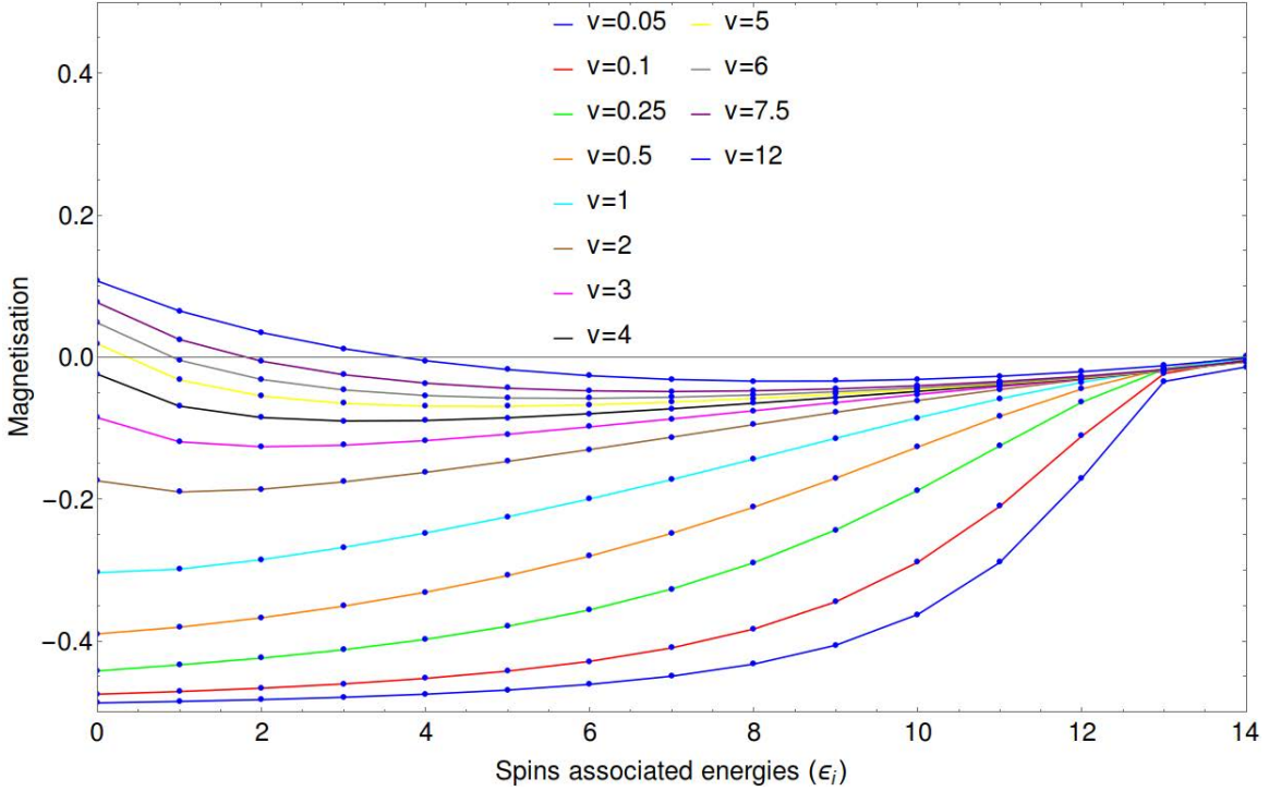
Figure 4.3: Local magnetisation in the steady-state for the initial state: |25; \downarrow\downarrow\downarrow\downarrow\downarrow\downarrow\downarrow\downarrow\downarrow\downarrow\downarrow\downarrow\downarrow\rangle as a function of V . The total number of excitations is M = 25 and the bosonic frequency is set to \omega = 13.5 near the maximum of the energy band.
