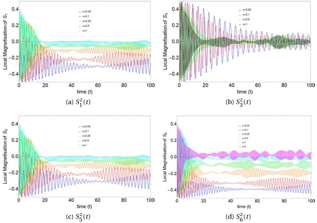
Figure 5.2: Evolution of the local magnetisation of four different spins as a function of the time for a variety of coupling constants V governed by H_{TC} . The initial state is |\downarrow\uparrow\downarrow\downarrow\downarrow\downarrow\downarrow\rangle and the bosonic mode is set at \omega = 2.99 in every case.
