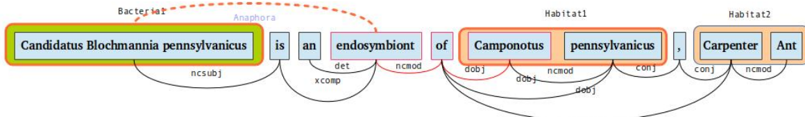
(c) The Dependency Graph with the Path of the candidate "Localization" relation between Bacteria1 and Habitat1, on "sentence2", highlighted in red.
