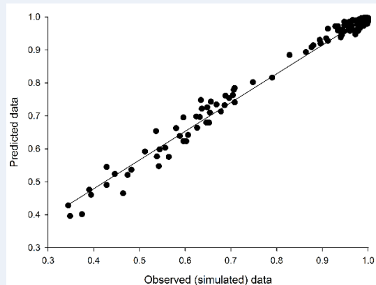
Figure 1. Predicted values (obtained by a logistic regression) vs observed data (obtained with MarCPFS simulations). Fitted line: y = 0.8713x + 0.1306 ( R^2 = 0.987 ).
