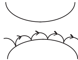
Figure 6.5 – Effect of magnetic field on backscattering.
