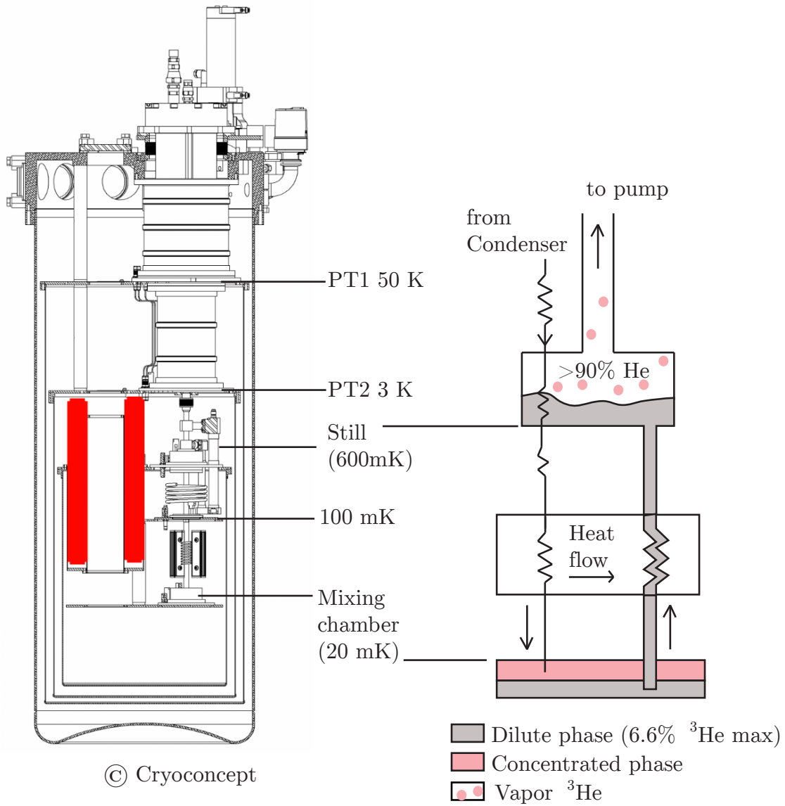
Figure 2.6 – Dilution Refrigerator schematic. A sectional view of the DR is represented on the left. The 7 T coil is shown in red. A detailed schematic of the last step of the cooling where ^3\text{He} is forced to enter the dilute phase is shown on the right.
