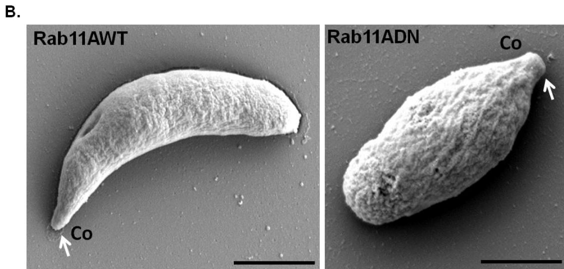
Figure 9. Cortical integrity and recruitment of glideosome components on extracellular parasites (A) IFA performed on Rab11A WT and Rab11A DN parasites fixed during the invasion process. The panel on the left shows Rab11A WT parasites fixed after 2 minutes following inoculation onto HFF monolayers. SAG1 staining (blue) prior to permeabilization reveals a faint signal in Rab11A WT parasites, which have either already invaded or in the process of invasion. In the panel on the right, extracellular Rab11A DN parasites reveal a SAG1 signal (although patchy) even after 5 minutes of inoculation onto host cells. , GAP45 and MLC1 stainings (green) allowed the detection of the glideosome components, which appear normally distributed in both the strains, while tubulin, representing the cortical cytoskeleton, showed a patchy distribution in Rab11A DN parasites. – The Rab11A signal (red) appeared as vesicles in the Rab11A WT and diffused cytosolic distribution in the Rab11A DN parasites. Scale bar = 2 \mu m. (B) Scanning electron micrographs reveal morphological defects in Rab11A DN parasites. The conoid (Co) is indicated by an arrow. Scale bar = 2 \mu m.
