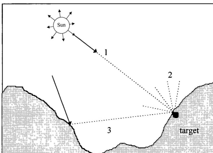
Figure 1. 19: Downward irradiance received in a mountainous region (1) direct irradiance,(2) diffuse irradiance from the sky, and (3) terrain reflected irradiance Source: (Kondrat'Yev, 2013)
