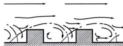
Figure 1. 17: The wake interference flow Source: Based on Oke (1988)
