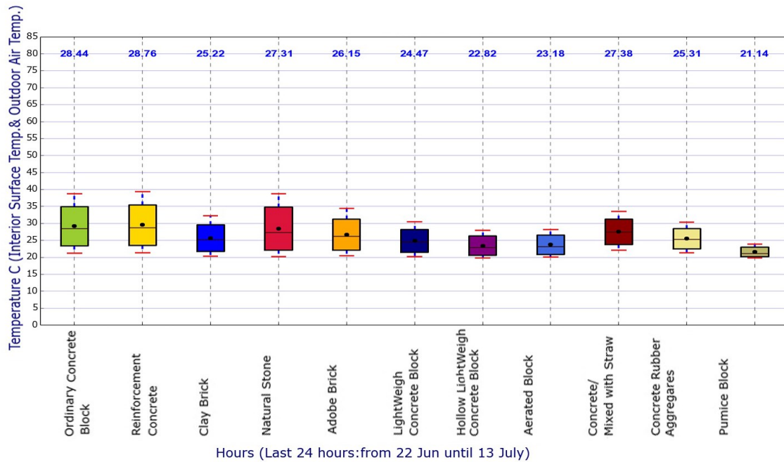
Figure 6. 21: Interior surface temperature of different materials selected | Preliminary perception of the materials performance
