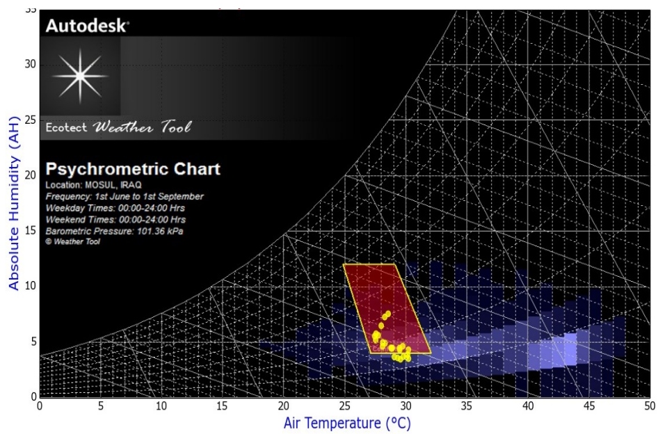
Figure 6. 70:Psychrometric chart of proposed scenario
