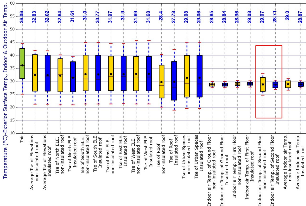
The Period of Simulation From 22 Jun-13 July with Focusing On 13 July
