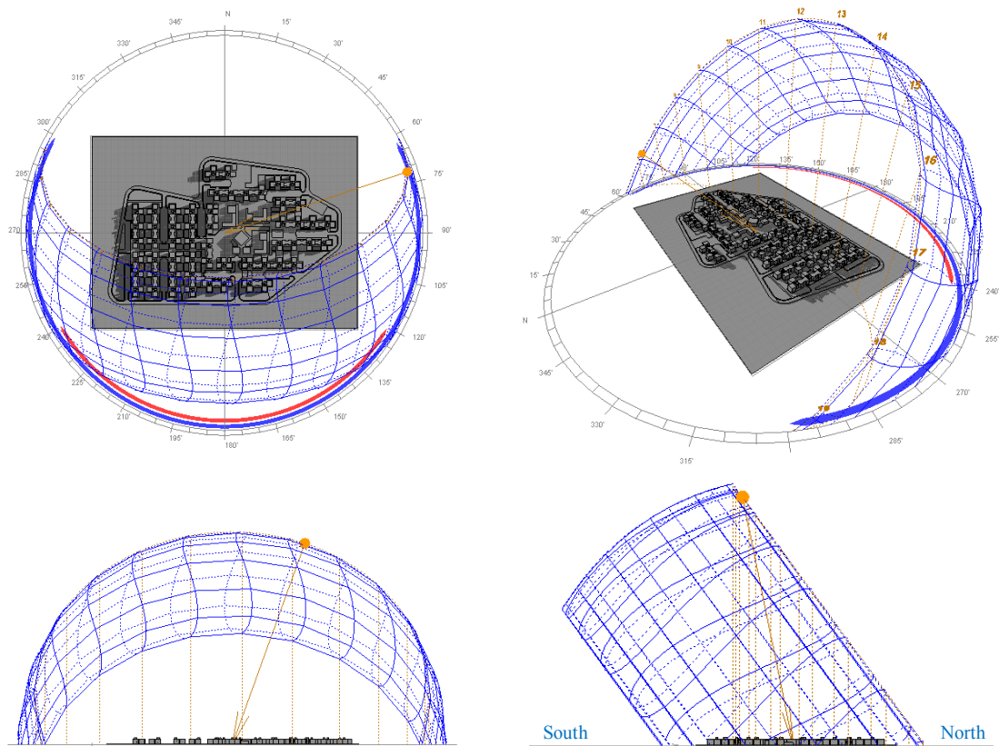
Figure 4. 26: The sun path of Mosul city
