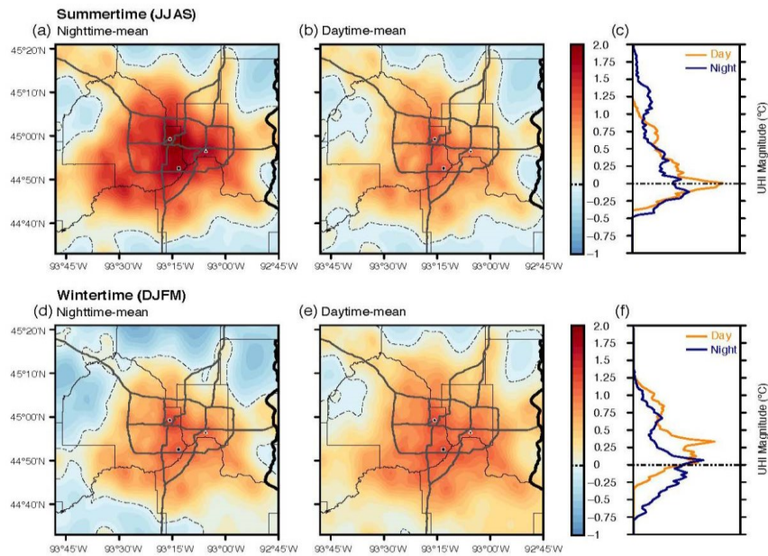
Figure 2. 7: The urban heat island averaged over nighttime and daytime, by season
