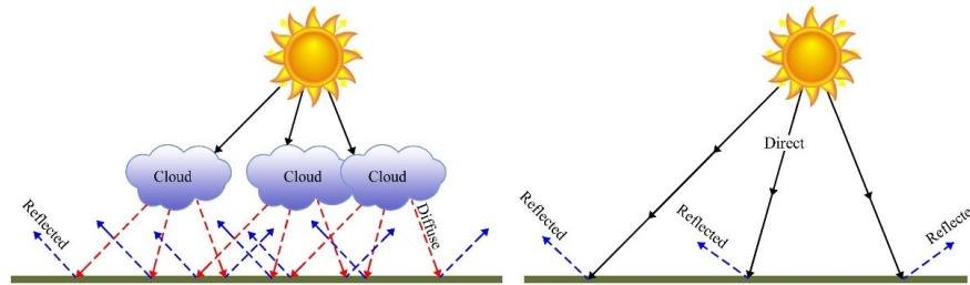
Figure 1. 22: The influence of the atmosphere Source: Adapted by (Sen, 2008)
