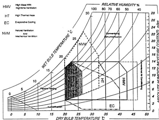
Figure 2. 14: Givoni's building bioclimatic chart Source: (Sayigh and Marafia, 1998)
