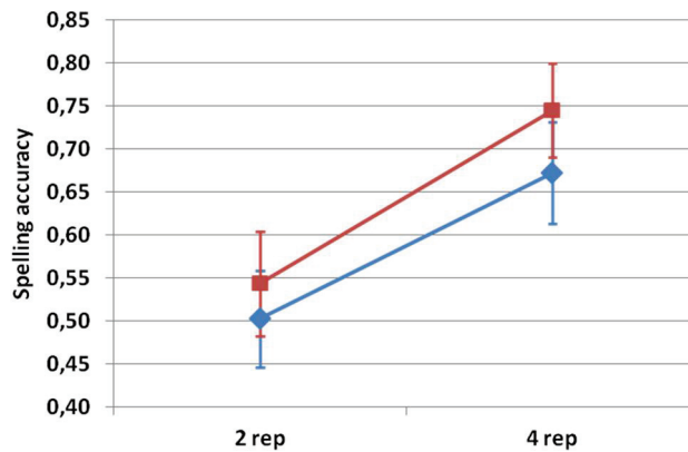
Figure 6. Spelling accuracy using an optimal selection of 9 sensors, as a function of the number of repetitions (2 or 4), for SRS (blue diamonds) and DRS (red squares). Error bars indicate the standard error of the mean.
