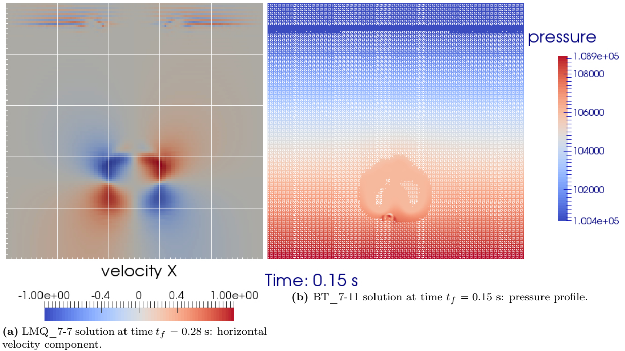
Figure 9.18: Rising bubble test: issues of the low-Mach correction (upper figure) and AMR solutions.
