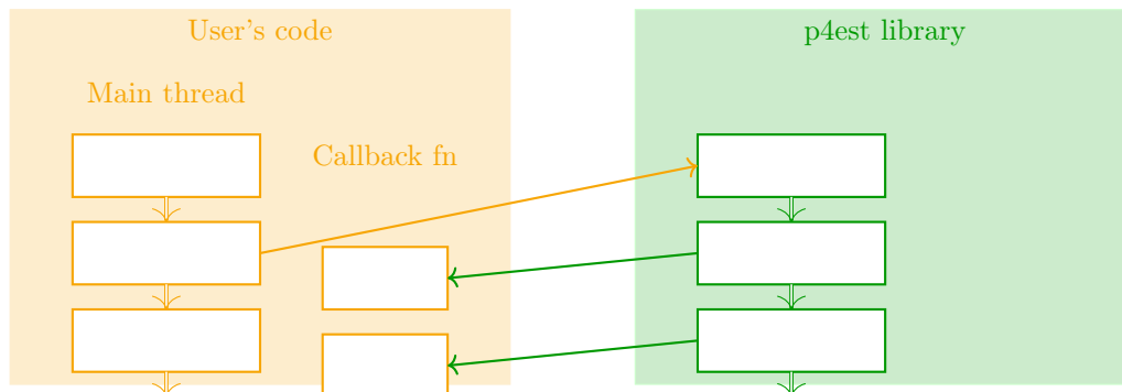
Figure 7.8: Sketch of the interactions between the user's code and p4est library. Simple arrows stand for the calls of one function to another. Double arrows stand for the progression of the computation.
