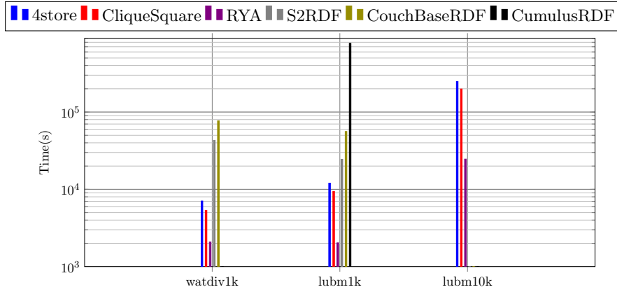
Figure 4.1: Preprocessing Time.
