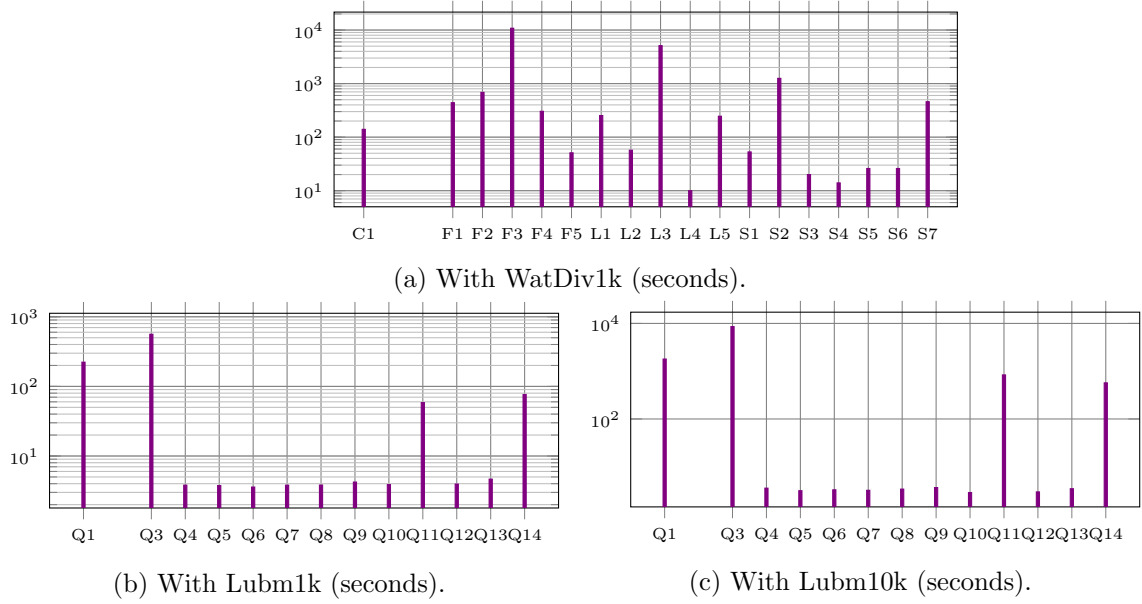
Figure 4.5: RYA Performance.
