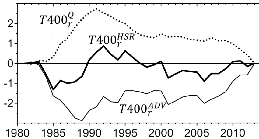
Figure 4.27. Area averaged reconstructed T400 time series obtained from annual averaged HSR ( T400_r^{HSR} , thick line), Q_{net} ( T400_r^Q , dotted line), and ADV ( T400_r^{ADV} , thin line) in the KOE region with a unit of °C.
