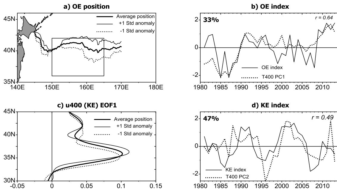
Figure 4.17. First EOFs (left panels) and corresponding PC time series (right panels) of (a–b) the latitudes of maximum meridional SST gradient representing the OE and (c–d) the zonal mean ( 145^{\circ} – 170^{\circ} E) zonal velocity averaged from the surface to the 400 m (u400) representing the KE. The mean position of OE is shown with a thick solid line in (a) together with their \pm 1 standard deviations with thin solid and dotted lines. The T400 PC1 from Figure 4.1b (dotted line) is overlaid in (b). The mean position of KE is shown with thick solid line in (c) together with their \pm 1 standard deviations with thin solid and dotted lines. The T400 PC2 from Figure 4.1d (dotted line) is overlaid in (d).
