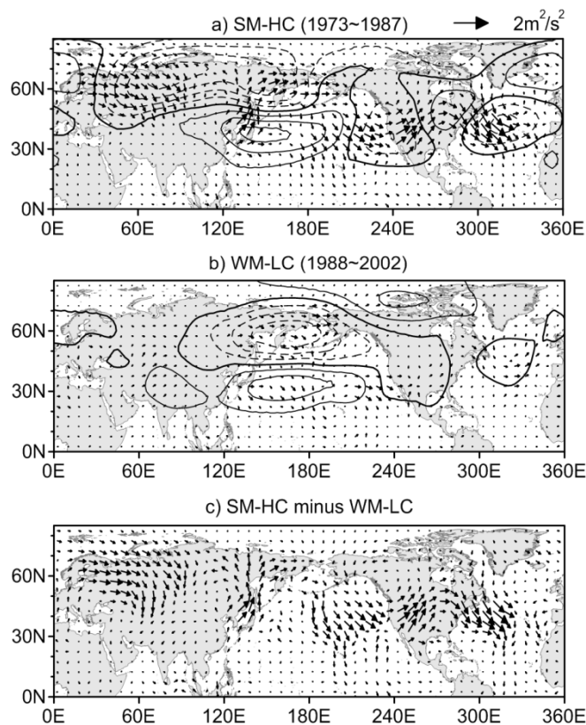
Figure 3.21. Stationary wave activity flux (in m^2 s^{-2} ; scale is given in the top-right corner) superimposed on the anomalous winter Z500 field regressed on the WP index for the (a) SM-HC and (b) WM-LC periods. (c) Difference in wave activity flux between the two periods.
