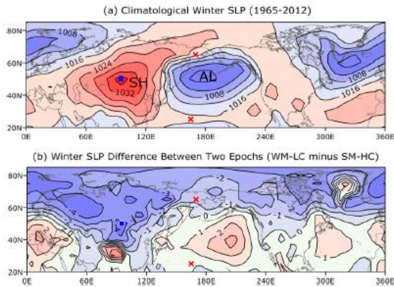
FIG. 3. (a) Climatological winter-mean SLP (in hPa) in the Northern Hemisphere north of 20°N during 1965–2012. The SH center (blue square) and the two centers of the NPO (red crosses) are indicated. (b) Winter SLP difference between two contrasting epochs: WM-LC (1988–2002) minus SM-HC (1973–87).
