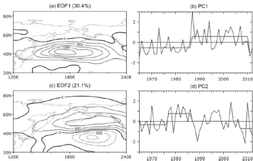
FIG. 8. Storm-track EOF and corresponding PC for the (a),(b) first mode and (c),(d) second mode. Contour interval is 300\text{m}^2 and negative values are dotted in (a),(c). Regime shift determination is shown by thick lines in (b),(d).
