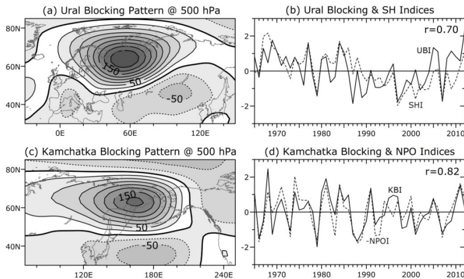
Figure 3.20. Blocking pattern \Delta Z_b (in m) over the projection area for (a) the Ural blocking and (c) the Kamchatka blocking. Comparison between (b) the Ural blocking index (UBI, solid) and SH index (SHI, dotted) and (d) the Kamchatka blocking index (KBI, solid) and negative NPO index (NPOI, dotted).
