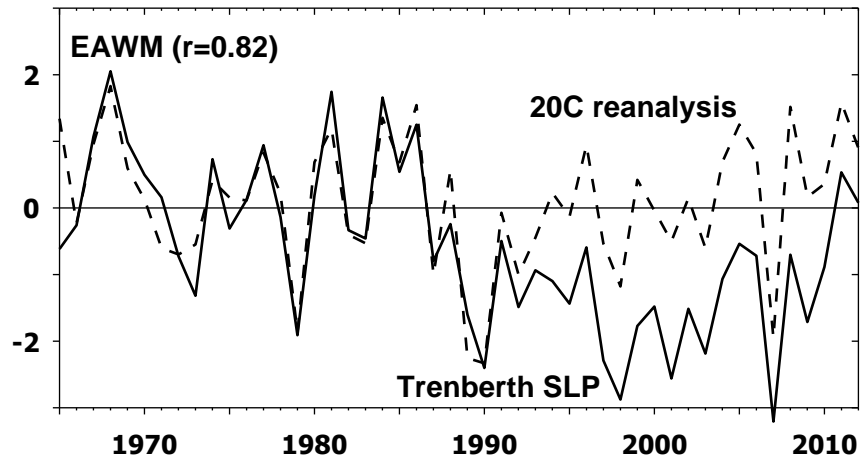
Figure 2.2. Comparison of EAWM indices obtained from Trenberth SLP (solid line) and 20C reanalysis (dotted line).
