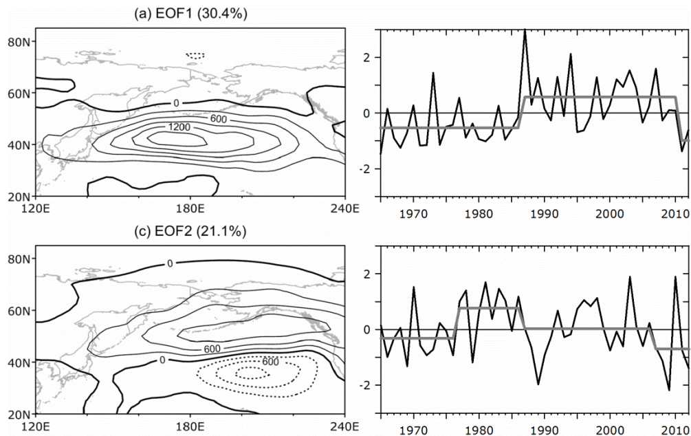
Figure 3.16. Storm track EOF and corresponding PC for the (a-b) first mode and (c-d) second mode. Contour interval is 300 m 2 and negative values are dotted in (a) and (c). Regime shift determination is shown by thick lines in (b) and (d).
