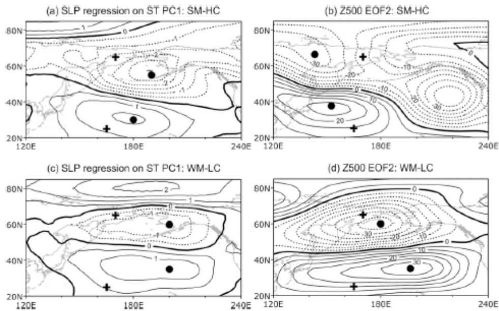
FIG. 9. Regression maps of anomalous winter SLP on the storm-track PC1 for the (a) SM–HC and (c) WM–LC periods. EOF2 of anomalous winter Z500 for the (b) SM–HC and (d) WM–LC periods. Contour intervals are 0.5 hPa for (a),(c) and 5 m for (b),(d). Crosses represent the two centers of action of NPO according to Wallace and Gutzler (1981), whereas black circles are those from the mapped patterns.
