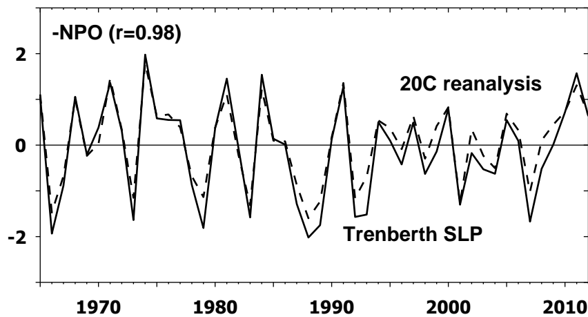
Figure 2.4. Comparison of NPO indices obtained from Trenberth SLP (solid line) and 20C reanalysis (dotted line).
