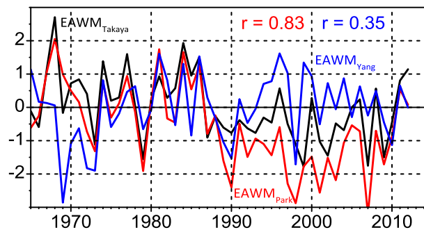
Figure 2.1. Comparison of EAWM_{Park} (red) and EAWM_{Yang} (blue) in reference to EAWM_{Takaya} (black), with corresponding correlation coefficients given ( EAWM_{Park}:EAWM_{Takaya} = 0.83 ; EAWM_{Yang}:EAWM_{Takaya} = 0.35 ).
