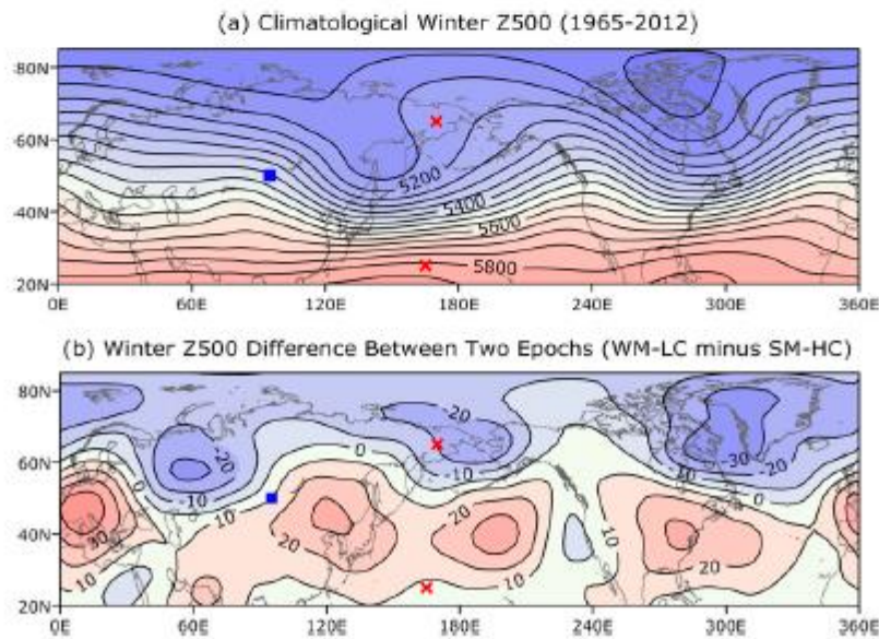
FIG. 4. (a) Climatological winter-mean Z500 (in m) in the Northern Hemisphere north of 20°N during 1965–2012. (b) Winter Z500 difference between two contrasting epochs: WM-LC (1988–2002) minus SM-HC (1973–87).
