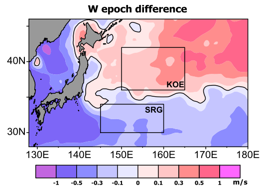
Figure 4.24. Spatial distribution of the composite difference (weak monsoon: 1997, 1990, 2001, 1998, 2007 minus strong monsoon: 1981, 1984, 1986, 1985, 2011) of wind speed obtained from 0.25^\circ \times 0.25^\circ gridded values.
