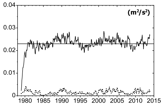
Figure 2.5. Temporal evolution of volume-averaged kinetic energy (unit is \text{m}^2 \text{s}^{-2} ) over the upper 400 m in the western North Pacific ( 140^\circ\text{--}180^\circ\text{E} , 28^\circ\text{--}46^\circ\text{N} , solid line) obtained from monthly averaged horizontal velocities. Kinetic energy obtained from volume-averaged velocity over the upper 400 m in the KOE region ( 150^\circ\text{--}165^\circ\text{E} , 36^\circ\text{--}42^\circ\text{N} , dotted) is also overlaid and a solid line indicating constant value of 0.023 \text{ m}^2 \text{ s}^{-2} is superimposed.
