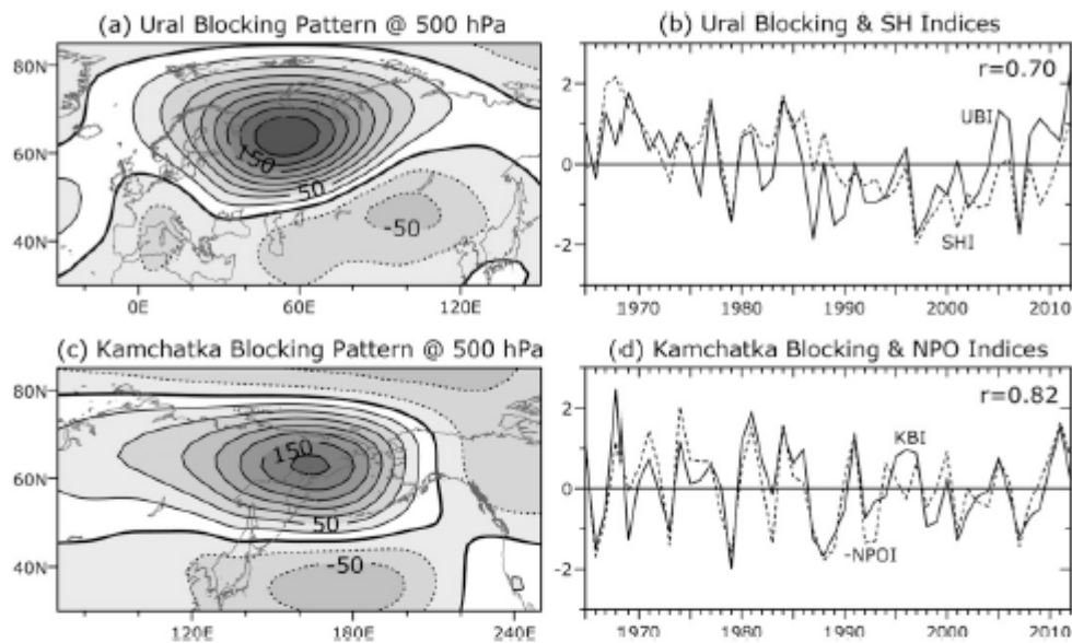
FIG. 6. Blocking pattern \Delta Z_s (in m) over the projection area for (a) the Ural blocking and (c) the Kamchatka blocking. Comparison between (b) the Ural blocking index (UBI; solid) and SH index (SHI; dotted) and (d) the Kamchatka blocking index (KBI; solid) and negative NPO index (NPOI; dotted).
