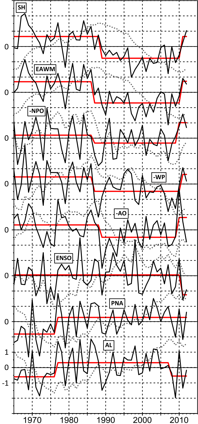
Figure 3.3. Climate regime shift determination (red) from normalized climate indices (black) based on Rodionov (2004), together with normalized cumulative sums (dotted gray).
