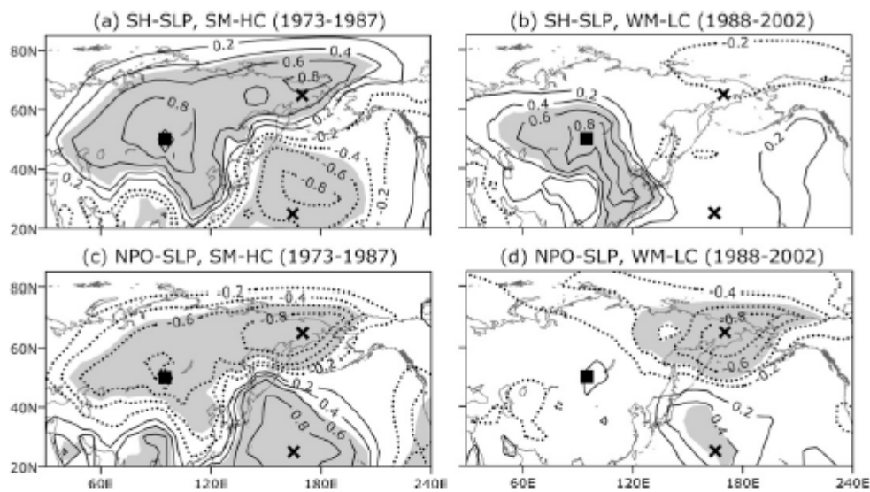
FIG. 5. (a),(b) Correlation maps of SLP anomalies with the SH index for the SM–HC epoch (1973–87) and the WM–LC epoch (1988–2002), respectively. (c),(d) As in (a),(b), but for the NPO index. The areas with significant correlations at the 95% confidence level are shaded.
