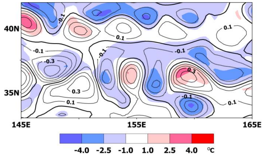
Figure 4.2. T400a (color, anomaly subtracting total period mean) and SSHA (contour, high pass filtered one using 6^{\circ} \times 4^{\circ} filter) for winter (DJF) 1984. Showing warm/cold eddy contribution to the temperature anomaly.
