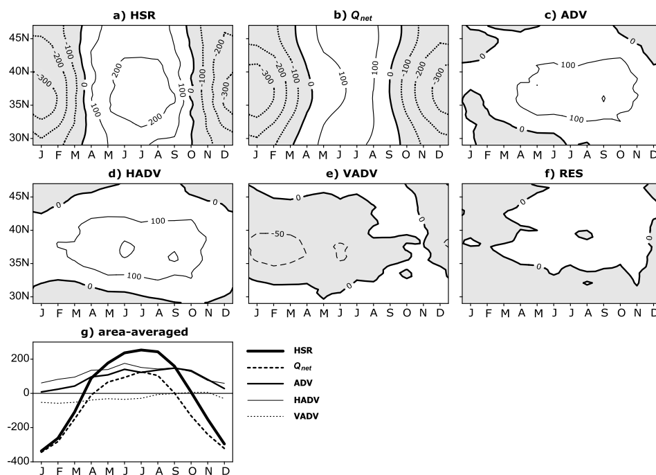
Figure 4.8. Zonal mean ( 150^{\circ} - 165^{\circ} E) seasonal climatologies of (a) heat storage rate (HSR), (b) net heat surface flux ( Q_{net} ), (c) total heat advection (ADV), (d) horizontal heat advection (HADV), (e) vertical heat advection (VADV), and (f) residual (RES) over the western North Pacific between 28^{\circ} N and 46^{\circ} N. Model outputs have previously been spatially smoothed with a 6^{\circ} \times 4^{\circ} window. Contour interval is 100 \text{ W m}^{-2} and supplementary contour of -50 \text{ W m}^{-2} is added in (e). Negative values are shaded. (g) Spatially-averaged monthly climatologies of heat budget components (in \text{W m}^{-2} ) in the KOE region ( 150^{\circ} - 165^{\circ} E, 36^{\circ} - 42^{\circ} N).
