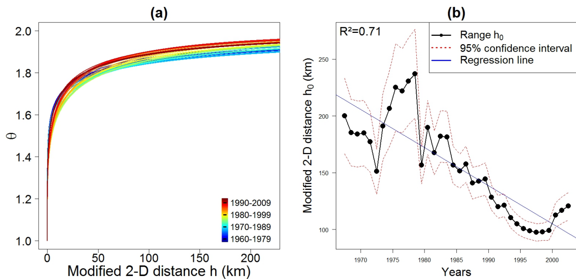
Figure 3.7: (a) Temporal evolution of the fitted Brown-Resnick extremal functions under the 2-D modified distance, from oldest time windows (blue curves) to the most recent ones (red curves). (b) Temporal evolution of the range of extremal dependence. The range (equation (3.15)) is expressed as a function of the 2-D modified distance (equation (3.11)). It is plotted (black dots) as a function of the center of the considered estimation window. The associated 95% confidence interval is evaluated by the delta method using equation (3.18). The linear fit (straight blue regression line) is made on the winter estimates (black dots).
