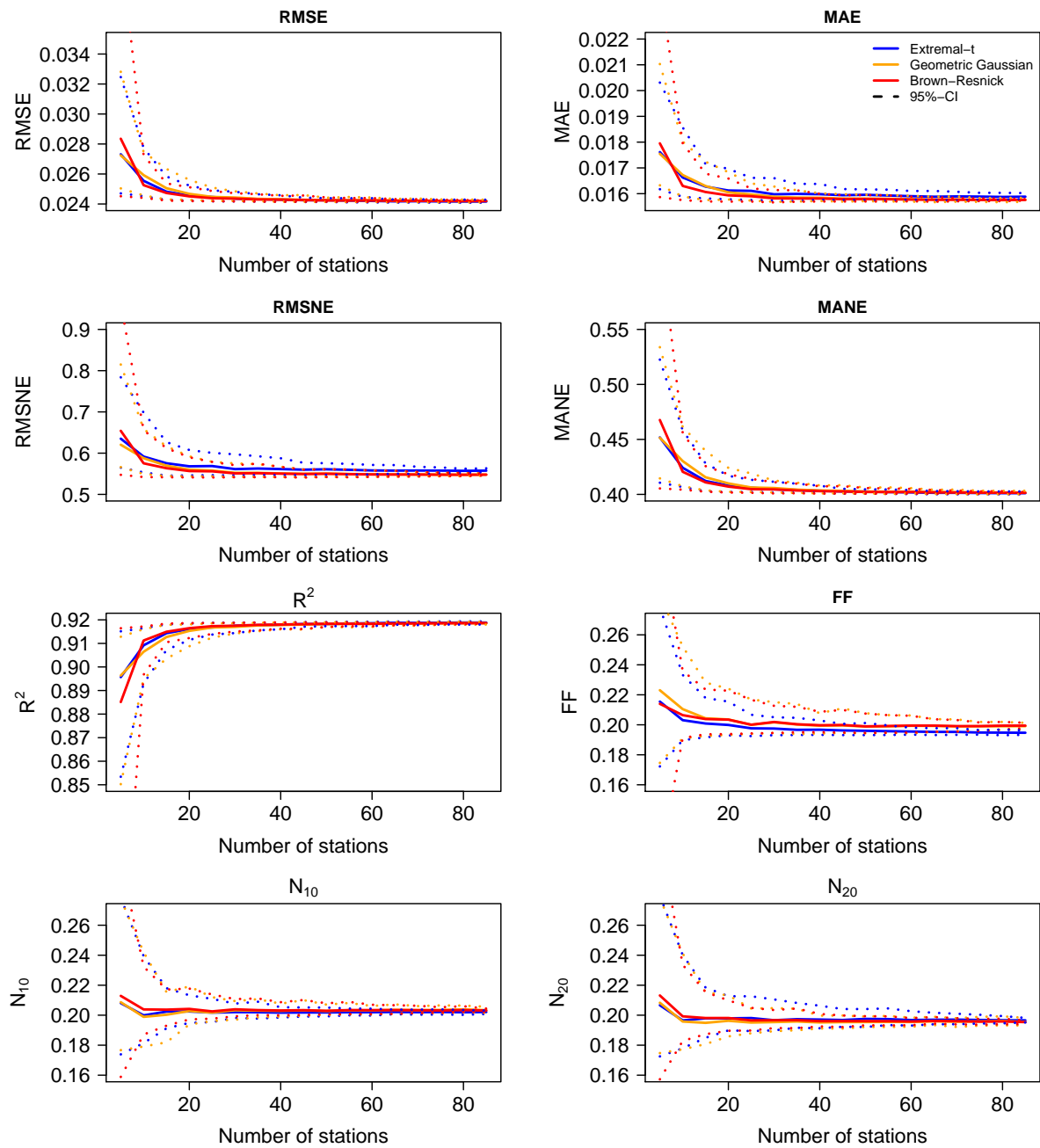
Figure 2.3: RMSE , MAE , R^2 , RMSNE , MANE , N_{10} , N_{20} and FF criteria according to the number of stations, each of them having 55 years of observations. Plain lines represent means. The dotted lines represent the empirical 95%-confidence interval.
