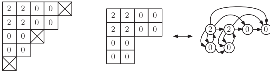
FIGURE 5.14. How to obtain a valued digraph associated with \mathcal{T}_3^{(2)} . The (non-simple) valued digraph on the right also gives a lattice isomorphic to \mathcal{T}_3^{(2)} .
