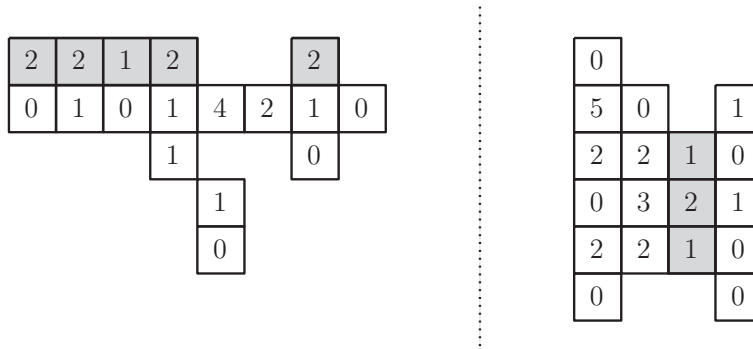
FIGURE 6.7. A dominant row (on the left) and a dominant column (on the right).
