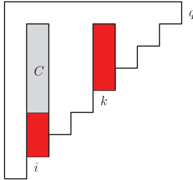
FIGURE 5.10. An element A in IS(\mathcal{A}_n^\uparrow) is depicted in red, while an admissible column above A is in grey.
