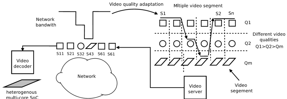
Figure 23. Adaptive streaming
