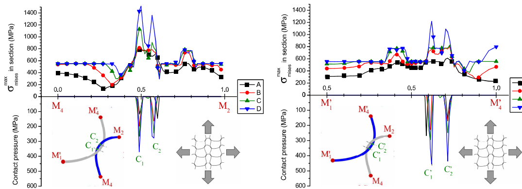
Figure V.43. Maximum mises stress (top) and contact pressure (bottom) in the wire section along normalized curvilinear abscissa between points M_4 and M_2 (left) and points M_1' and M_4' (right) using superelastic material during biaxial tension at strains increments A, B, C, and D.
