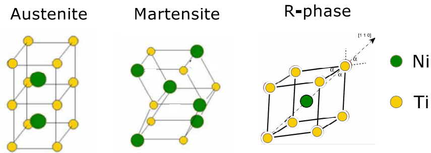
Figure II.1. Crystal structure of austenite, martensite, and R-phase for NiTi SMA.
