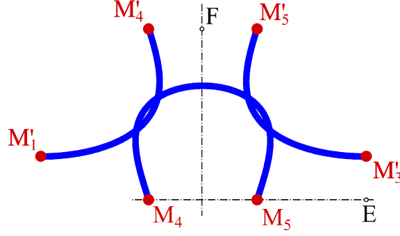
Figure IV.10. Knit loop model presenting boundary points and master nodes E and F.
