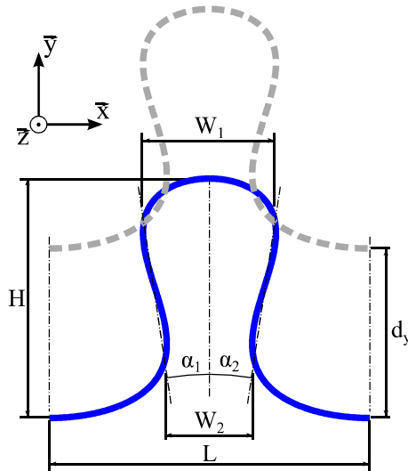
Figure V.4. Knit loop dimensional parameters.
