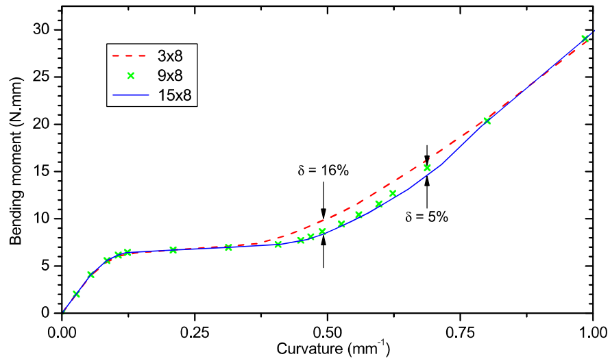
Figure IV.7. Bending moment versus curvature using 3x8 (red dash), 9x8 (green crosses), and 15x8 (blue line) integration points along \vec{e}_r and \vec{e}_\theta respectively.
