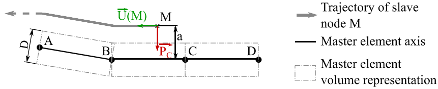
Figure IV.12. Illustration of contact management between beam finite elements using explicit resolution method.
