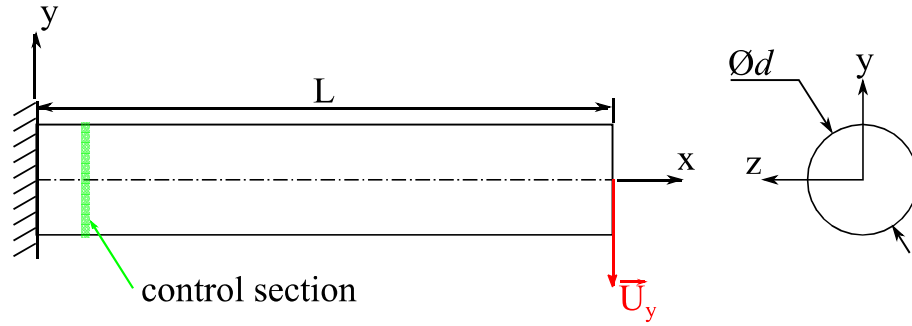
Figure IV.5. Beam bending benchmark performed to compare beam finite elements and standard 3D brick elements.
