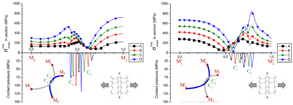
Figure V.36. Maximum mises stress (top) and contact pressure (bottom) in the wire section along normalized curvilinear abscissa between points M_4 and M_2 (left) and points M_1' and M_4' (right) using linear elastic material during uniaxial course-wise tension at strains increments A, B, C, and D.
