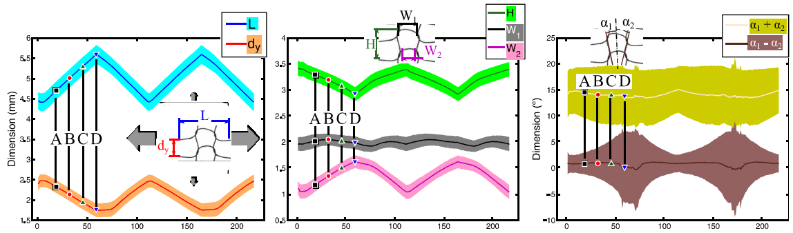
Figure V.13. Loop dimensions variations during loading cycles in course-wise tension
