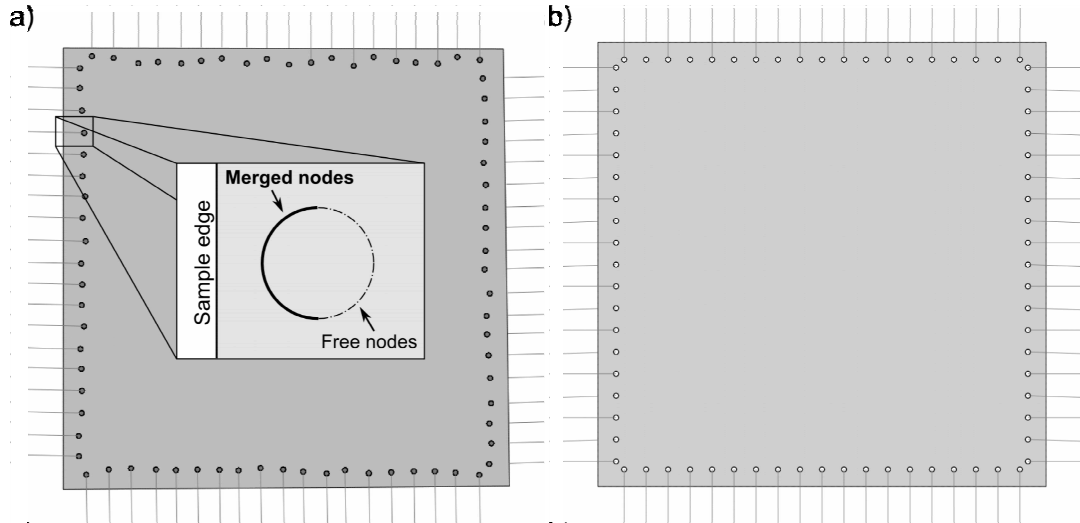
Figure III.21. Geometry of finite elements models with a) experimental hooks disposition and b) ideal hooks disposition.
