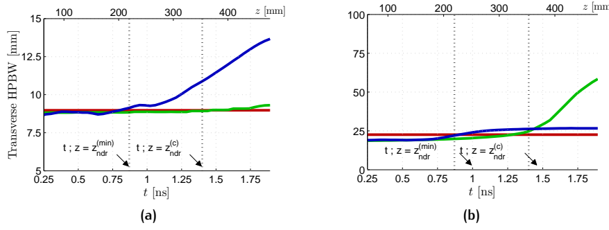
Figure 6.11.: Evolution of the (a) transverse and (b) longitudinal HPBW vs. t . The ideal (red curves), dispersive (green curves), and the dispersive-finite case (blue curves) are represented for \Delta\omega = 0.2 . The x -axis on the top is obtained by scaling the temporal axis with the theoretical group velocity v_z \simeq 0.84c_0 .
