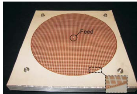
Figure 5.7.: Final prototype. The array of vias comprising the outer metallic rim is shown in the inset. Courtesy of Mauro Ettorre [234].
