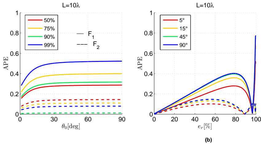
Figure 2.10.: (a) APE (calculated as 100 \cdot |eF_1BW - eBW| / |eBW| ) vs. \theta_0 for \epsilon_r = 50\%, 75\%, 90\%, 99\% (in order in red, yellow, green, blue) and (b) APE vs. \epsilon_r for \theta_0 = 5^\circ, 15^\circ, 45^\circ, 90^\circ (in order in red, yellow, green, blue). The e F_1 BW is calculated using either the F_1 (solid lines) or the F_2 (dashed lines) formulas. Results are shown only for L = 10\lambda .
