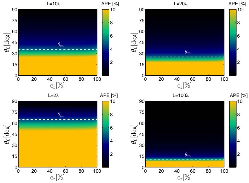
Figure 2.9.: APE (calculated as 100 \cdot |\text{aBW} - \text{eBW}| / |\text{eBW}| ) vs. \theta_0 and e_r . White dashed lines highlight the boundaries set by \theta_m .
