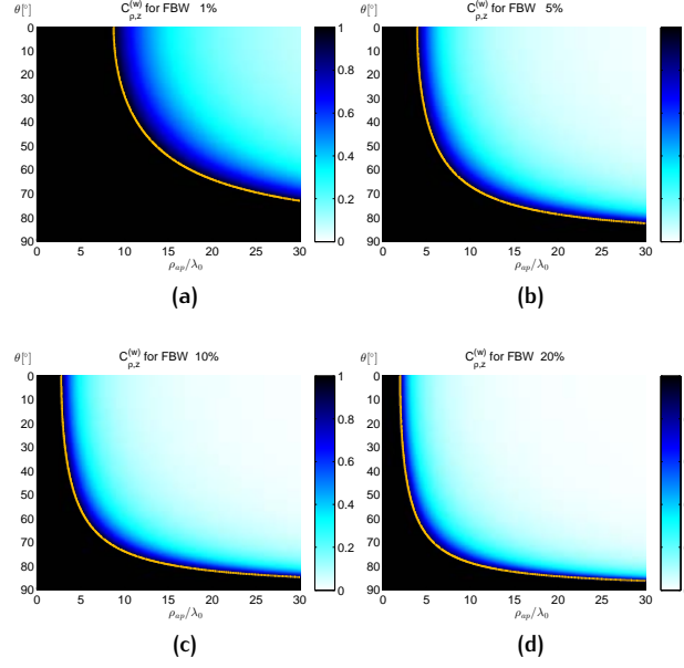
Figure 6.3.: Weak confinement C_{\rho,z}^{(w)} vs. \rho_{ap}/\lambda_0 and \theta . The yellow hyperbola represents the boundary between the region of efficient (in white) and non-efficient confinement (in black) for ideal UXWs, when fractional bandwidths of (a) \overline{\Delta\omega} = 0.01 , (b) \overline{\Delta\omega} = 0.05 , (c) \overline{\Delta\omega} = 0.1 , and (d) \overline{\Delta\omega} = 0.2 are considered. The region of efficient confinement increases for larger fractional bandwidths. In any case, this region corresponds to electrically large apertures with small axicon angles.
