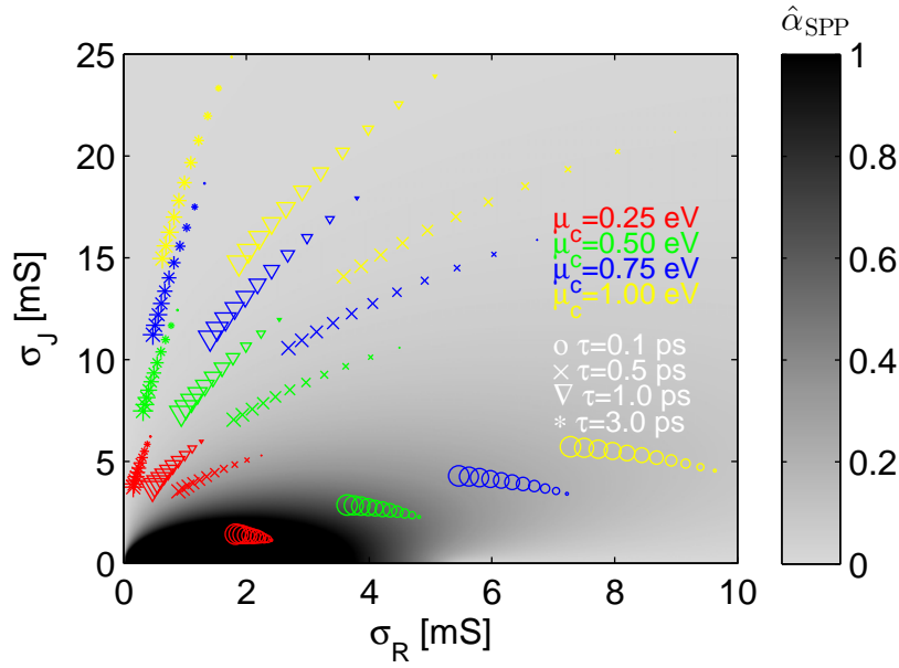
Figure 3.7.: Intensity of plasmonic dissipation losses \hat{\alpha}_{SPP} in the range [0,1] in the \sigma complex plane. The dynamic range of \hat{\alpha}_{SPP} has been saturated to values greater than 1 for readability purposes. The paths followed by the graphene surface conductivity in the complex plane have been reported for values of f ranging from 0.75 THz to 1.25 THz (size of the symbols increases), \tau ranging from 0.1 ps to 3 ps (symbols change shape in the following order: \circ, \times, \nabla, * ) and \mu_c ranging from 0.25 eV to 1 eV (color of the symbol change in the following order: red, green, blue, and yellow). The black region represents the area characterized by the highest dissipation losses and is attained by graphene samples with both lower \mu_c and \tau .
