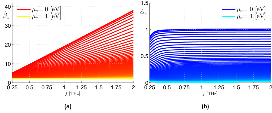
Figure 3.14.: Dispersion curves of (a) \hat{\beta}_z , (b) \hat{\alpha}_z for the plasmonic mode SPP. Lines become brighter (red to yellow, and blue to cyan) as \mu_c increases from 0 to 1 eV. Note that as \mu_c approaches 1 eV the SPP mode approaches the PPW TEM mode.
