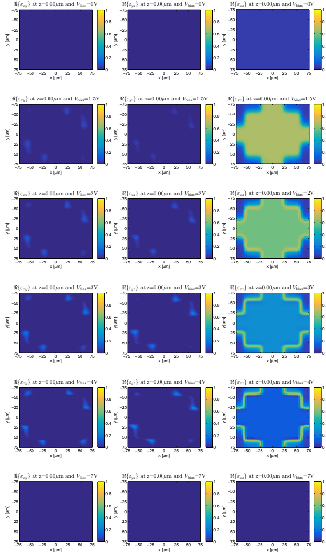
Figure 3.33: Real part of the off-diagonal terms \varepsilon_{ij}(x, y, z = 0) vs. xy -plane of the relative permittivity tensor for V_{\text{bias}} = 0 - 7 [V]. First column ( i = x, j = y ), second column ( i = y, j = z ), and third column ( i = x, j = z ). Starting from the first row the driving voltage takes the following values: \{0, 1.5, 2, 3, 4, 7\} [V].
