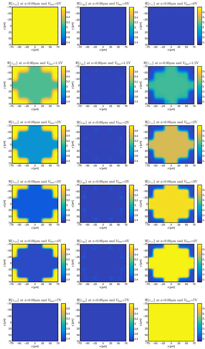
Figure 3.32.: Real part of the diagonal terms \varepsilon_{ii}(x, y, z = 0) vs. xy -plane of the relative permittivity tensor for V_{\text{bias}} = 0 - 7 [V]. First column ( i = x ), second column ( i = y ), and third column ( i = z ). Starting from the first row the driving voltage takes the following values: \{0, 1.5, 2, 3, 4, 7\} [V].
