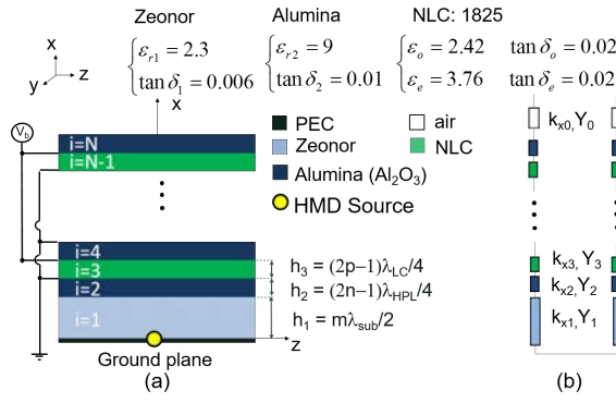
Figure 3.36.: 2-D section view of the proposed device and its equivalent transmission-line representation. The NLC layers are biased through a pair of extremely-thin moderately-conductive polymer films (not reported in the picture), e.g., PEDOT:PSS [99], whose absorption is neglected here.
