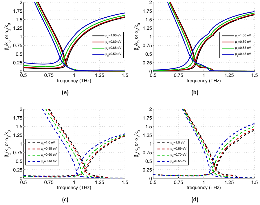
Figure 3.28.: Dispersion diagrams of \hat{\beta}_z and \hat{\alpha}_z vs. f for (a)-(c) TE and (b)-(d) TM fundamental leaky modes of a (a)-(b) graphene-based planar single-slab antenna (solid lines) and a (c)-(d) graphene-strip grating antenna (dashed lines). The values of the chemical potentials \mu_c are reported in the legends.
