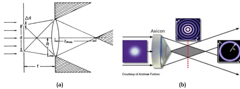
Figure 4.5.: (a) A sketch of the experimental setup used by J. Durnin for the first generation of a Bessel beam in optics [188]. (b) A sketch of the experimental setup for generation of a Bessel beam through an axicon lens as presented in [222]. The axicon element allows for converting a Gaussian beam into a Bessel beam within a rhomboidal region located in the near field. The dashed red line is located at z = z_{\text{ndr}}/2 . In the far-field, the Fourier-Transform of the aperture field gives rise to the expected annulus shape.
