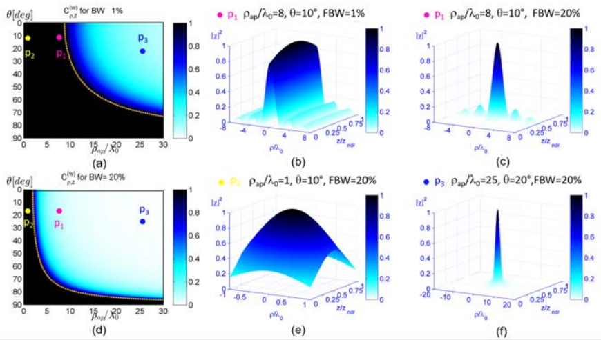
Figure 6.5.: C_{\rho,z}^{(w)} vs. \rho_{ap}/\lambda_0 and \theta_0 for (a) FBW = 1% and (d) FBW = 20%. The purple dot p_1 represents an X-wave with m = 8 and \theta = 10^\circ . The yellow dot p_2 represents an X-wave with m = 1 and \theta = 10^\circ . The blue dot p_3 represents an X-wave with m = 25 and \theta = 20^\circ . An X-wave in p_1 is generated for (b) FBW = 1% and (c) FBW = 20%, whereas X-waves in (e) p_2 and (f) p_3 are both generated for FBW = 20%. In (b-c) and (e-f), the intensity of the X-wave is reported over a \rho z plane limited by \rho_{ap} along \rho and z_{ndr} along z . From this representation, if S_\rho and S_z fit in the plot, then the X-wave is confined over the respective axis. Note that, the \rho -axis is normalized to \rho_{ap} while the z -axis is normalized to z_{ndr} .
