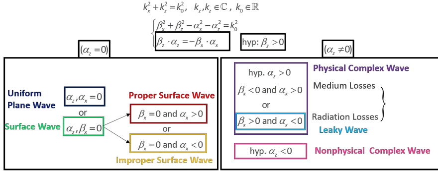
Figure 1.3.: Classification of forward waves in open regions with respect to their propagating features. When \alpha_z = 0 two kinds of waves exist: uniform plane waves \alpha_x = 0 , and surface waves \alpha_x \neq 0 . Surface waves might be proper or improper, depending on the sign of \alpha_x . When \alpha_z \neq 0 , physical leaky waves exist only when \alpha_z > 0 . Even more interestingly, in order to describe a radiation mechanism \beta_x > 0 , a forward leaky wave must be improper.
