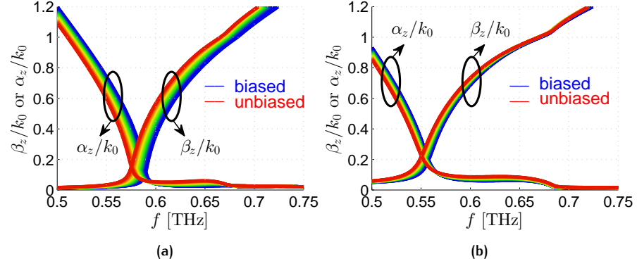
Figure 3.39: Dispersion curves ( \hat{\beta}_z and \hat{\alpha}_z vs. f ) of the fundamental TM leaky mode for (a) Layout 2 and (b) Layout 4 (see Table 3.5) in the lossy case, when the NLC layer is biased at V_\infty (blue lines) and when is unbiased 0 V (red lines). Colors gradually shades from blue to red as V_b decreases from V_\infty to 0 V.
