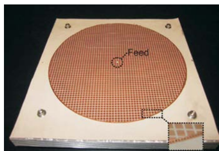
Figure 5.7.: Final prototype. The array of vias comprising the outer metallic rim is shown in the inset. Courtesy of Mauro Ettore [234].
