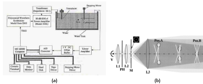
Figure 4.7.: (a) A sketch of the experimental setup used by Lu and Greenleaf for the first generation of X-waves in acoustics [263]. (b) A sketch of the experimental setup for the first measurement of the 3-D field distribution of X-waves in optics [264]. Except for a system of converging lenses and a pinhole, the mechanism of generation was equal to the one originally proposed by Durnin [188] for the Bessel beam generation.
