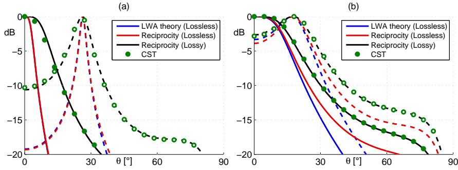
Figure 3.40.: Radiation patterns for (a) Layout 2 and (b) Layout 4 for radiation at broadside (solid) and at the maximum pointing angle (dashed). The radiation patterns have been calculated by means of reciprocity theorem in both the lossless (in red) and the lossy (in black) case, and then compared with those given by means of LWA theory (blue). Full-wave simulations with CST are also reported for the lossy case for radiation at broadside (filled green circles) and at the maximum pointing angle (empty green circles).
