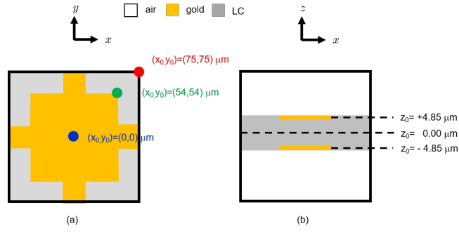
Figure 3.31.: 2-D section (a) on the xy -plane and (b) on the xz -plane of the THz fishnet MM. Further details on the unit-cell are available in [96].
