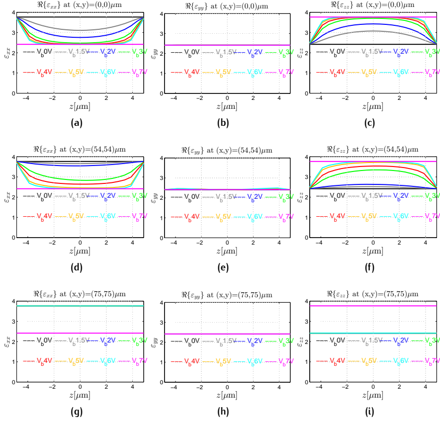
Figure 3.34.: Real part of the diagonal terms \epsilon_{ii}(x = x_0, y = y_0, z) vs. z for V_{\text{bias}} = 0 - 7 [V]. First column ( i = x ), second column ( i = y ), and third column ( i = z ). Starting from the first row the (x_0, y_0) position takes the following values: (0, 0) \mu\text{m} , (54, 54) \mu\text{m} , and (75, 75) \mu\text{m} .
