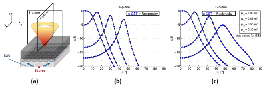
Figure 3.23: (a) Illustrative example of the typical conical beam-scanning feature of a GSS antenna. In (b) and (c), the radiation patterns normalized to the overall maximum (achieved at broadside) vs. elevation angle \theta for the GSS antenna represented in (a), are reported for the H-plane and E-plane, respectively. Analytical results are plotted in black solid lines, whereas full-wave results obtained with the tool CST Microwave Studio [159] are given by blue circles. The scanning behavior at a fixed frequency ( f_c = 1.132 THz) is shown for beam maxima at \theta = 0^\circ, 15^\circ, 30^\circ, 45^\circ . The corresponding chemical potentials are reported in the legend.
