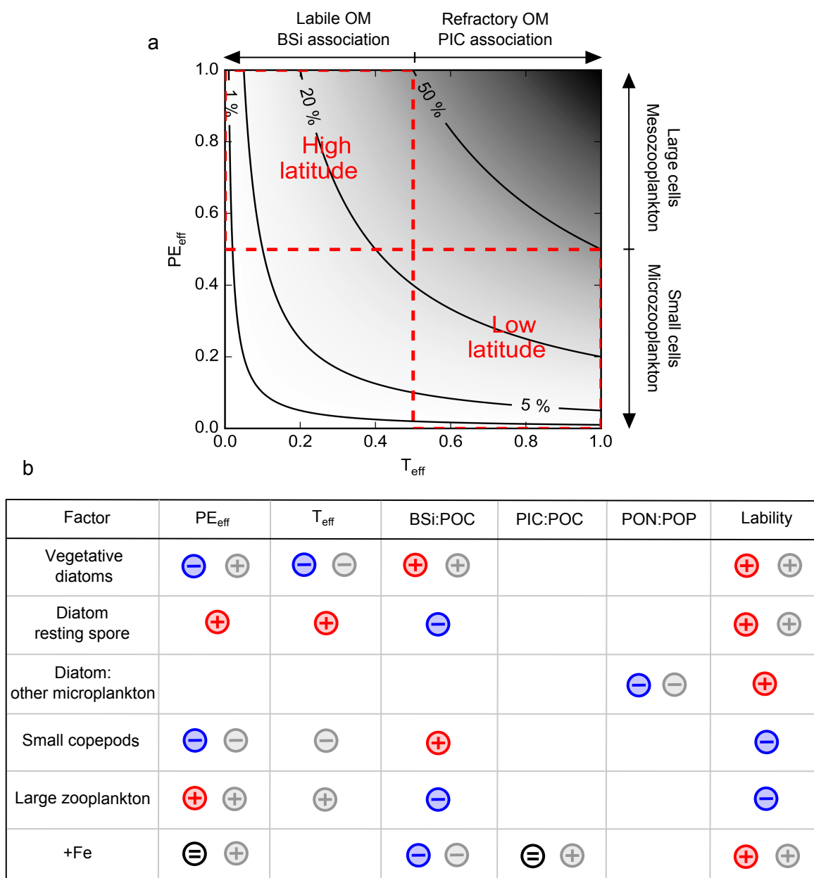
Figure 5.2: a. Summary of the relationship between ecosystem structure and the functioning of the biological pump from the literature. Isolines and grey scale represent the biological pump efficiency (fraction of net primary production exported). b. Table synthesizing the main results obtained during the PhD (coloured symbols). Positive relationships shown in red, negative in blue, no effect in black. Grey symbols represent the relationships suggested by the literature.
