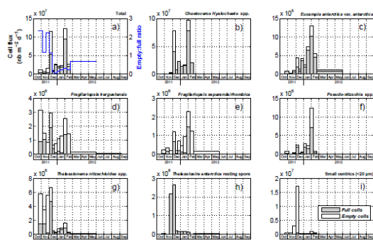
a) total full and empty cell fluxes. Blue line denotes the total empty:full cell ratio. b) to i) fluxes of major diatom species (> 1% of the total cell flux).
