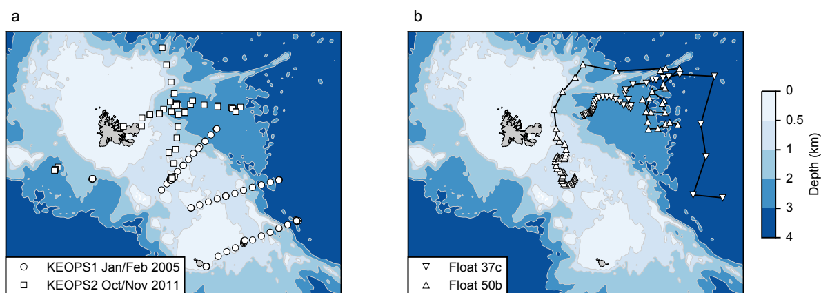
Figure A.4: a. Location of the KEOPS1 (January/February 2005) and KEOPS2 (October/November 2011) CTD profiles. b. Location of the profiles from two bio-argo floats deployed from January to May 2015. Colors correspond to bathymetry.
