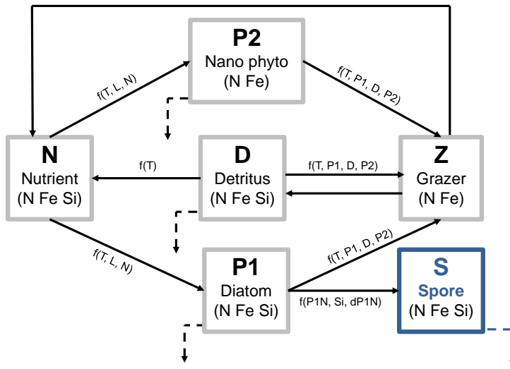
Figure A.8: Scheme of a simple NPZD model used to test formulations of resting spore formation. Continuous arrows represent the flux of matter and dashed arrows represent the sinking of components.
