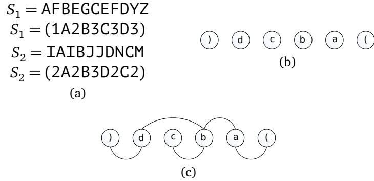
Figure 3.11: Input sequences S_1 and S_2 in (a) are parsed into nodes in (b) and then used to build Hasse diagram in (c).
