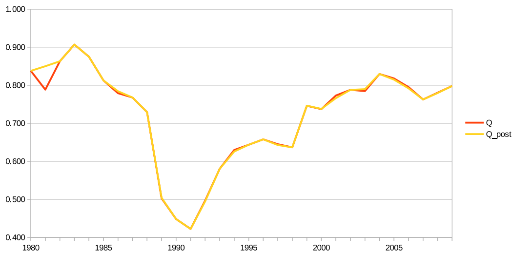
FIGURE 3.5: Modularity evolution, pre- and post-filtering.
