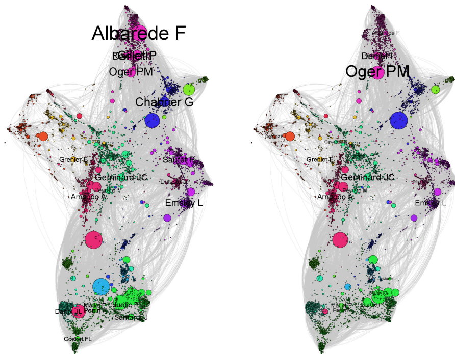
FIGURE 1.5: Co-citation and co-author network of articles published by scientists at ENS de Lyon. Nodes represent the authors of references appearing in the articles, while links represent co-appearances of these features in the same article. The color of the nodes corresponds to the modularity partition and their size is proportional to their BC (left) or to their bridge-gness (right), which clearly leads to different rankings (references cited are used in the computations of the centrality measures but appear as dots to simplify the picture). We only keep nodes - authors - that appear on at least four articles and links that correspond to at least 2 co-appearances in the same paper. After applying these thresholds, the 8,000 articles lead to 8,883 nodes (author or references cited in the articles) and 347,644 links. The average degree is 78, the density 0.009 and the average clustering coefficient is 0.633. Special care was paid to avoid artifacts due to homonyms. Weights are attributed to the links depending on the frequency of co-appearances (as cosine distance, see Grauwijn and Jensen, 2011).
