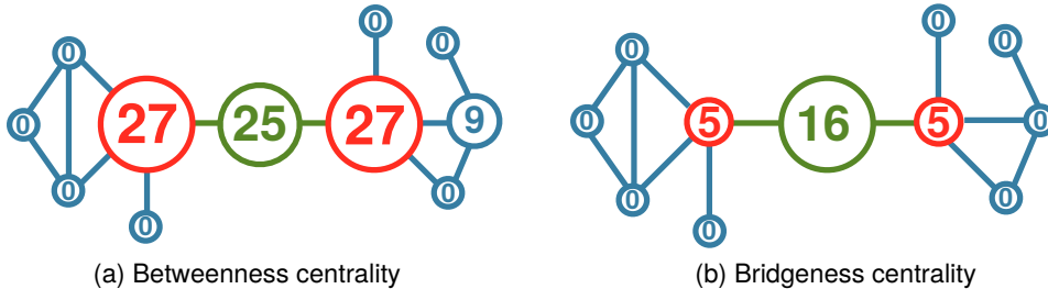
FIGURE 1.1: The figures show the betweenness (a) and bridgeness (b) scores for a simple graph. Betweenness does not distinguish centers from bridges, as it attributes a slightly higher score (Figure a, scores = 27) to high-degree nodes, which are local centers, than to the global bridge (Figure a, score = 25). In contrast, bridgeness rightly spots out the node (Figure b, score = 16) that plays the role of a global bridge.
