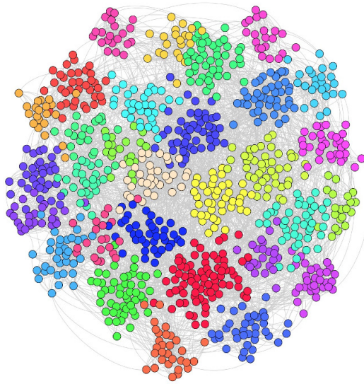
FIGURE 1.2: Artificial network with a clear community structure using Lancichinetti, Fortunato, and Radicchi (2008) method. For clarity, we show here a smaller network containing 1.000 nodes, 30 communities, 7.539 links (20% inter- and 80% intra-community links). Each color corresponds to a community as detected by modularity optimization (Newman, 2010; Blondel et al., 2008).
