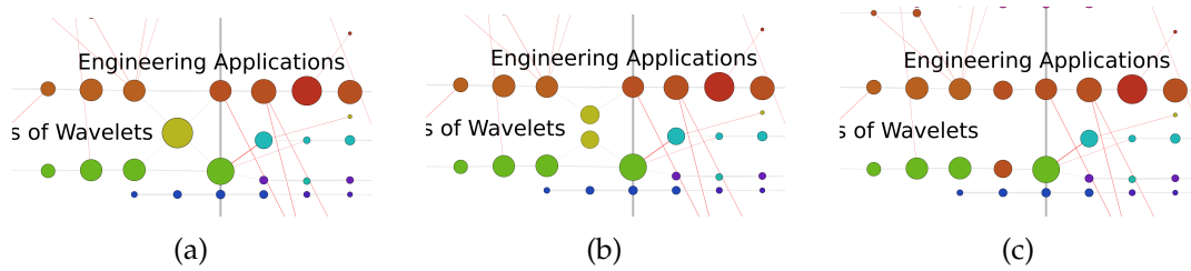
FIGURE 3.4: Detail of 1994 split. From left to right, the unduly merged communities are split and assigned to their respective streams.
