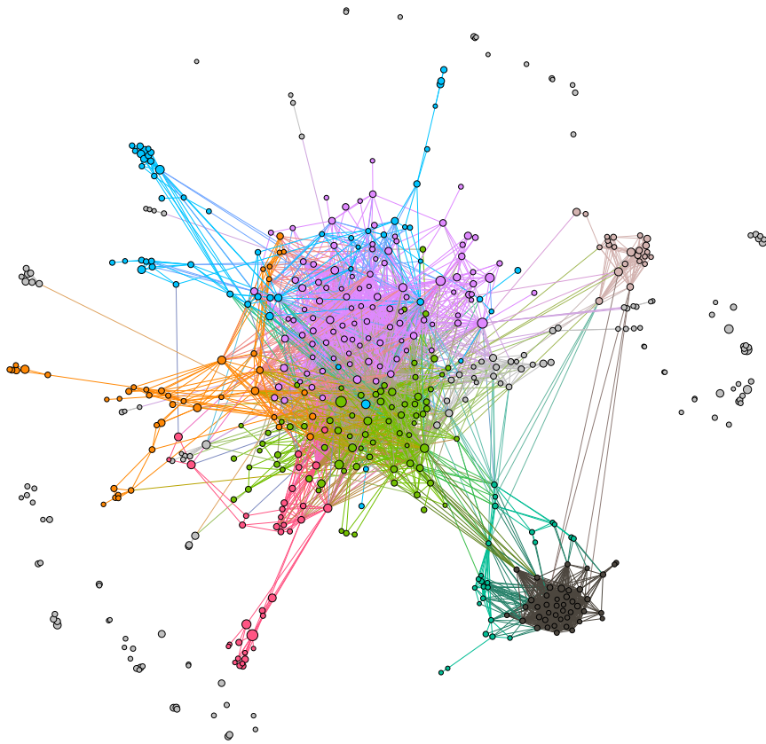
FIGURE S5: Full articles network, time window 1994–1997
