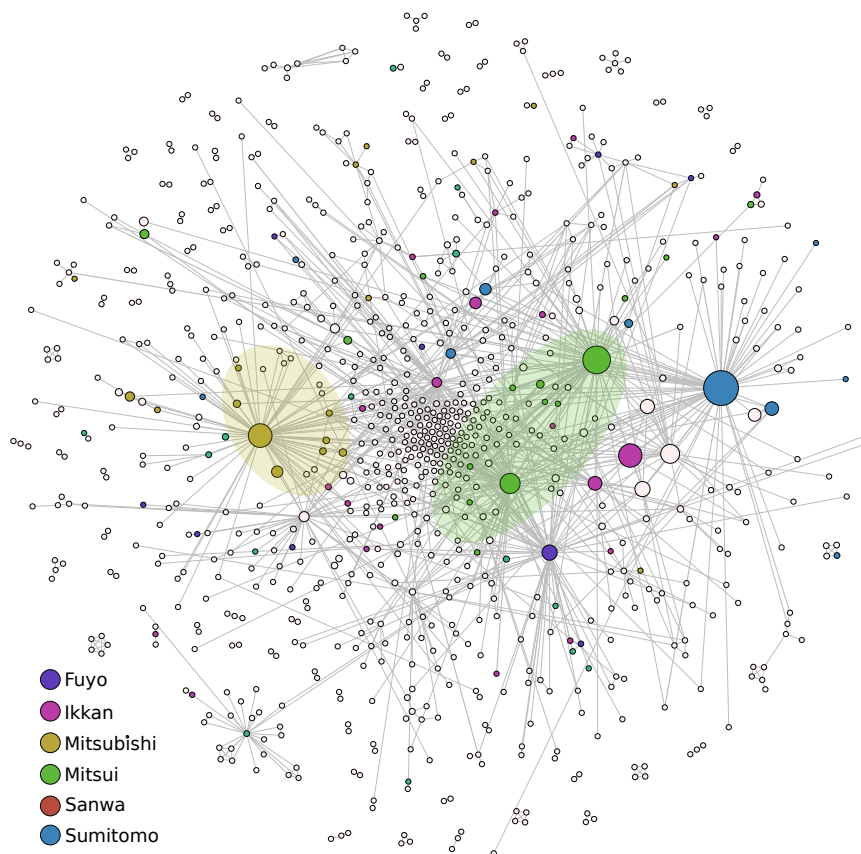
FIGURE 2.5: Worldwide Japanese investors network: business ties and Big-6 membership. Highlighted: Mitsubishi and Mitsui clusters
