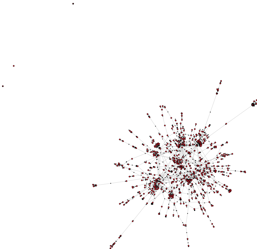
FIGURE 2.3: Heterogeneous network, including Japanese investors and overseas subsidiaries, ASEAN countries only
