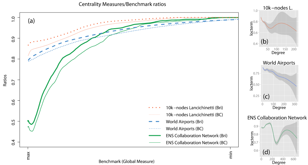
FIGURE 1.3: (a) Ability of BC or bridgeness to reproduce the ranking of bridging nodes, taking as reference the global indicator (Eq2). For each of the three networks, we first compute the cumulative sums for the global measure G , according to three sorting options: the G measure itself and the two centrality metrics, namely BC and bridgeness. By construction, sorting by G leads to the highest possible sum, since we rank the nodes starting by the highest G score and ending by the lowest. Then we test the ability of BC or bridgeness to reproduce the ranking of bridging nodes by computing the respective ratios of their cumulative sum, ranking by the respective metric (BC or Bri), to the cumulative obtained by the G ranking. A perfect match would therefore lead to a ratio equal to 1. Since we observe that the ratio for bridgeness is higher than for BC, this means that ordering nodes by their decreasing bridgeness leads to a better ranking of the 'global' scores as measured by G . To smooth the curves, we have averaged over 200 points. Curves corresponding to different networks are coloured as LFR (red), Airports (blue), ENS (green). (b, c, d): average relative local terms as function of node degree for the three investigated networks (for definition see text).
