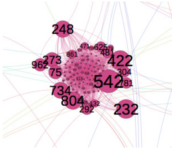
FIGURE S1: Zoom on cluster 5 of the synthetic network. The numbers represent labels, while the size of the nodes is proportional to their BC score.
