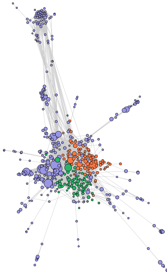
FIGURE S4: Year 1994: an ambiguous group of nodes, can be either split in two or merged in one single community, colored in green and orange; see also main text, section 3.5
