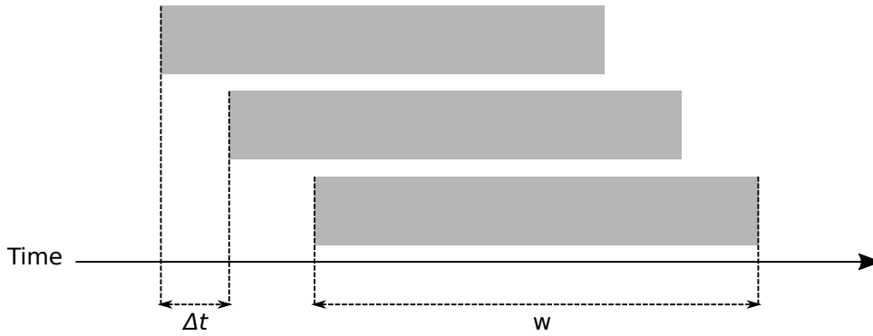
FIGURE 3.1: Sliding temporal windows
