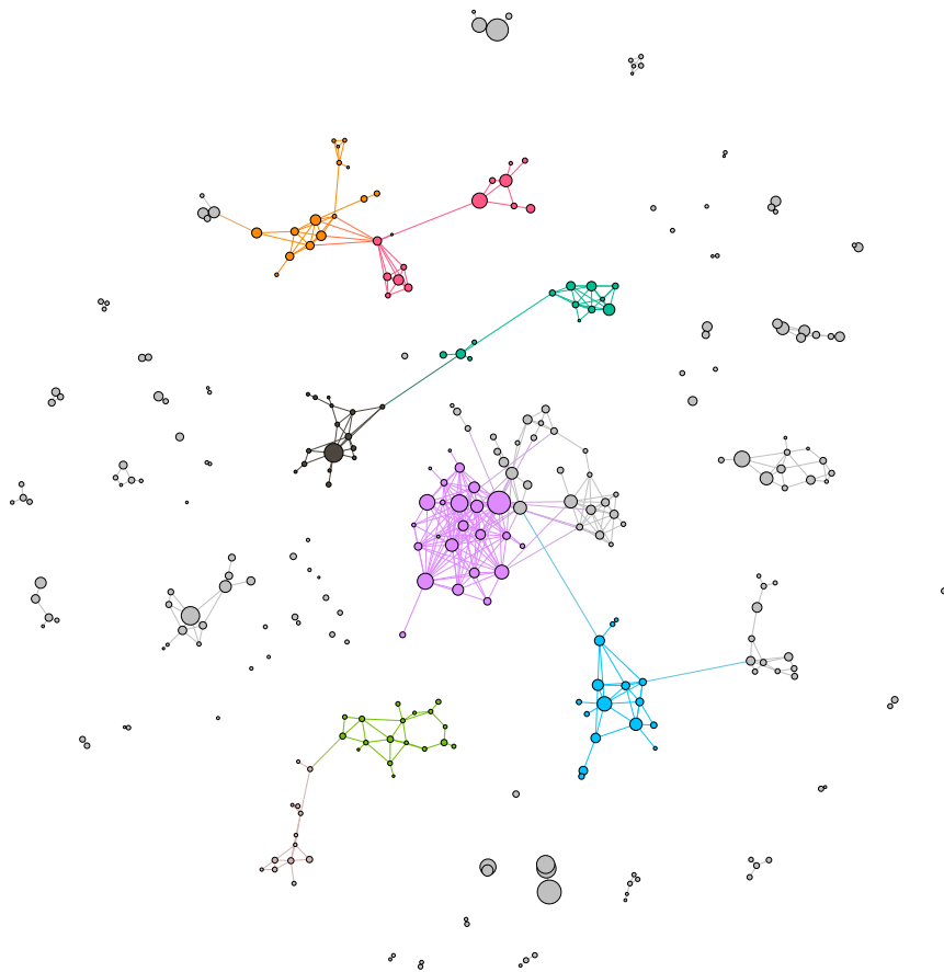
FIGURE S6: Full articles network, up to year 1982
