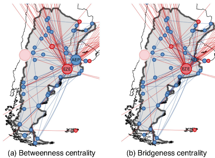
FIGURE 1.4: Example of the two largest Argentinean airports, Ezeiza (EZE) and Aeroparque (AEP). Both have a similar degree (54 and 45 respectively), but while the first connects Argentina to the rest of the world (85% of international connections, average distance 2,848 miles, G=2,327.2 ), Aeroparque is only a local center (18% of international connections, average distance 570 miles, G=9.0 ). However, as in the simple graph (Figure 1), BC gives the same score to both ( BC_{EZE}=79,000 and BC_{AEP} = 82,000 ), while bridgeness clearly distinguishes the local center and the bridge to the rest of the world, by attributing to the global bridge a score 250 times higher ( Bri_{EZE}=46,000 and Bri_{AEP} = 174 ). Red nodes represent international airports while blue nodes are domestic.
