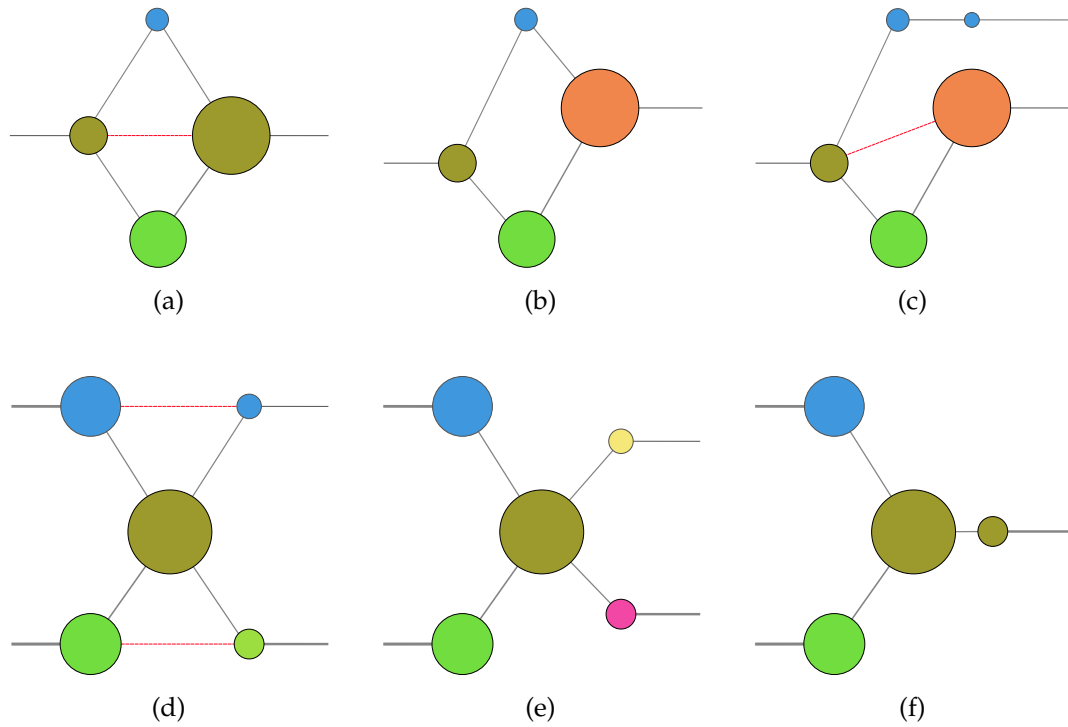
FIGURE 3.2: Ephemeral (artificial) versus structural (real) events
