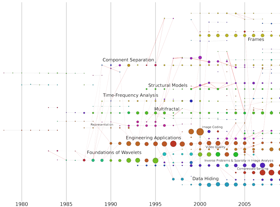
FIGURE 3.3: Overview of the history of wavelets
