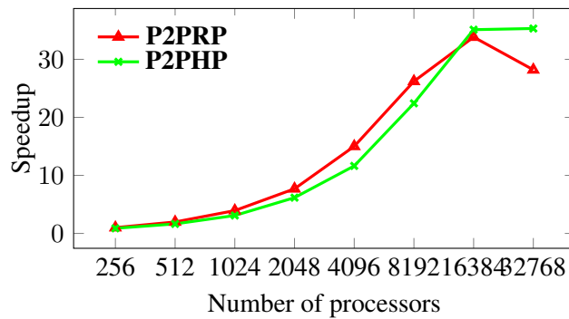
(c) Flickr matrix with k = 48 on Blue Gene/Q.
