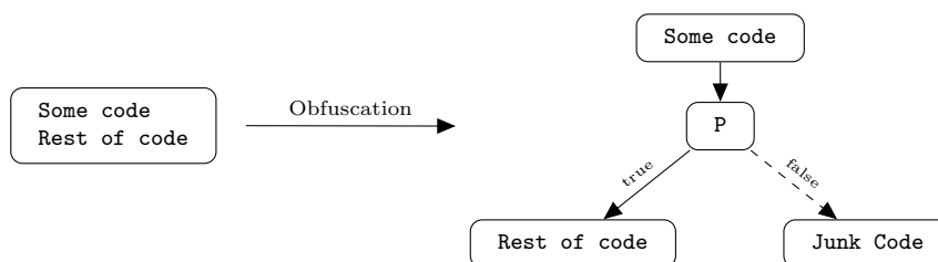
Figure 1.4: Classical opaque predicate construct with P always true.
