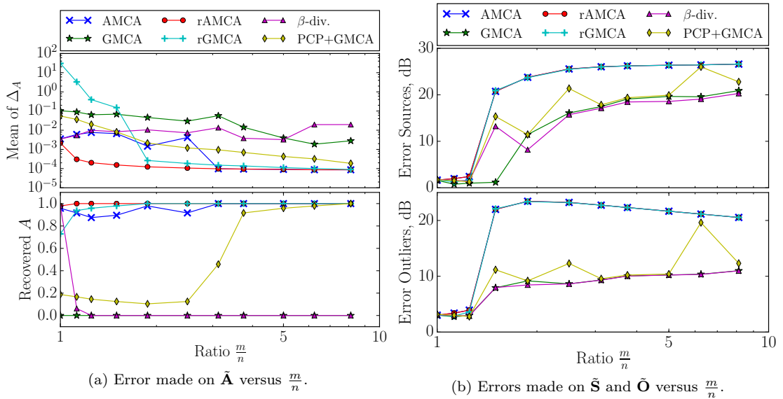
Figure 4.11: Influence of the number of observations on the estimations of \mathbf{A} , \mathbf{S} and \mathbf{O} .
