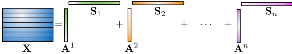
Figure 1.5: Illustration of the underlying structure of multivalued data with the LMM model.
