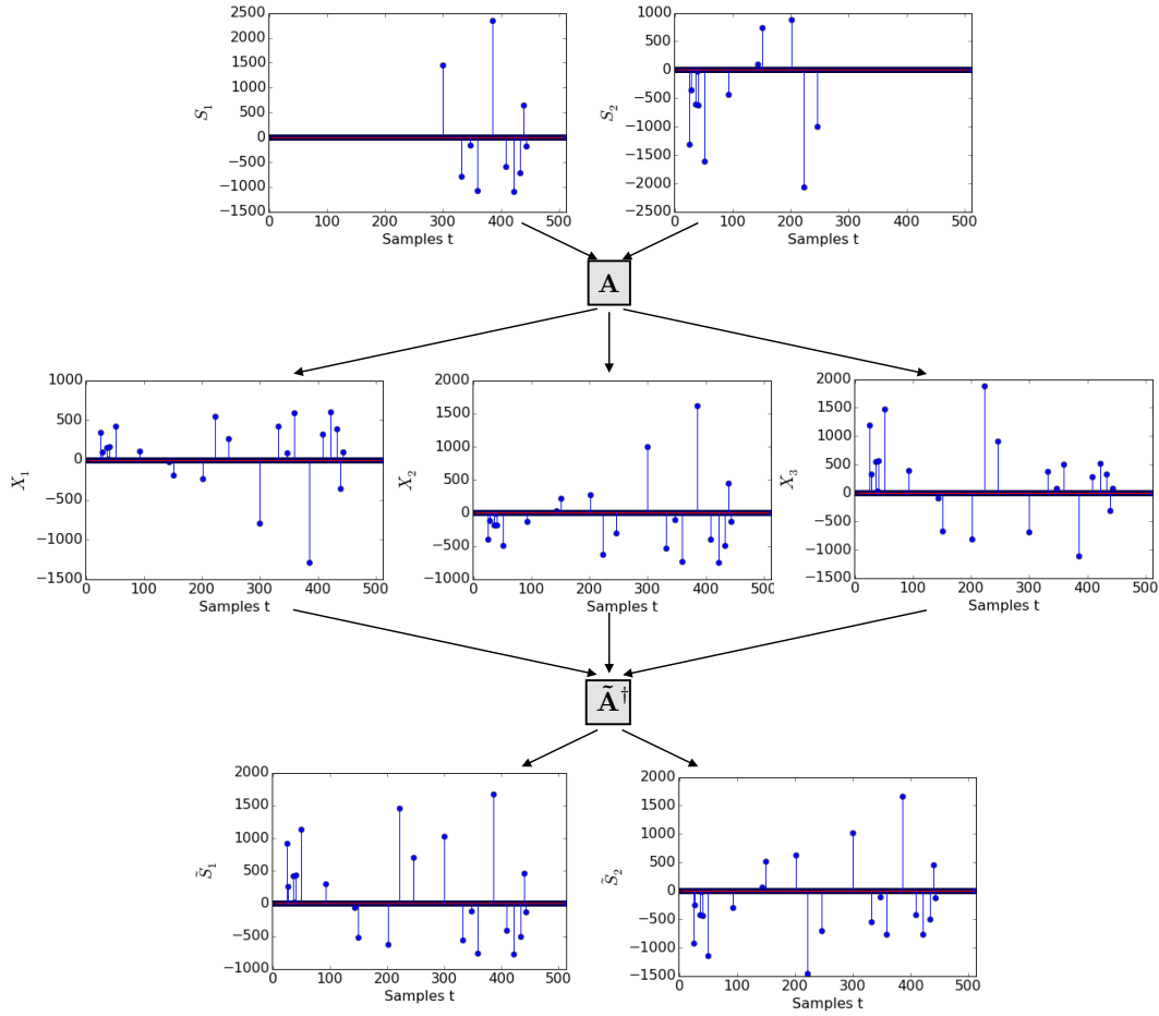
Figure 1.10: Two exactly sparse sources \mathbf{S}_1 and \mathbf{S}_2 are mixed with \mathbf{A} into 3 noiseless observations \mathbf{X} . Two estimated sources \tilde{\mathbf{S}} , given by \tilde{\mathbf{A}}^\dagger \mathbf{X} (noiseless case) are represented. In this case, the tuple (\tilde{\mathbf{A}}, \tilde{\mathbf{S}}) fits perfectly the observations \mathbf{A}\mathbf{S} = \tilde{\mathbf{A}}\tilde{\mathbf{S}} , but the sources \tilde{\mathbf{S}} are not the ones that we are looking after.
