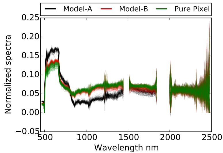
Figure 6.21: Normalized spectra of pure pixels of water and comparison with the corresponding local spectra obtained by Model A and Model B.
