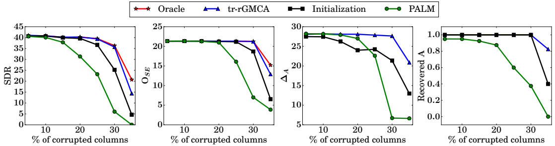
Figure 5.3: Performance indicators for a varying percentage of corrupted columns in the determined case for different optimization strategies.
