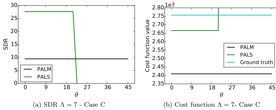
Figure 3.8: Variations of the SDR and cost function values for PALS and PALM and \Lambda = 7
