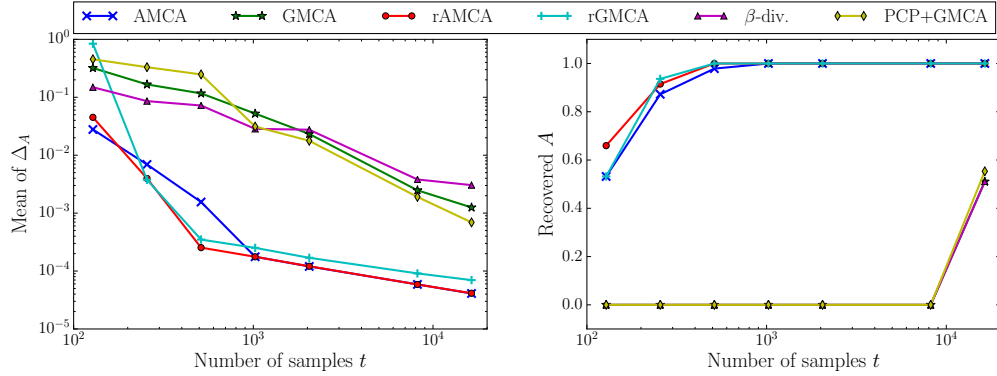
Figure 4.13: Performance results of the methods versus the number of samples t .
