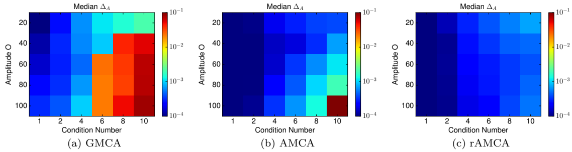
Figure 4.12: Median over 20 runs of \Delta_A for varying \mathbf{A} and amplitude of the outliers.
