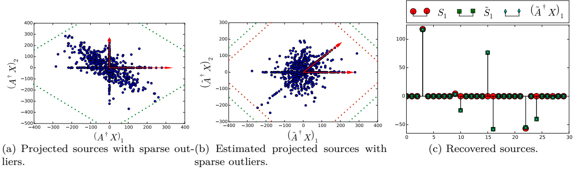
Figure 2.8: Left: scatter plot of (A^\dagger X)_1 versus (A^\dagger X)_2 with sparse outliers. Middle: scatter plot of (\tilde{A}^\dagger X)_1 versus (\tilde{A}^\dagger X)_2 with sparse outliers. The green dashed lines symbolize the \ell_1 ball in which is enclosed (A^\dagger X) and the red dashed lines the \ell_1 ball enclosing (\tilde{A}^\dagger X) . Right: some of the samples of the recovered source \tilde{S}_1 . The tuple (\tilde{A}, \tilde{S}) is estimated with GMCA.
