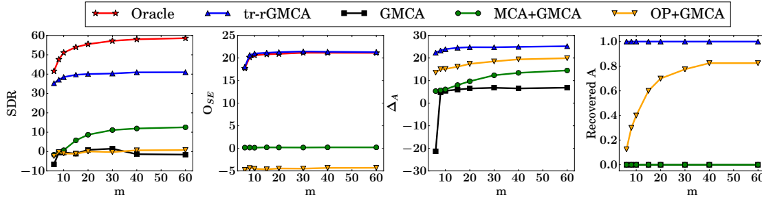
Figure 5.8: Performance indicators for a varying number of observations, m , for 6 sources.
