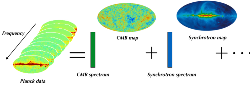
Figure 1.2: Illustration of the underlying data model with the Planck data.
