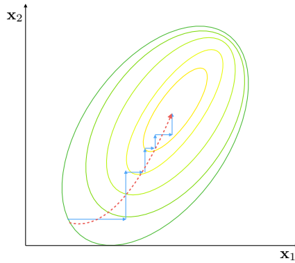
Figure 3.5: Illustration of the minimization paths for BCD (blue), and PALM (red), with two components \mathbf{x}_1 and \mathbf{x}_2 . The cost function is represented by some of its level sets, the yellower, the lower.
