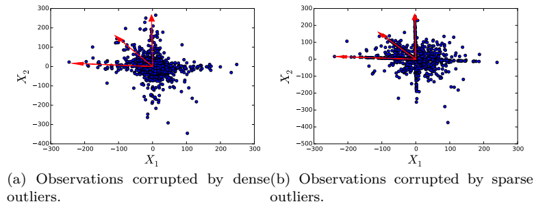
Figure 2.6: Left: scatter plot of \mathbf{X}_1 versus \mathbf{X}_2 when the observations are corrupted by dense outliers. Right: scatter plot of \mathbf{X}_1 versus \mathbf{X}_2 when the observations are corrupted by sparse outliers, with a same energy. The red arrows symbolize the directions of \mathbf{A} .
