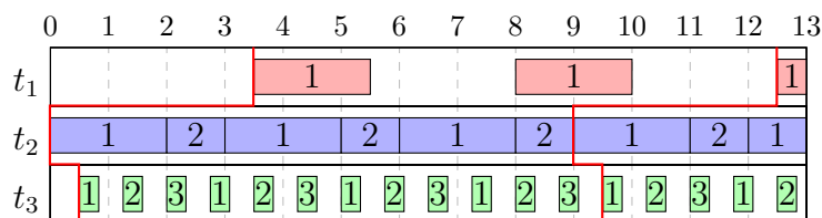
Figure 3.9 – One-periodic schedule for the CSDFG of Figure 3.8(a). Since the repetition vector of the graph is R = [2, 3, 4] and the iteration period is T = 9 , the tasks have periods w_1 = 4.5 , w_2 = 3 and w_3 = 2.25 . The red lines delimit the first iteration.
