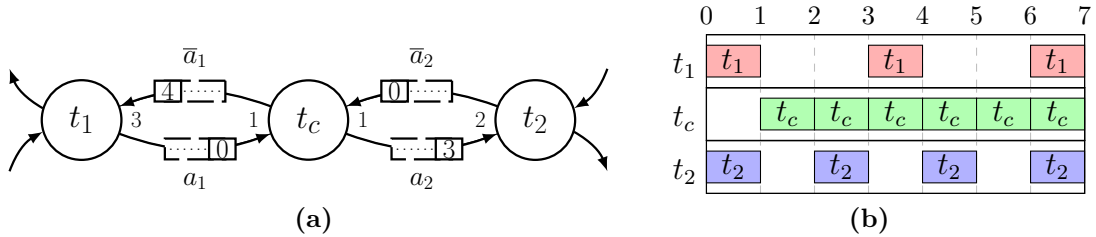
Figure 5.9 – (a) The bounded buffer a = (t_1, t_2) of Figure 5.8(a) when distributed between two clusters. (b) One-periodic schedule for the bounded buffer between two clusters with period T = 6 .
