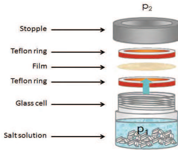
Figure 3.14. Water vapour permeation cell.
