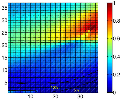
Diebold-Mariano test results on RMSE
