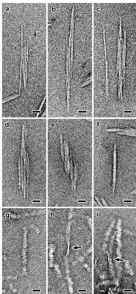
Figure 30 – Higher magnification TEM images of CN-I (a-c), MCN-II (d-f) and RCN-II (g-i) particles (negative staining). The arrows in (h) and (i) indicate twist regions. Scale bars: 20 nm.
