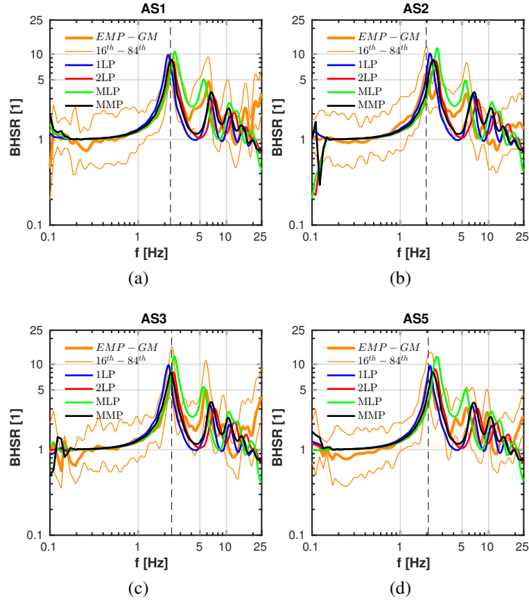
Figure 2.15: Theoretical transfer function for borehole KK5, compared to the Empirical ones along the generic X-Y directions for (a) aftershock 1, (b) aftershock 2, (c) aftershock 3 and (d) aftershock 5. EMP-GM represents the geometric mean transfer function on different in-plane rotation angles \theta \in [0^\circ; 180^\circ] . 16 th -84 th percentiles of Empirical borehole spectral ratios are plotted as thin orange lines.
