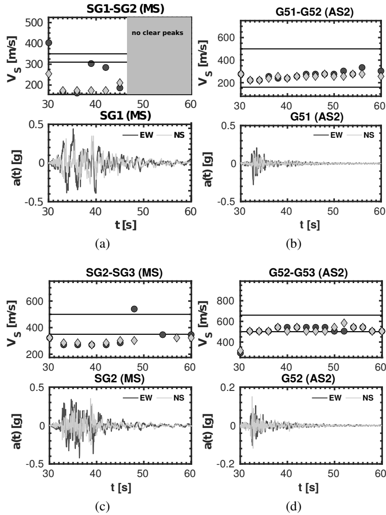
Figure 2.11: V_S values estimation by borehole interferometry (along the EW-NS directions, dark grey circles and light grey diamonds, respectively); solid black lines indicate average V_S values (from PS-log) at the two devices' locations. The EW-NS time-histories are shown along side, for (a) main shock at KSH (seismometers SG1-SG2); (b) aftershock 2 at KK5 (seismometers G51-G52); (c) main shock at KSH (seismometers SG2-SG3); (d) aftershock 2 at KK5 (seismometers G52-G53).
