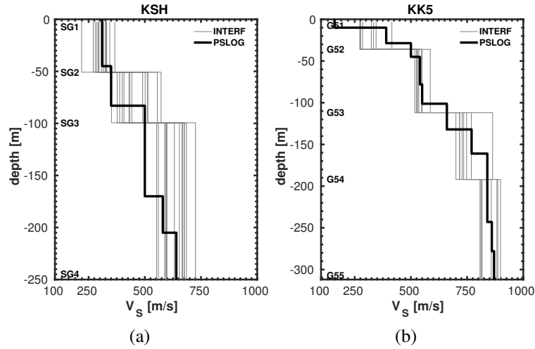
Figure 2.12: V_S profile obtained by averaging EW-NS results from borehole interferometry analysis on the two arrays KSH (instruments SG1 to SG4 at depths GL-2.4, -50.8, -99.4 and -250 m respectively) and KK5 (instruments G51 to G55 at depths GL-2.7, -36, -112, -192 and -312 m respectively). Computed profiles are compared with the PS-logging one (black line) provided by TEPCO (2008).
