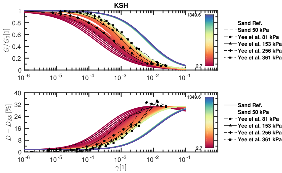
Figure 2.20: \frac{G}{G_{max}} - \gamma - D curves for KSH site. Experimental data from laboratory tests conducted by the Tokyo Soil Research (Yee et al., 2011) and by TEPCO are compared to curves used in equivalent linear analysis (MLP V_S profile), obtained by applying the overburden stress correction proposed by Yee et al. (2011).
