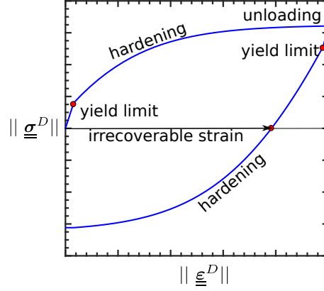
Figure 3.5: Typical non-linear strain-stress curve.
