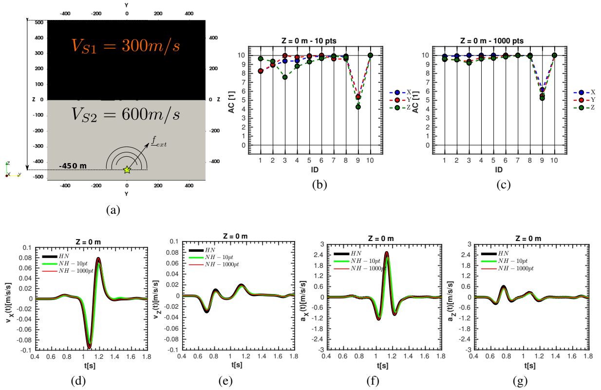
Figure 3.4: (a) Example of bi-layered domain. (b-c) Anderson’s criteria values for the three components of motion simulated at the material discontinuity ( Z=0 m): the honouring approach is compared to the not-honouring one, with 10 points (b) and 1000 points (c) of discretization respectively. Velocity (d-e) and Acceleration (f-g) time-histories obtained at the interface between layers 1 and 2, by employing an honouring ( HN , black line) and not-honouring (coarse NH - 10pt , green line, and fine NH - 1000pt , red line) approach respectively.
