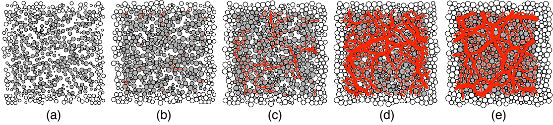
Figure 1.1: Compression stage during the preparation of the REV, from the resultant gas like configuration after shaking (a) to the final dense packing in (e) passing by different compaction stages during the process (b,c,d) in which new force chains are created (red lines).
