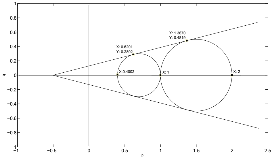
Figure 3.20: Mohr circles and failure envelope in the q - p plane. The failure envelope corresponds to the residual values of compression and extension tests in (Fig. 3.19). Results: residual friction angle 18^\circ and cohesion 0.125 stress units.
