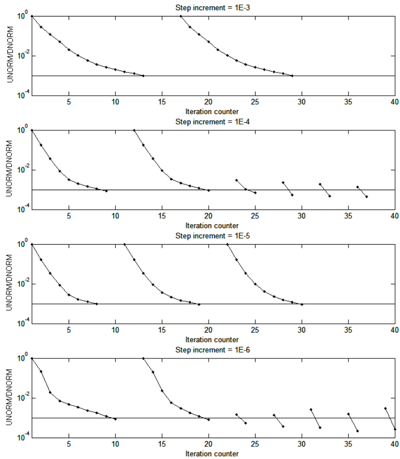
Figure 2.11: Deficit of compatibility for the norm of the displacement (UNORM/DNORM) for four different initial step size: \epsilon_2 = 1 \cdot 10^{-3} , \epsilon_2 = 1 \cdot 10^{-4} , \epsilon_2 = 1 \cdot 10^{-5} , \epsilon_2 = 1 \cdot 10^{-6} . Kruyt operator. The horizontal line indicates the precision threshold.
