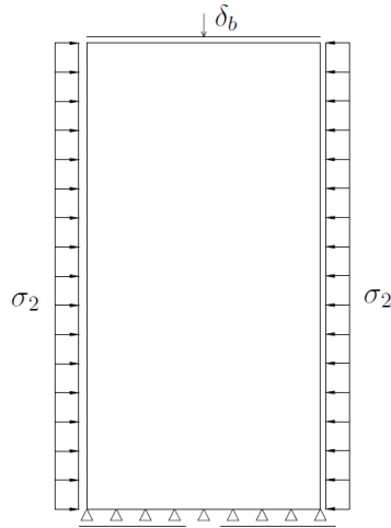
Figure 4.3: Biaxial test geometry and boundary conditions
