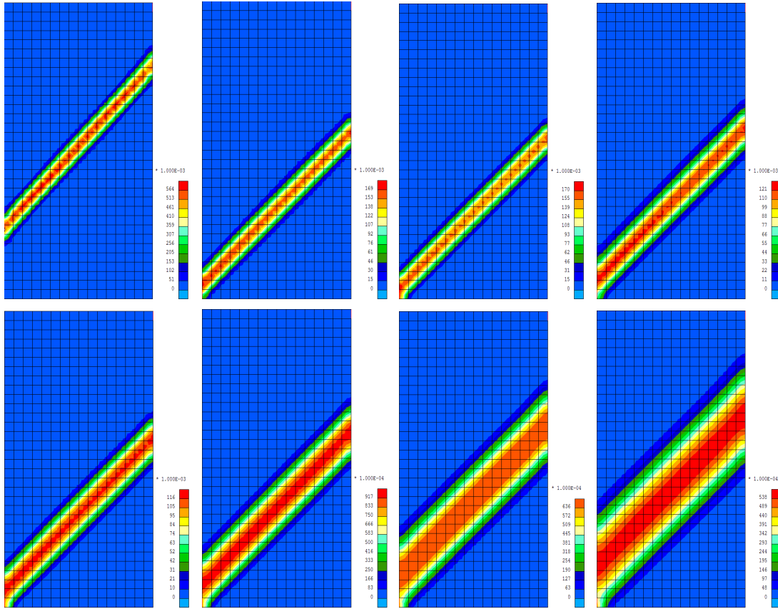
Figure 4.4: Second invariant of strain at 2,5% axial strain (constant pressure biaxial test with 512 elements). Parametric study of the second gradient value D . Respectively: D = no second gradient,31,63,125,250,500,1000 and 2000.
