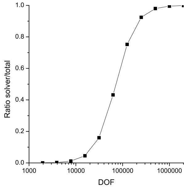
Figure 5.5: Ratio solver time/total time for a non parallelized problem.
