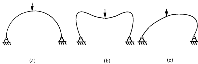
Figure 2.4: (a) The simply supported arch; (b) symmetric deformation; (c) asymmetric deformation. (Shi and Crisfield, 1992)
