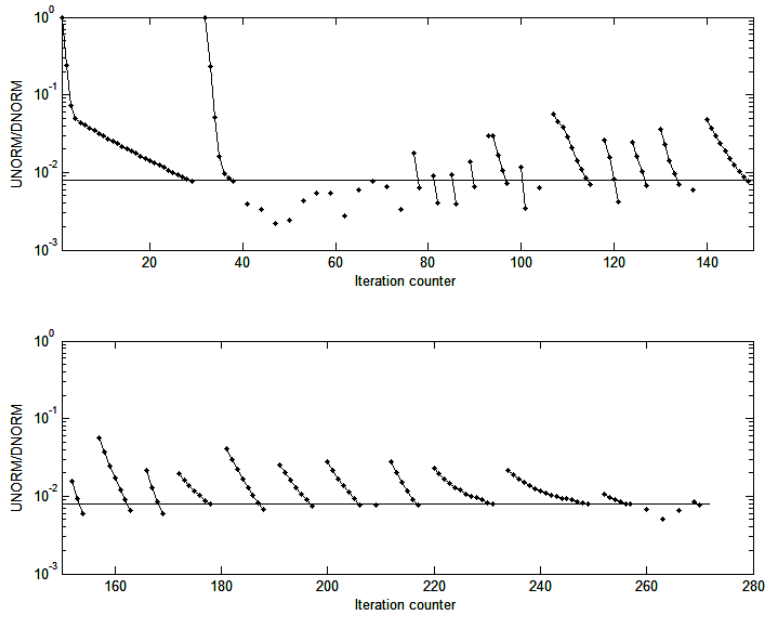
Figure 3.7: Deficit of compatibility for the norm of the displacement (UNORM/DNORM) for a 512 element biaxial test without defect. Kruyt operator. The horizontal line indicates the precision threshold.
