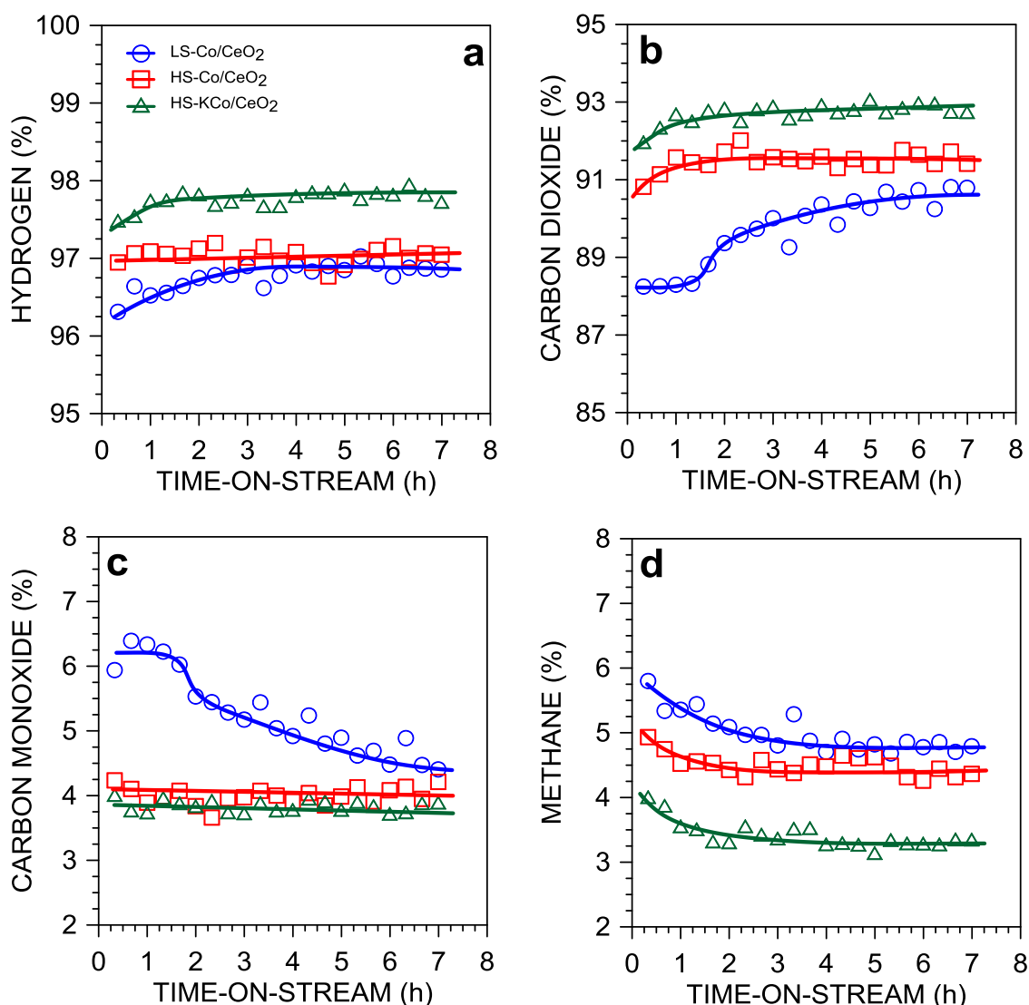
Fig. 6. The effect of time-on-stream on ceria-supported catalysts' selectivity towards hydrogen, carbon dioxide, carbon monoxide and methane ( \text{H}_2\text{O}/\text{EtOH} = 12/1 mol/mol, 420^\circ\text{C} , p_{\text{total}} = 1 atm).
