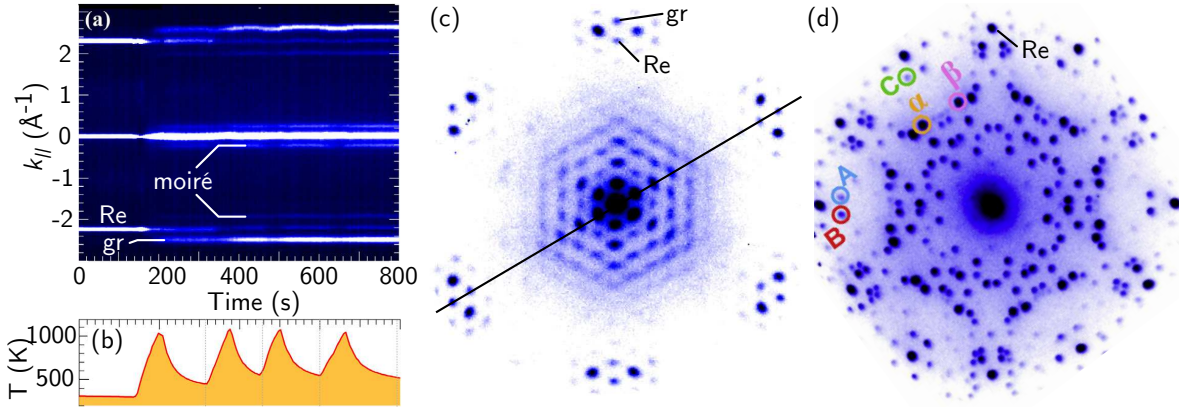
Figure 3.5: Graphene and carbide formation on Re(0001) . (a) LEED line profile evolution during graphene growth on Re(0001), following annealing-cooling cycles indicated by the temperature evolution (b). (c) LEED pattern for high quality graphene on Re(0001), with the cut taken for the profile (a). Spots due to graphene, rhenium are indicated, while all the others are due to the moiré superlattice. (d) LEED pattern of the surface carbide, with six-fold symmetry due to the coexistence of rotated carbide domains. Adapted from [143].
