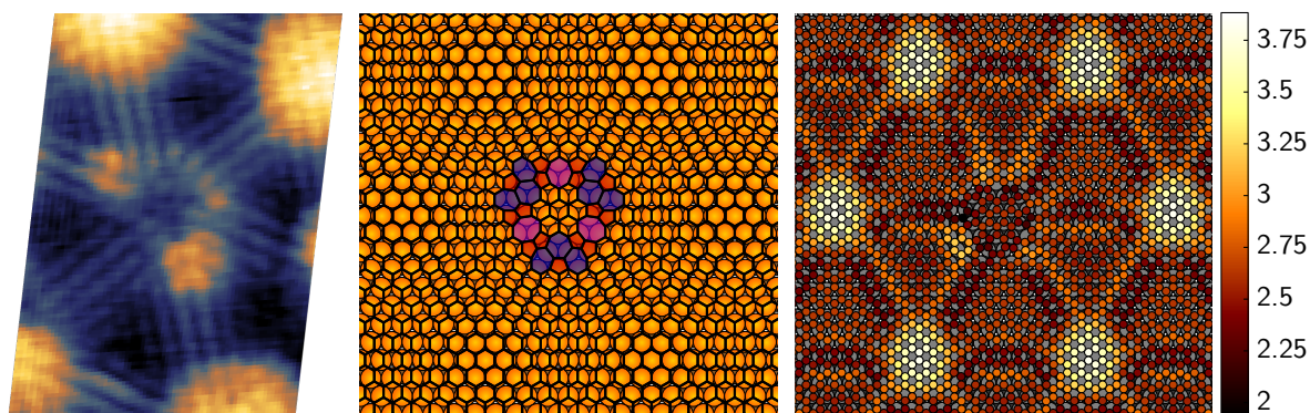
Figure 5.19: Missing hill defect. Left: STM topograph ( V_b = 30 mV and I_t = 6 nA, scale bar 1 nm) of full layer graphene with a defect positioned where a moiré hill is expected, lowering its apparent height. Middle: interpreted atomic structure of this kind of defect, where a grain boundary loop stabilizes the core of the defect on top-fcc sites instead of the hcp-fcc registry of intact neighbouring moiré hills. Right: atomic structure converged by atomistic simulations of a large unit cell containing 1 defective missing hill and 15 intact moiré hills. Carbon atoms are coloured depending on their z position (taken from substrate, in Å), revealing the atoms in the missing hill lie close to the substrate.
