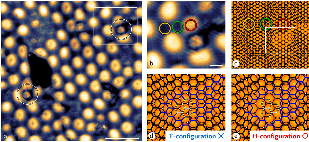
Figure 5.14: Carbon nanocluster incorporation. (a) STM topograph ( V_b = 30 mV and I_t = 6 nA, 20 \times 20 nm 2 ) showing two of the smallest carbon nanoclusters (circled) surrounded with a continuous graphene layer. (b) Close-up view of one of the nanocluster, where the typical hcp-fcc, top-fcc and top-hcp of the moiré superlattice are circled respectively in red, green and orange. (c) Ball and stick interpretation of the graphene and substrate atomic structures. (d-e) Tentative incorporation of either T- or H-configured nanocluster. Only the H-configuration yields the observed blocked incorporation.
