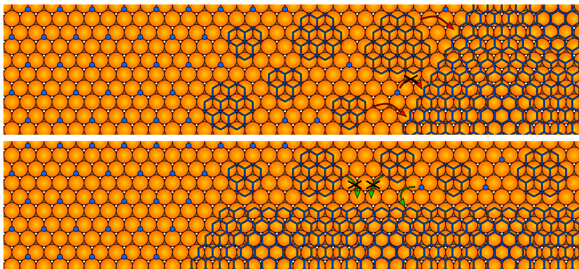
Figure 5.13: Growth scenarios: ball and stick models representing the two typical growth scenarios, with chronological order from left to right. Top: carbon nanoclusters as intermediates. Carbon adatoms first form a (2 \times 2) superstructure, then assemble into carbon nanoclusters, which act as necessary intermediates in the growth of a graphene layer. Bottom: carbon nanoclusters as competitors. Carbon adatoms, initially in a (2 \times 2) arrangement, form simultaneously carbon nanoclusters and graphene. However, the carbon nanoclusters are kinetically blocked from incorporating the graphene layer.
