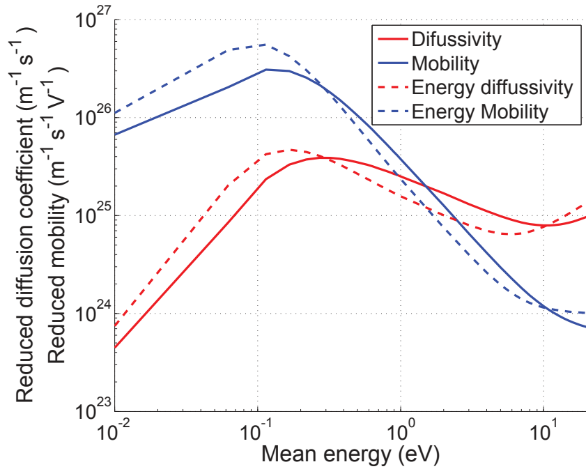
Figure 4.2: Reduced transport coefficients of a Maxwellian electron population in argon gas as a function of the mean electron energy.
