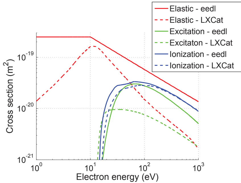
Figure 3.7: LXCat [51] vs. EEDL [50] electron-impact cross sections for elastic, inelastic and ionization collisions in argon. The different scope of each database (eV range for LXCat, keV and higher for EEDL) results in different values of each database for the same collision in the overlapping region.
