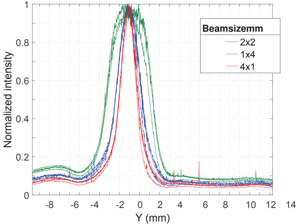
Figure 2.9: Scan of the OES signal along the vertical direction, for 400 mbar Ar and an X-ray beam of 6 mm gap in the undulator and a variable beam size (shown in the legend). The channel intensities have been normalized to its maximum value to simplify the comparison.
