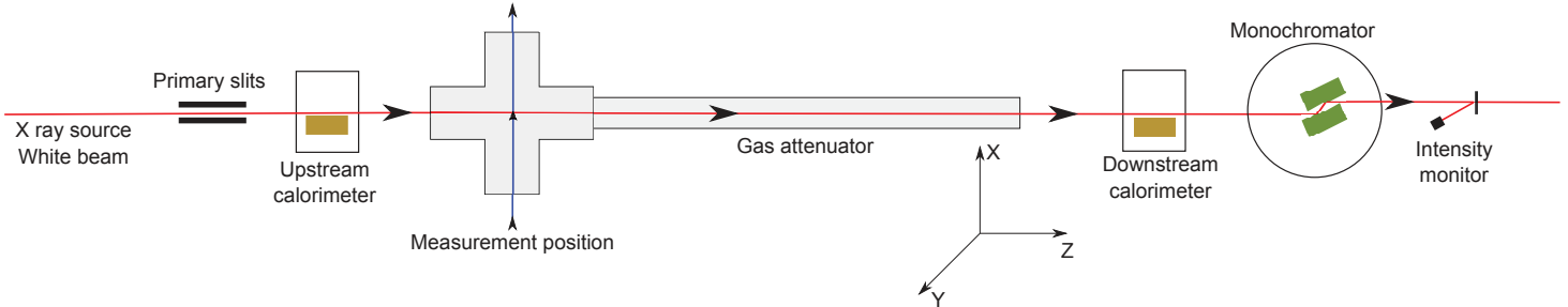
Figure 2.2: Setup of the beamline for the optical and power absorption measurements.
