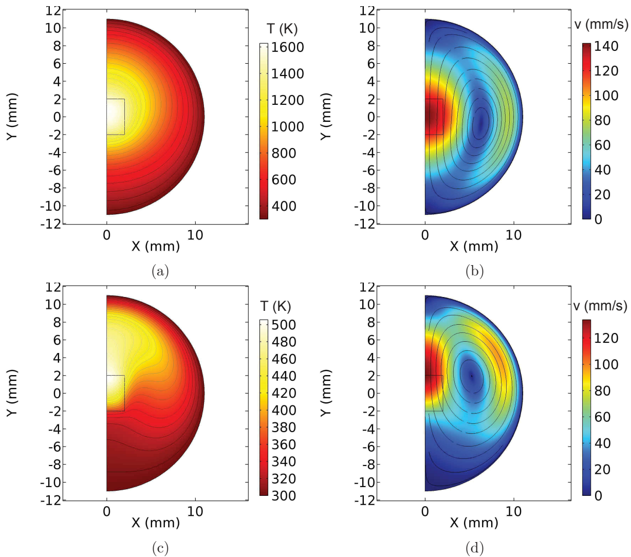
Figure 4.7: Temperature and velocity distributions from the heat transfer simulations, for 200 mbar of pressure and 100 W input power (a and b) and 400 mbar and 20 W (c and d). The solid lines represent isothermal curves in the temperature plots and streamlines in the velocity plots. The color legend represents the intensity of temperature and velocity respectively.
