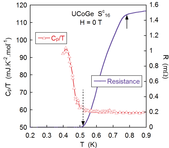
Figure 3.1 | Superconducting transition probed with specific heat (red triangles) and resistivity (purple line) of UCoGe (sample S_{16}^c ). The onset of the bulk superconducting transition in specific heat lies close to the temperature at which the resistivity becomes zero (marked by the broken line). The onset of the resistivity transition lies much higher in temperature (marked by the up arrow).
