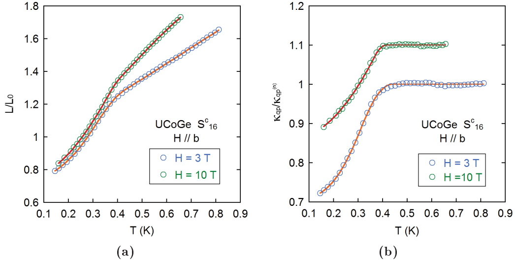
Figure 3.7 | (a): The Lorenz ratio L/L_0 as a function of temperature, obtained from the measurements at 3 T and 10 T for \mathbf{H} // \mathbf{b} . The solid lines present the corresponding fit F_{other}(T) + F_{qp}(T) (explained in the text). (b): The normalized quasiparticle contribution to thermal conductivity \kappa_{qp}/\kappa_{qp}^{(n)} as a function of temperature, obtained from the measurements at 3 T and 10 T for \mathbf{H} // \mathbf{b} . The solid lines present the corresponding fit F_{qp}(T) .
