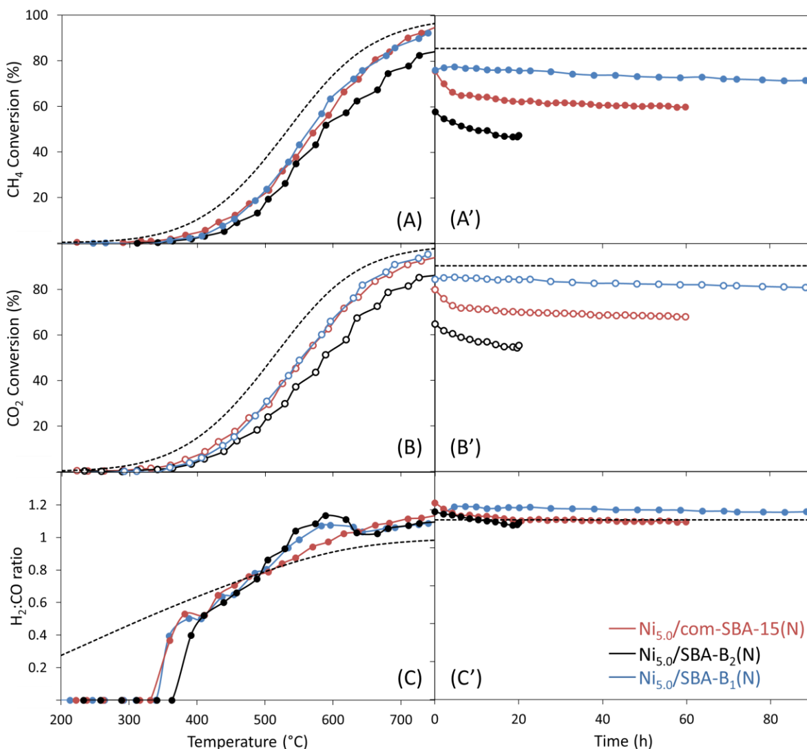
Figure IV-7: Variation of (A,A') CH 4 conversion, (B,B') CO 2 conversion and (C,C') H 2 :CO ratio as a function of temperature (A,B,C) and time at 650°C (A',B',C') at 1bar, 36 L.g -1 .h -1 and CH 4 :CO 2 :Ar = 5:5:90 (dashed lines represent thermodynamic data under the used conditions)
