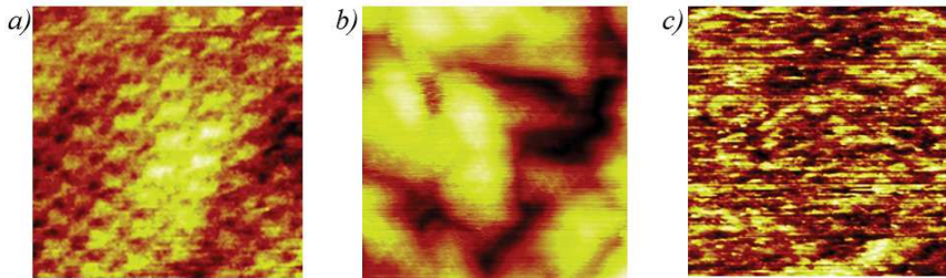
Figure 2.6: Structural characterization of the self-assembled a) PTCDI-C13 ( 18\text{nm} \times 18\text{nm} , 10\text{pA} , -800\text{mV} ), b) PTCDI-JT pedestal ( 75\text{nm} \times 75\text{nm} , 3\text{pA} , -1350\text{mV} ) and c) 1:1 ratio of PTCDI-JT and PTCDI-JT pedestal ( 38\text{nm} \times 38\text{nm} , 5\text{pA} , -1560\text{mV} ) monolayers on graphene on PET. The images were acquired at the interface between the substrate and a 10^{-5}\text{M} solution in phenyloctane at room temperature.
