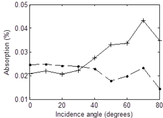
Figure 1.25: Variable incidence polarized-transmission analysis of the contribution of the self-assembled PTCDI-C7 monolayer to the absorption (cross: TM, points: TE). The mean optical density around the absorption maximum (460 nm to 500 nm) is plotted.
