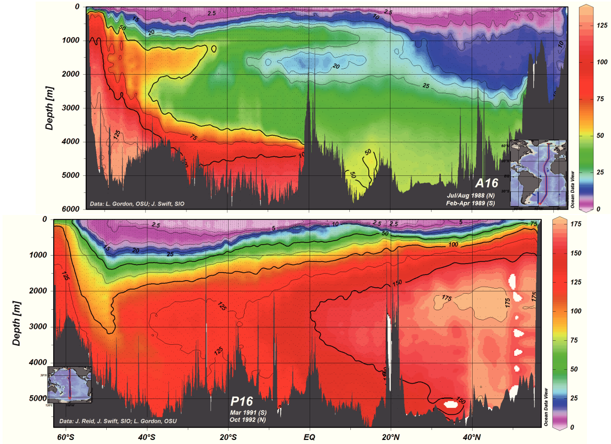
Figure 1.2 Longitudinal section across the entire Atlantic Ocean (top panel) and Pacific Ocean (bottom panel) of the DSi concentration versus depth (eWOCCE, Schlitzer, 2000).
