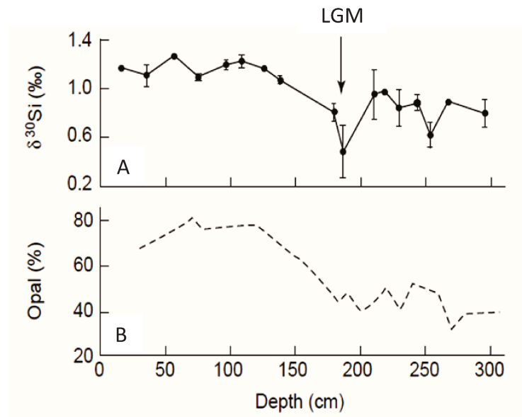
Figure 1.8 Representation of the South Atlantic sediment core RC13-269 (52°38' S, 00°08' W, 2,591 mbsl) for the A) \delta^{30}\text{Si} evolution versus depth, error bars on \delta^{30}\text{Si} represent standard error on 2–3 separate measurements, the arrow indicates the Last Glacial Maximum (LGM) and B) BSi against depth. The percentage opal (P. N. Froelich, unpublished data) was determined through extraction into a sodium carbonate solution 32. Modified from De La Rocha et al. (1998).
