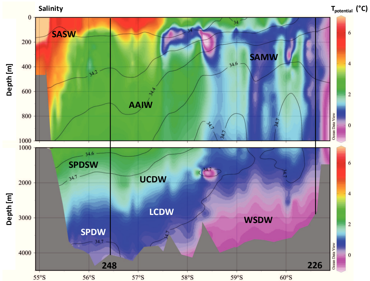
Figure 4.9 Latitudinal transect of Drake Passage realized with data from ANTXXIV/3 campaign. Our stations 248 and 226 are indicated by vertical lines. Thin horizontal lines indicate salinity boundaries. Potential temperature colour maps were created with ODV (Schlitzer, Ocean Data View, http://odv.awi.de , 2013) using data from ANTXXIV/3 campaign. SASW: Subantarctic surface Water, SAMW: Subantarctic Mode Water, AAIW: Antarctic Intermediate Water, SPDSW: Southeast Pacific Deep Slope Water, UCDW: Upper Circumpolar Deep Water, LCDW: Lower Circumpolar Deep Water, SPDW: Southeast Pacific Deep Water, WSDW: Weddell Sea Deep Water.
