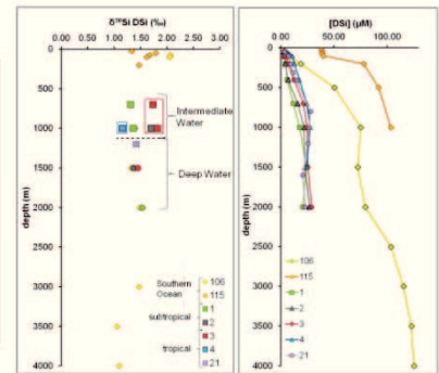
Intermediate and deep water from the sub-tropic to the prime meridian
