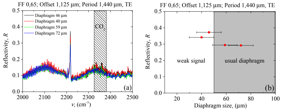
Figure 7.28: (a) Spectral reflectivity of CVL4C9_14_1 CRIGF filter with FF=0.65 , offset= 1.125 \mu\text{m} and period= 1.440 \mu\text{m} obtained for different sizes of the diaphragm (illumination spots of the diffraction grating). (b) Maximum of the reflectivity peaks as a function of diaphragms size.
