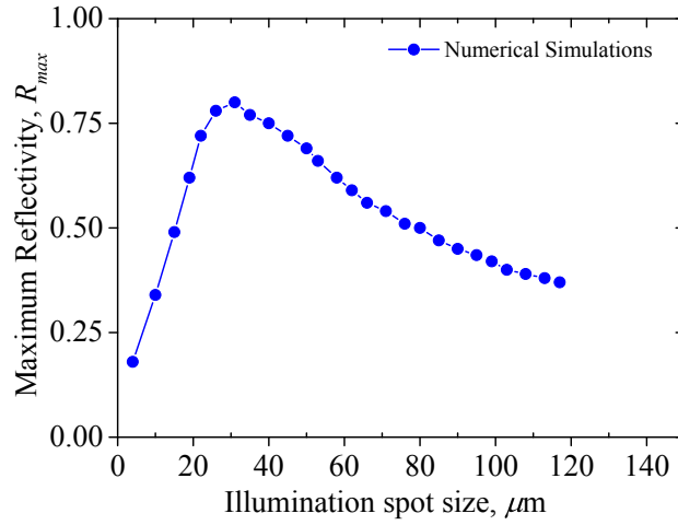
Figure 7.29: RCWA numerical results for the maximum of the reflectivity peaks of CVL4C9_14_1 CRIGF filter with FF = 0.65 , offset = 1.125 \mu m and period = 1.440 \mu m as a function of diaphragm sizes. These results are obtained by our partners at Institute Fresnel.
