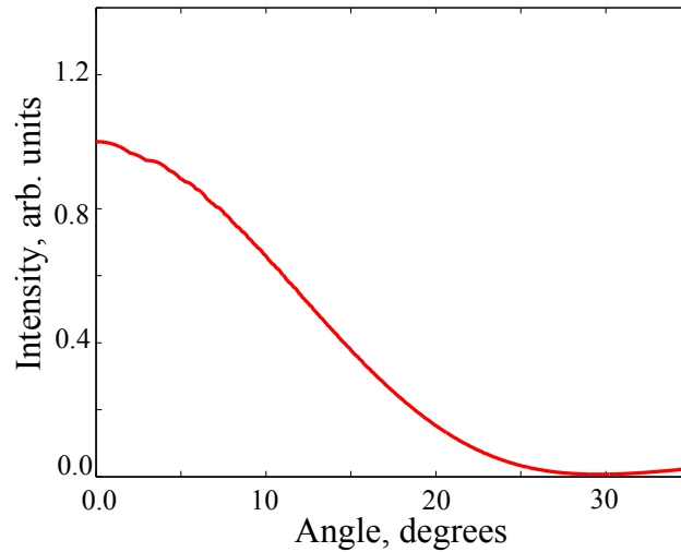
Figure 4.8: Intensity of diffraction of an electromagnetic monochromatic plane wave of wavelength \lambda = 10.9\ \mu\text{m} which corresponds to the frequency f = 27.5\ \text{THz} , and the slit width d = 21\ \mu\text{m} as a function of the observation angle. The angle of diffraction \alpha = 29.7^\circ is defined as the angle of the first dark zone. The result is obtained by post-treatment of FDTD simulations.
