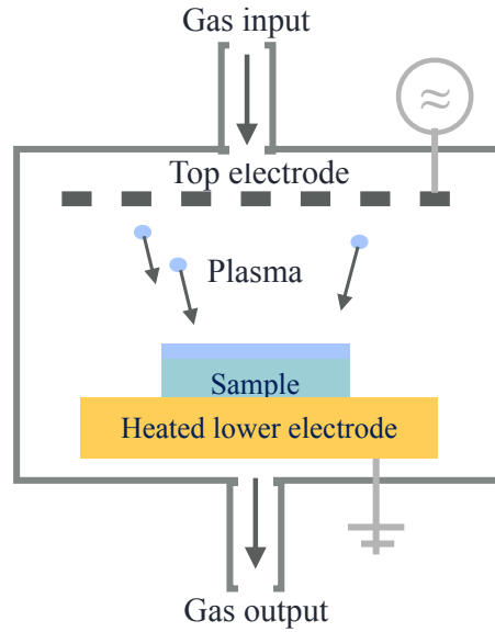
Figure 6.12: Illustration of the Plasma Enhanced Chemical Vapor Deposition (PECVD) process of a thin \text{SiO}_2 layer.
