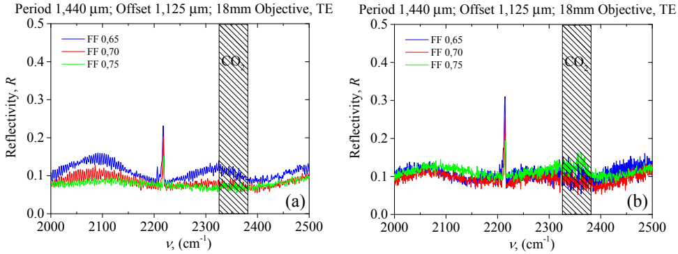
Figure 7.24: Spectral reflectivity of CVL5C9_6_1 sample generation (a) and CVL4C9_14_1 sample generation (b) of diffraction gratings for different CRIGF filters filing factors with same offset = 1.125 \mu\text{m} and period = 1.440 \mu\text{m} . The results are obtained with WD = 18 \text{ mm} ZnSe objective for TE polarization.
