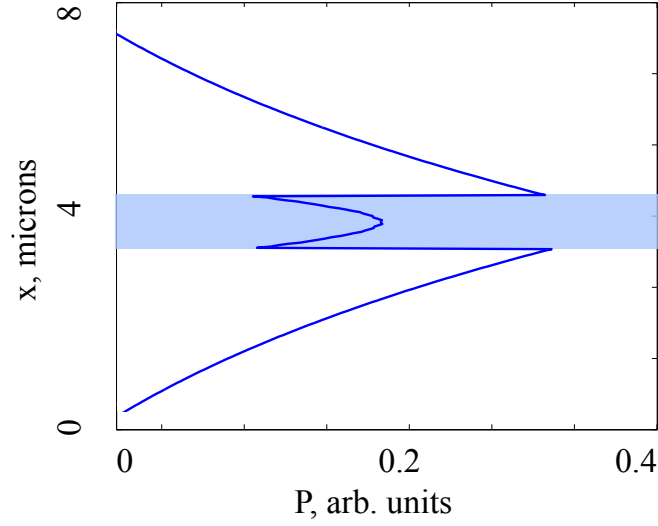
Figure 6.5: Energy density profile along the x axis of a Zenneck mode bounded to the interfaces of a 1\ \mu\text{m} thick suspended \text{SiO}_2 membrane. The result is obtained by FDTD numerical simulations by using the excitation frequency \nu = 900\ \text{cm}^{-1} where the relative permittivity of \text{SiO}_2 satisfies Zenneck mode condition ( \epsilon_r > 0 and \epsilon_i > 0 ). The scale is in arbitrary units.
