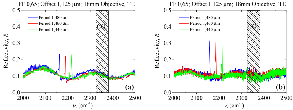
Figure 7.22: Spectral reflectivity of CVL5C9_6_1 sample generation (a) and CVL4C9_14_1 sample generation (b) of a diffraction gratings for different CRIGF filters periods with same FF = 0.65 \mu\text{m} and \text{offset} = 1.125 \mu\text{m} . The results are obtained with WD = 18 mm ZnSe objective for TE polarization.
