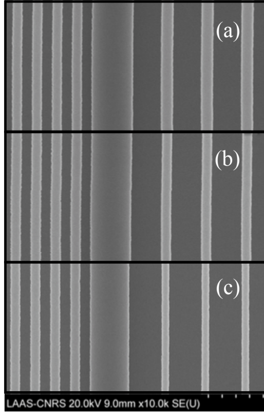
Figure 7.25: SEM images of CVL4C9_14_1 CRIGF filters for different filling factors: (a) FF=0.65 , (b) FF=0.70 , and (c) FF=0.75 . The offset= 1.125\ \mu\text{m} and period= 1.440\ \mu\text{m} are the same for all samples. The results are obtained by LAAS partners.
