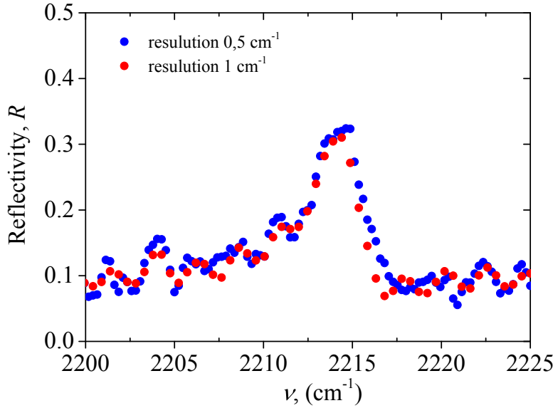
Figure 7.26: Spectral reflectivity of CVL4C9_14_1 CRIGF filter with FF=0.65 , \text{offset}=1.125 \text{ }\mu\text{m} and \text{period}=1.440 \text{ }\mu\text{m} measured with usual 1 \text{ cm}^{-1} resolution and 0.5 \text{ cm}^{-1} resolution with 256 and 1024 scans, respectively.
