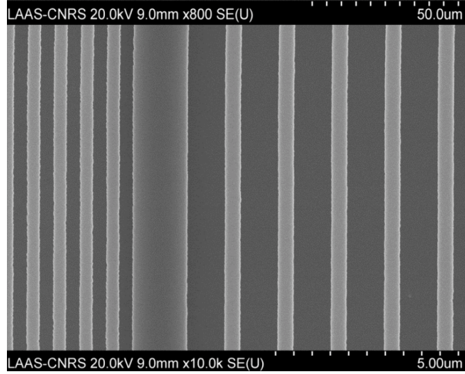
Figure 7.7: SEM image of a CRIGF filter with 1.460\ \mu\text{m} period, FF=0.65 , and 1.125\ \mu\text{m} offset zoomed on the border of Bragg grating (right side) with diffraction grating (left side) with offset region (wide strip in the middle). The results are obtained by LAAS group.
