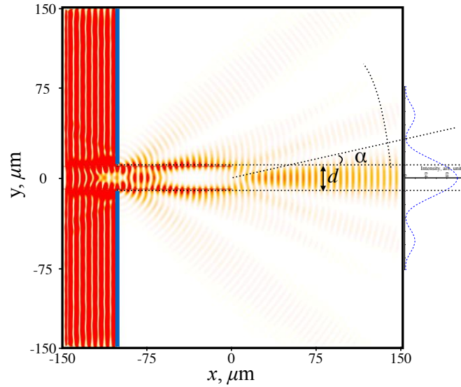
Figure 4.11: Intensity of diffraction of an electromagnetic monochromatic plane wave of wavelength \lambda = 10.9 \mu\text{m} which corresponds to the frequency f = 27.5 \text{ THz} , and the slit width d = 21 \mu\text{m} , with glass suspended membranes embedded. The thickness of the membranes is h = 1 \mu\text{m} , the suspension length L = 100 \mu\text{m} . Red color stands for larger values of the intensity. The blue line shows the metallic plane with an aperture. The right side blue dashed curve demonstrates the intensity profile along the wavefront. The result is obtained by FDTD simulations.
