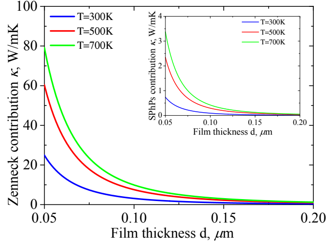
Figure 6.31: Theoretical calculation of the in-plane thermal conductivity of an amorphous glass membrane as a function of its thickness calculated for different temperatures by considering both Zenneck and SPhP modes. The inset plot displays the same results obtained by considering only SPhPs modes Ordóñez-Miranda, Tranchant, Tokunaga, Kim, Palpant, Chalopin, Antoni, and Volz (2013) .
