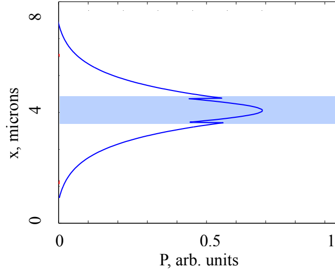
Figure 6.6: Energy density profile along the x axis of a TM guided mode bounded to the interfaces of a 1\ \mu\text{m} thick suspended \text{SiO}_2 membrane. The result is obtained by FDTD numerical simulations by using the excitation frequency \nu = 2500\ \text{cm}^{-1} where the relative permittivity of \text{SiO}_2 satisfies TM guided mode condition ( \epsilon_r > 0 and \epsilon_i \approx 0 ).
