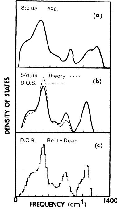
Figure 6.29: Density of states of phonons in amorphous \text{SiO}_2 reported by R.B. Laughlin and J.D. Joannopoulos obtained by neutron measurements (a), by calculating average density of states (solid line) and by comparing with experimental data (dashed line) (b), by theoretical modelling with random-network model (c). The results are demonstrated in the work of R.B. Laughlin and J.D. Joannopoulos Laughlin and Joannopoulos (1977) .
