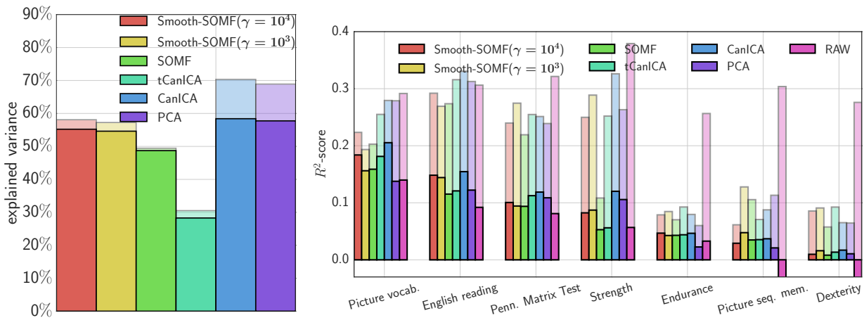
Figure 9.4: Left: Mean explained variance of the different models on both training data and test (left-out) data. N.B.: Bold bars represent performance on test set while faint bars in the background represent performance on train set. Right: Predicting behavioral variables of the HCP [van Essen et al., 2012] dataset using subject-level Z-maps.
