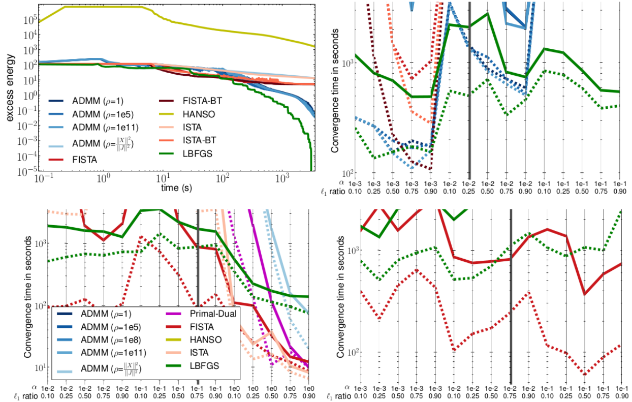
Figure 4.2: Benchmarking solvers for TV- \ell_1 penalized models. Top: TV- \ell_1 penalized Logistic Regression on the visual recognition face-house discrimination task. Top Left: excess energy E(\mathbf{w}_t) - E(\mathbf{w}^*) as a function of time. Top Right: convergence time of the various solvers for different choice of regularization parameters. Broken lines correspond to a tolerance of 10^0 , whilst full-lines correspond to 10^{-2} . The thick vertical line indicates the best model selected by cross-validation. Bottom: TV- \ell_1 penalized Least-Squares Regression. Bottom Left: on the visual recognition face-house discrimination task; Bottom Right: on the Mixed gambles dataset. The thick vertical line indicates the best model selected by cross-validation.
