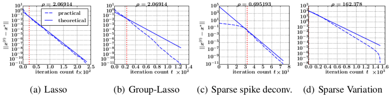
Figure 7.2: Experimental results from ICASSP paper [Dohmatob et al., 2015]. showing local Q -linear convergence for ADMM on problem (7.1). The “theoretical” line is the exponential curve t \mapsto \|x^{(0)} - x^*\| r(\Lambda'(x^*))^t . The red broken vertical line marks the instant the support of the fixed-point x^* is identified.
