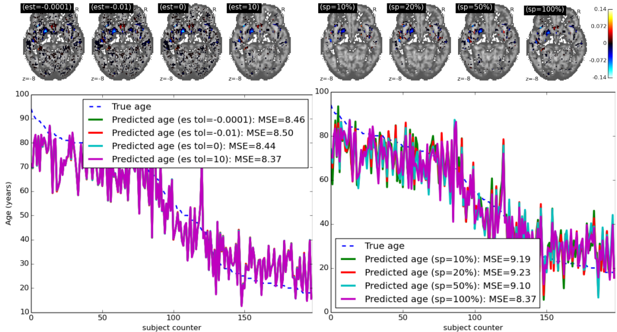
Figure 5.2: Predicting age from gray-matter concentration maps from the OASIS dataset [Marcus et al., 2007]. Top: Weights maps (solutions to problem (3.1)). Bottom-left: Mean Square Error (MSE) in age prediction, for different subjects of the validation set, for varying levels of the early-stopping tolerance (“es tol” for short), with the screening-percentile (sp) held constant at 100 (full-brain). Bottom-right: MSE in age prediction, for varying levels of the screening-percentile (sp).
