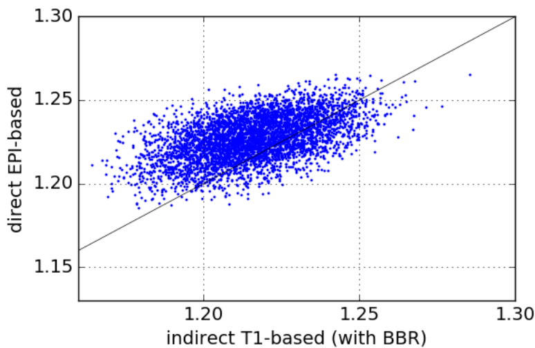
Figure 8.3: Normalized Mutual Information – NMI (higher values are better). Each point (x, y) on the plots such that x is the NMI of a given pair of subjects registered using the pipeline on the abscissa and y is the NMI of the same pair of subjects registered using the pipeline on the ordinate. From the one-sided We see that our proposed direct EPI-based pipeline significantly outperforms the classical indirect T1-based pipeline.
