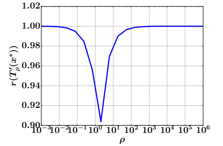
Figure 7.1: Rate of convergence r(\Lambda'_v(x^*)) as a function of v for a Lasso problem with column-rank deficient design matrix X . Taking v too small leads to badly conditioned problem (as I + (1/v)X^T X is then almost singular), and thus a slow rate of convergence (near 1). On the other hand, the figure suggests that taking v “too large” is also detrimental. Most remarkable, one notices that the basin of “good” v values is rather tight, and so care must be taken in choosing the v parameter.
