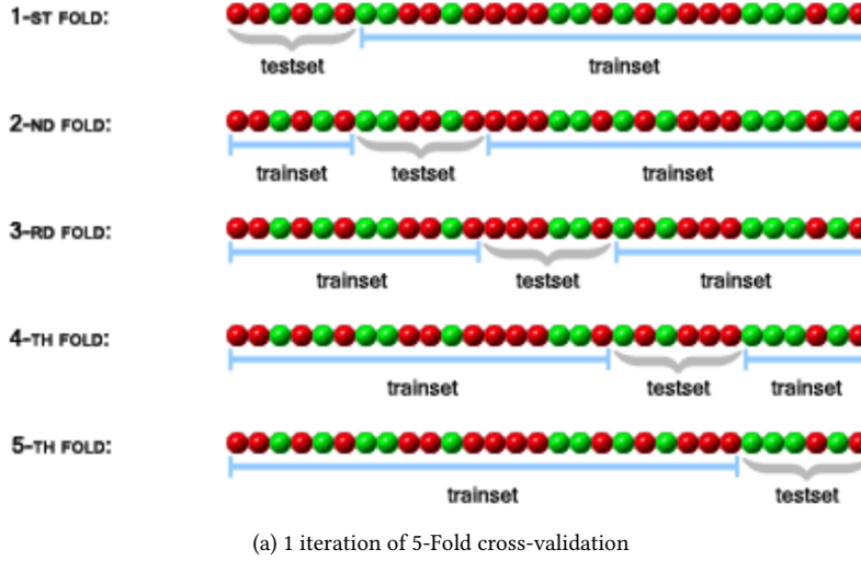
Figure 3.5: Model-selection via cross-validation. (a) K -Fold cross-validation, illustrated here for the case K = 5 , involves taking the available data and partitioning it into K groups. Then K - 1 groups are used to train a set of models that are then evaluated on the remaining group. Adapted from http://genome.tugraz.at/proclassif/help/pages/XV.html . (b) L \times M grid over which to search for optimal configuration in a model with two hyper-parameters \alpha and \rho . For a model like SpaceNet (7.1), the grid is constrained to verify 0 \leq \alpha_L < \dots < \alpha_1 = \alpha_{\max} and 0 \leq \rho_M < \dots < \rho_1 \leq 1 , with L = 10 and M = 3 typically, given a total of LM = 30 models to compare. In chapter 5, we show how early-stopping and other heuristics can be used to make the total cost much more effective than just fitting LM models in a CV loop.
