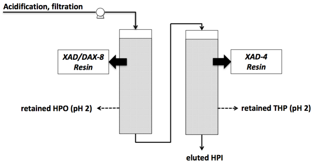
Fig. 2.5 Classical hydrophobic/hydrophilic fractionation by XAD/DAX resins.
