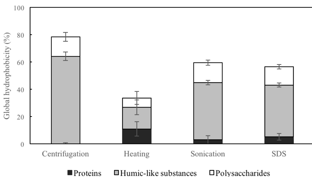
Fig. 4.3 Global hydrophobicity (%) of EPS and the contribution (%) of each EPS constituent (PN, HS-like and PS).
