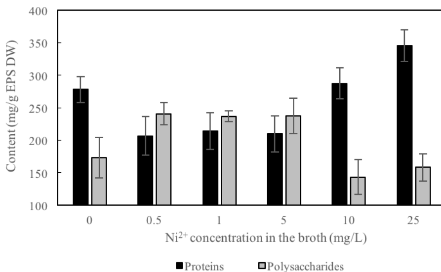
Fig. 5.4 The content of PN and PS in the EPS extracted from the fungus cultivated at different Ni 2+ concentrations.
