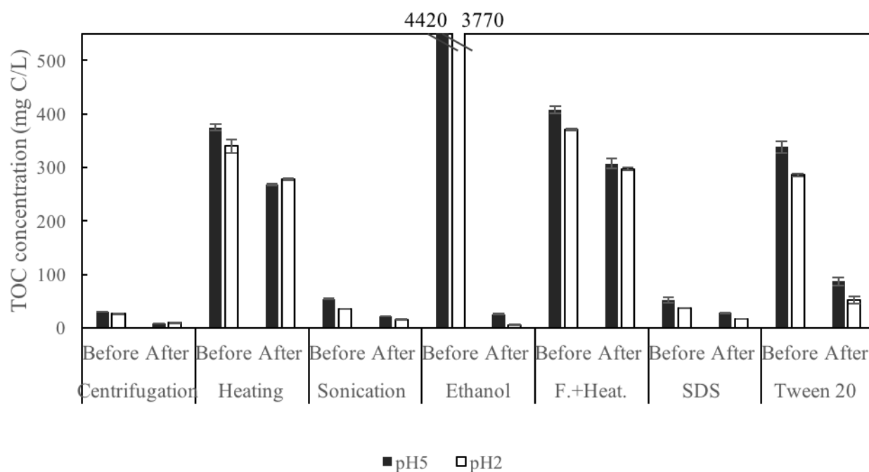
Fig. 3.4 TOC concentration of EPS extracted by different methods before and after DAX-8 treatment at pH 5 and pH 2.
