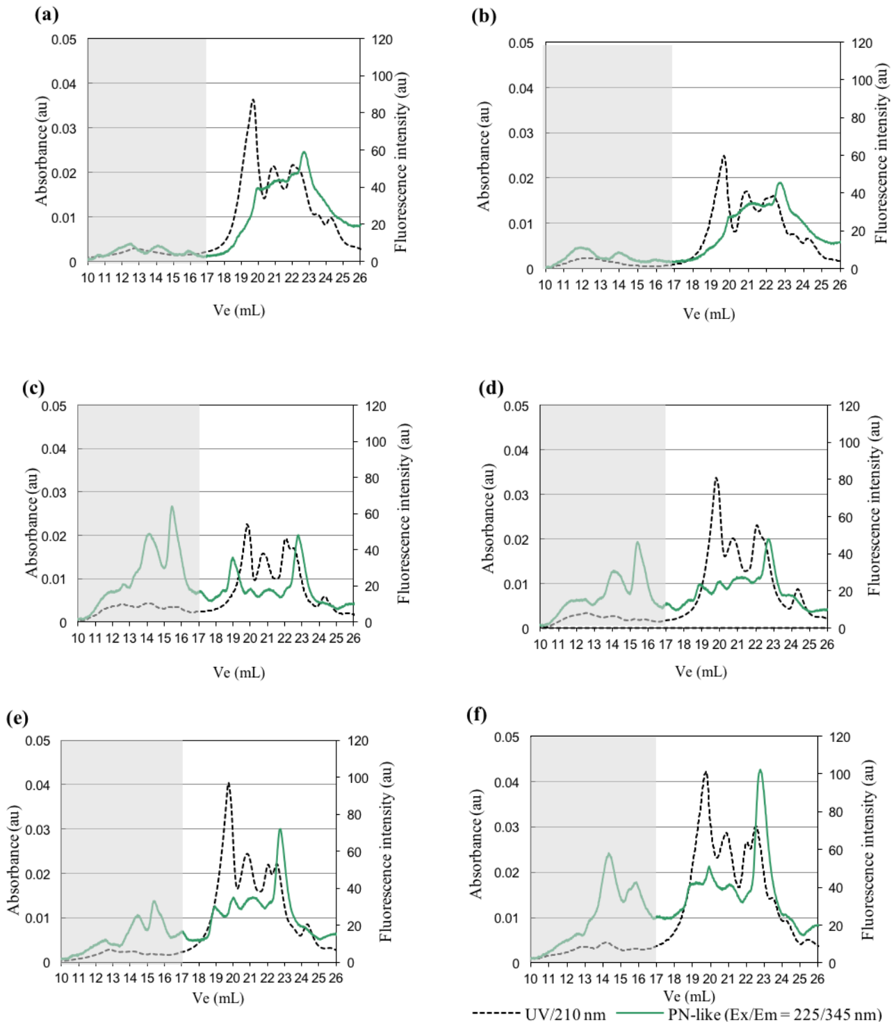
Fig. 5.7 aMW distribution of the EPS extracted from the fungus exposed to sub-toxic concentrations of \text{Ni}^{2+} : (a) 0 mg/L, (b) 0.5 mg/L, (c) 1 mg/L, (d) 5 mg/L, (e) 10 mg/L, and (f) 25 mg/L.
