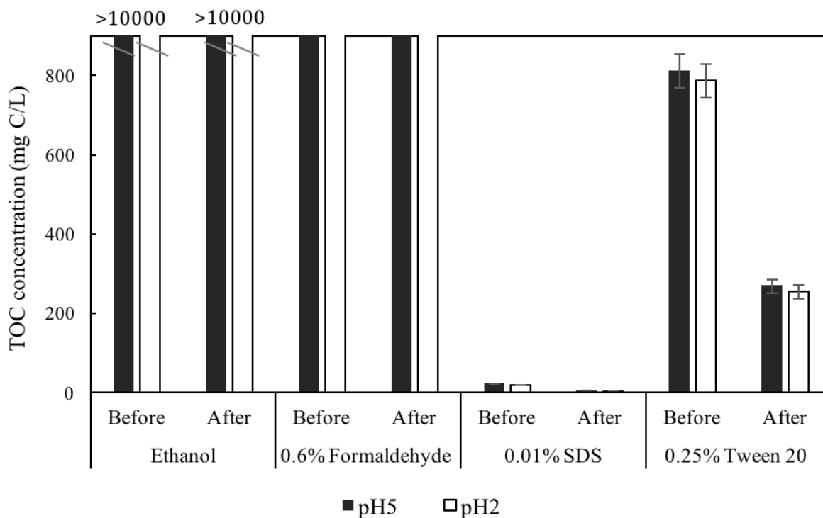
Fig. 3.5 TOC concentration of the organic reagents before and after DAX-8 treatment at pH 5 and pH 2.
