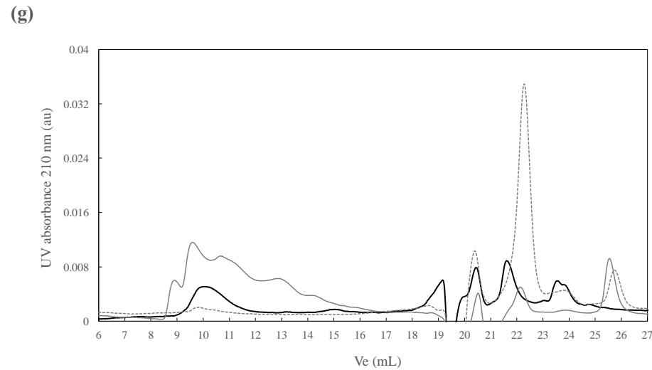
Fig. 3.3 pH effect on the SEC/UV 210 nm fingerprints of EPS extracted by different methods: (a) - centrifugation (d (dilution) 1/1); (b) - heating (untreated EPS, EPS before at pH 5 and pH 2, d 1/50, 1/5 and 1/4, respectively); (c) - sonication (EPS untreated , d 1/3); (d) - ethanol (d 1/1); (e) - F.+heat. (EPS untreated , EPS before at pH 5 and pH 2, d 1/50, 1/5 and 1/4, respectively); (f) - SDS (EPS untreated , d 1/2); and (g) - Tween 20 (EPS untreated , d 1/2).
