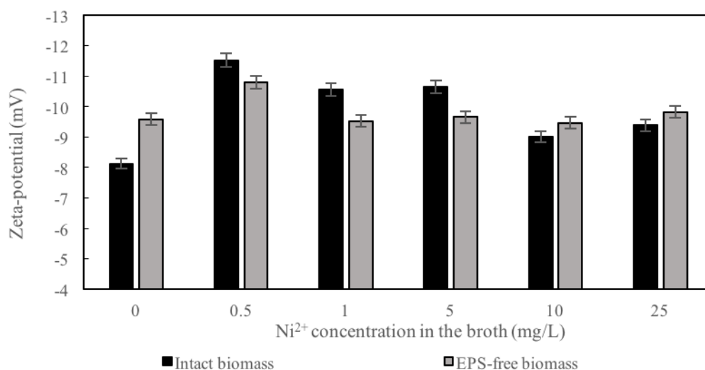
Fig. 5.1 Comparison of zeta-potential between the intact and the EPS-free fungal pellets in the PUM buffer (pH 7.1).
