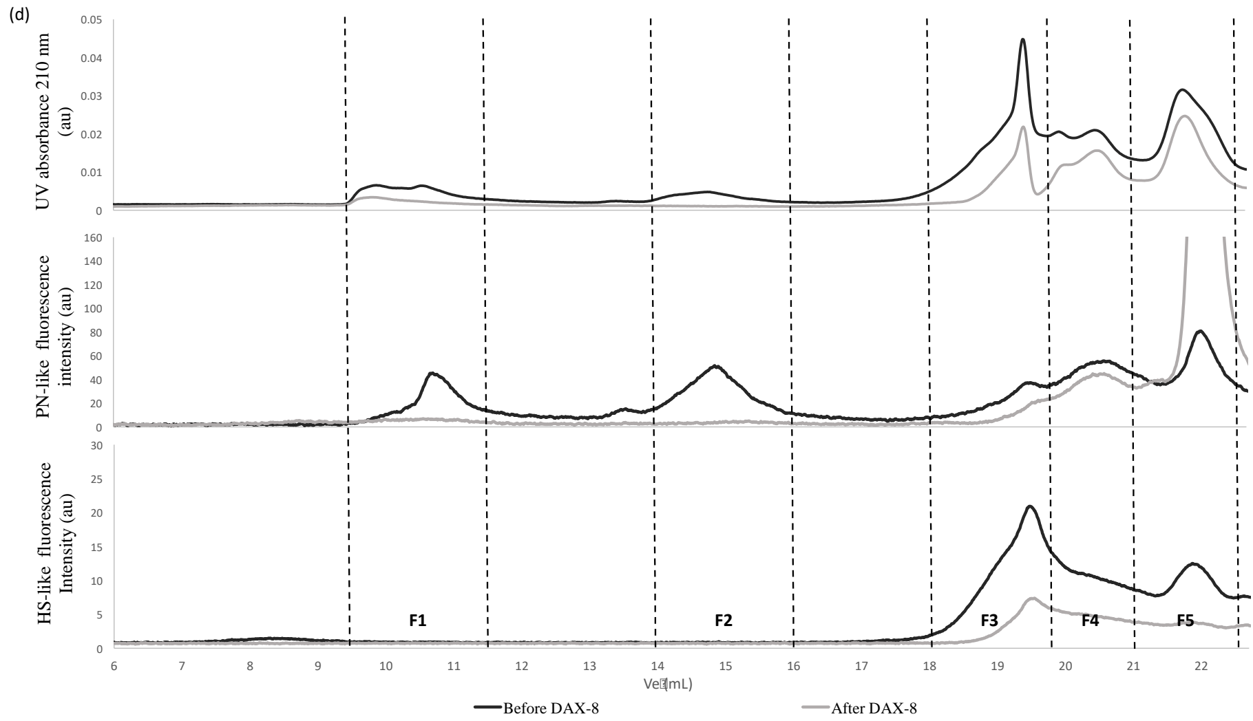
Fig. 4.5 Comparison of SEC/UV 210 nm, PN-like and HS-like fingerprints of EPS before and EPS after : (a) - centrifugation (d 1/1); (b) - heating (d 1/4); (c) - sonication (d 1/1); and (d) - SDS (d 1/1).
