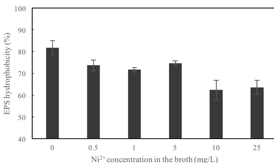
Fig. 5.3 EPS hydrophobicity (%) characterized by DAX-8 resin treatment at pH 2.
