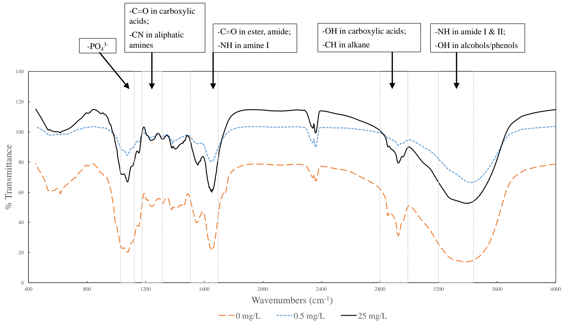
Fig. 5.5 FT-IR spectra of the EPS extracted from the fungus exposed to sub-toxic concentration of Ni 2+ : (a) 0 mg/L, (b) 0.5 mg/L, and (c) 25 mg/L.
