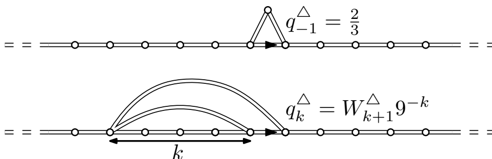
Figure 6.4: The configurations of the triangle incident to the root (up to symmetries).
