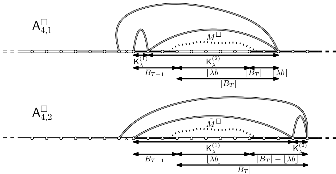
Figure 6.16: The likely subcases on the event A_4^\square .
