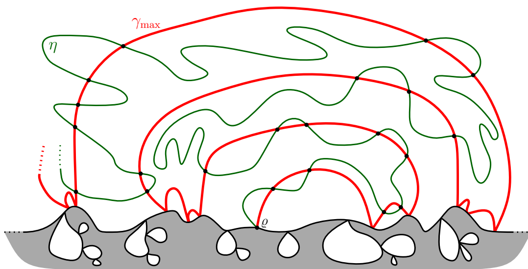
Figure 3.7: The infinite path \eta intersects \gamma_{\max} infinitely many times.
