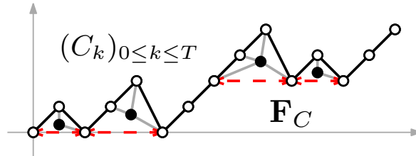
Figure 7.15: The construction of the forest \mathbf{F}_C from the excursion C with C_{T-1} = 4 .
