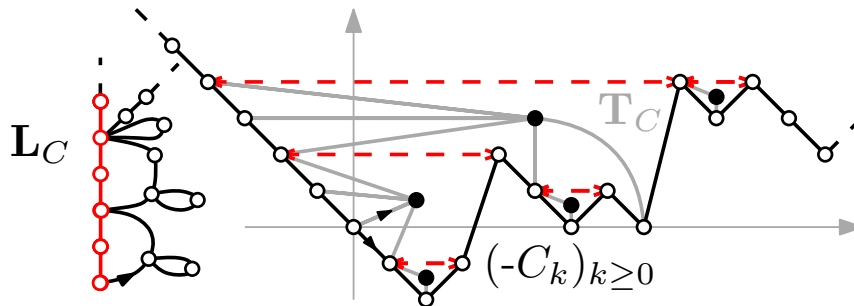
Figure 7.13: The construction of \mathbf{L}_C and \mathbf{T}_C from C .
