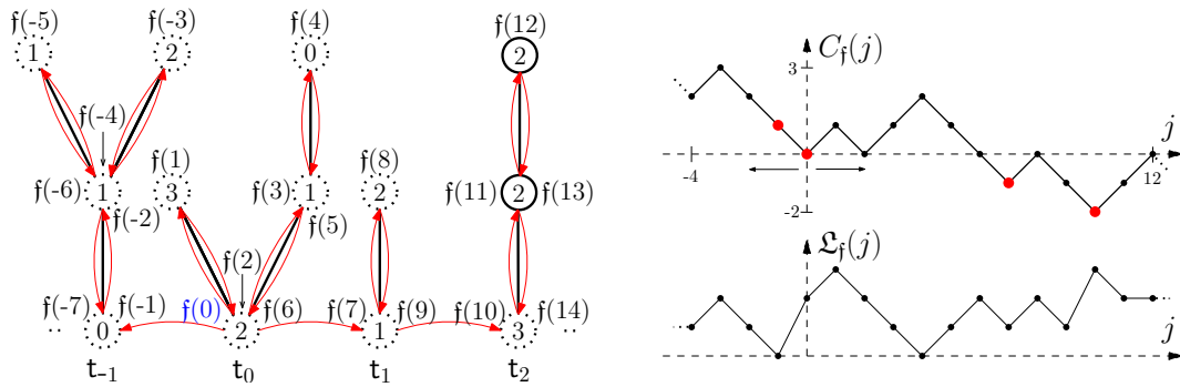
Figure 4.6: Contour and label functions C_f and \mathcal{L}_f of an element ((f, l), b) \in \mathfrak{F}_\infty \times \mathfrak{B}_\infty . The left side depicts the two-sided contour exploration of f . The labels are given by \mathcal{L}_f(j) , where now j \in \mathbb{Z} . The values of the infinite bridge b at its first three down-steps to the right of 0 read here b(d^\downarrow(1)) = 2 , b(d^\downarrow(2)) = 1 and b(d^\downarrow(3)) = 3 , while the first down-step to the left of zero has value b(d^\downarrow(-1)) = 0 . The arrows below the contour function indicate the direction of the encoding, and the red dots mark again the encoding of a new tree.
