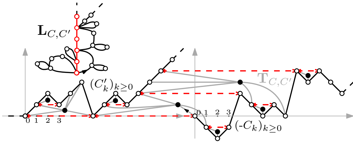
Figure 7.14: The construction of L_{C,C'} and T_{C,C'} from C and C' .
