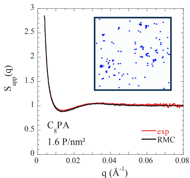
Figure 3.12: RMC fit of the apparent structure factor of C_8PA -grafted NPs at 1.6 \text{ P/nm}^2 . In the inset, a 100 nm-slice of the configuration of NPs in space corresponding to the fit is shown.
