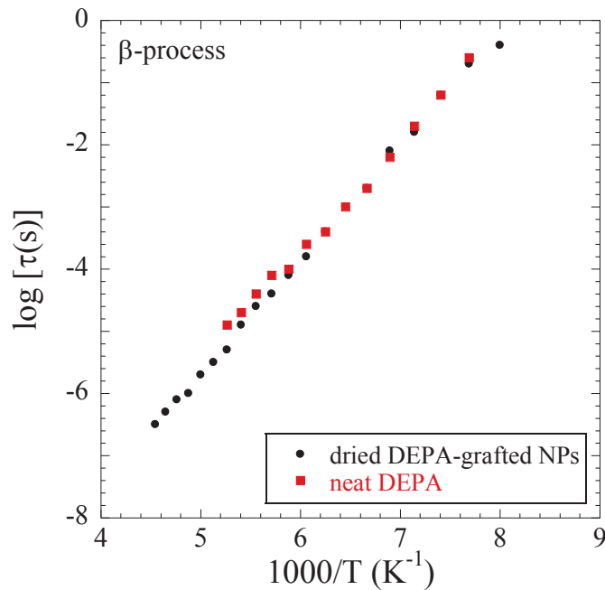
Figure 4.19: Evolution of \log \tau with 1000/T for dried neat DEPA and DEPA-grafted NPs ( 4 \text{ P/nm}^2 ).
