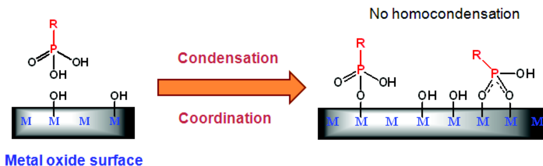
Figure 1.4: Schematic representation of the grafting of phosphonic acids on a metal oxide surface.
