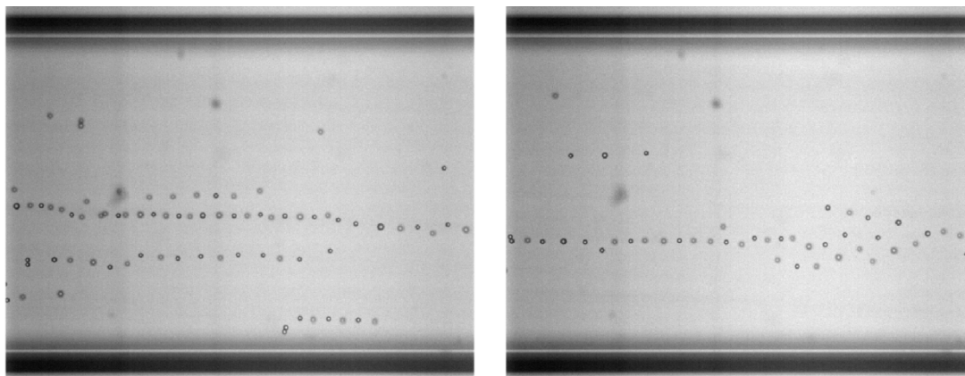
Fig. 4-9 Staggered particle trains in rectangular channels.
