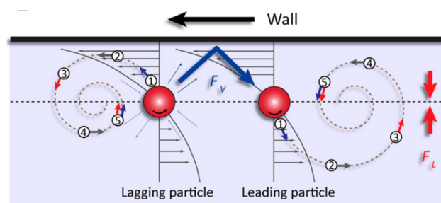
Fig. 4-2 Schematic drawing of the interaction between two aligned particles. (Reprinted from (Lee et al. 2010).)
