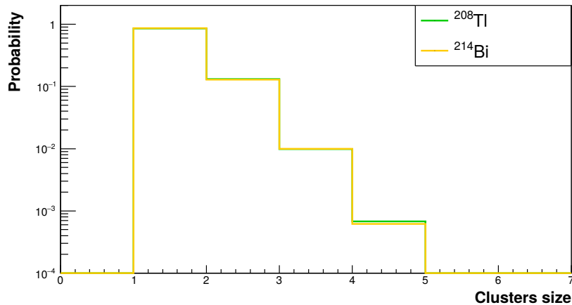
Figure 5.45 – Distributions of the reconstructed cluster sizes for ^{208}\text{Tl} and ^{214}\text{Bi} events.
