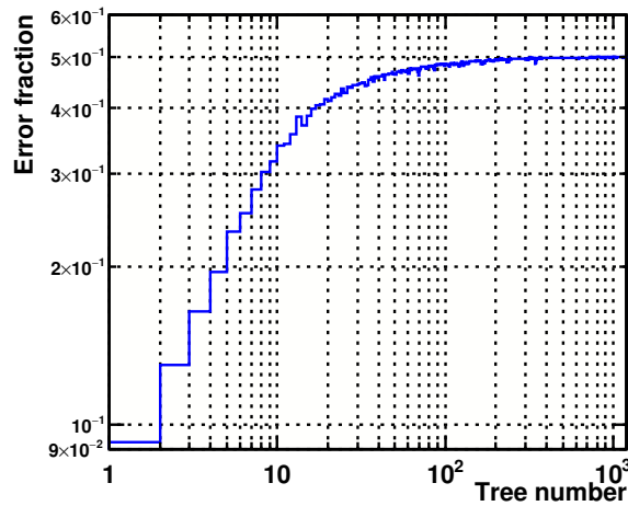
Figure 7.15 – Tree error fraction as a function of the tree generation.
