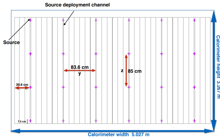
Figure 2.22 – Front view of the source strips. The 24 ^{207}\text{Bi} sources locations are indicated with a pink cross. [59]
