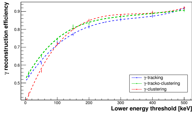
Figure 5.52 – ^{208}\text{Tl} reconstruction efficiency as a function of the lower energy threshold.
