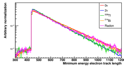
(i) Track length of the minimum energy electron
