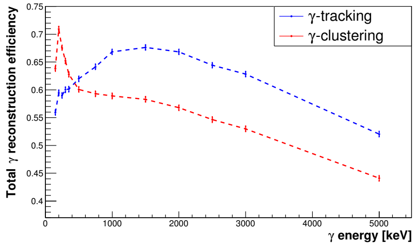
Figure 5.19 – Total \gamma reconstruction efficiency as a function of the 2 \gamma 's energies.
