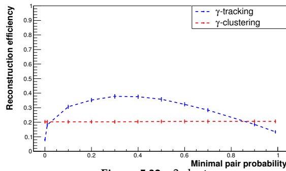
Figure 5.32 – 3 clusters
