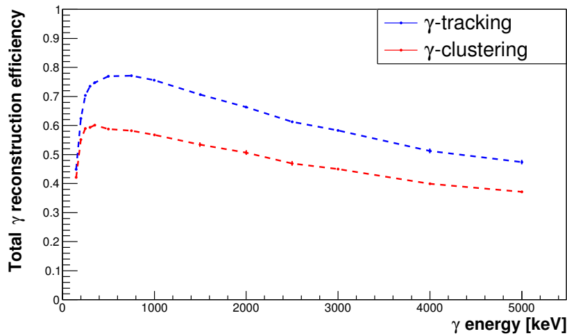
Figure 5.13 – Total \gamma reconstruction efficiency as a function of the \gamma energy.
