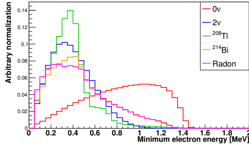
Figure 7.4 – Energy spectra of the lower energy electron for the 0\nu\beta\beta process (in red) and the main backgrounds.
