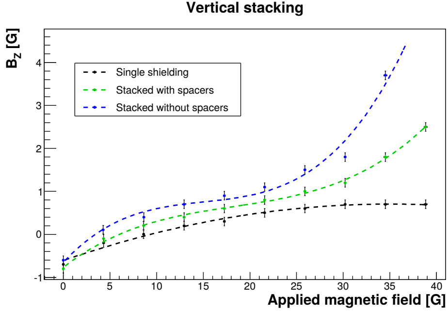
Figure 4.15 – Evolution of the magnetic field measured inside a shielding when subjected to an increasing magnetic field. The black curve represents this evolution for a single shielding. The green and blue curves show the same evolution in the middle shielding of three shieldings stacked vertically, with and without 10 mm spacers respectively.
