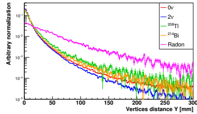
(g) Vertices separation in Y
