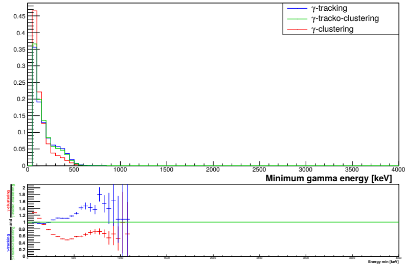
Figure 5.69 – Energy distribution of the \gamma of minimum energy in the 1e3\gamma channel of ^{208}\text{Tl} . All spectra are normalized to 1. The lower plot shows the ratio of the \gamma -tracking spectrum with the \gamma -tracko-clustering spectrum (in blue) and the ratio of the \gamma -clustering spectra with the \gamma -tracko-clustering spectra (in red).
