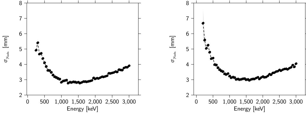
Figure 4.22 – Horizontal spatial resolution of the calorimeter vertex, as a function of the reconstructed electrons energy, with a uniform magnetic field ( left ) or a polynomial magnetic field ( right ) [92].
