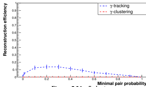
Figure 5.34 – 5 clusters
