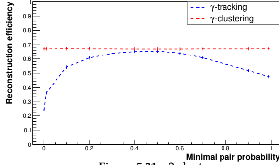
Figure 5.31 – 2 clusters
