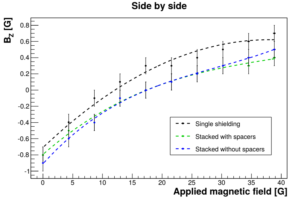
Figure 4.16 – Evolution of the magnetic field measured inside a shielding when subjected to an increasing magnetic field. The black curve represents this evolution for a single shielding. The green and blue curves show the same evolution in the middle shielding of three shieldings put side by side, with and without 10 mm spacers respectively.
