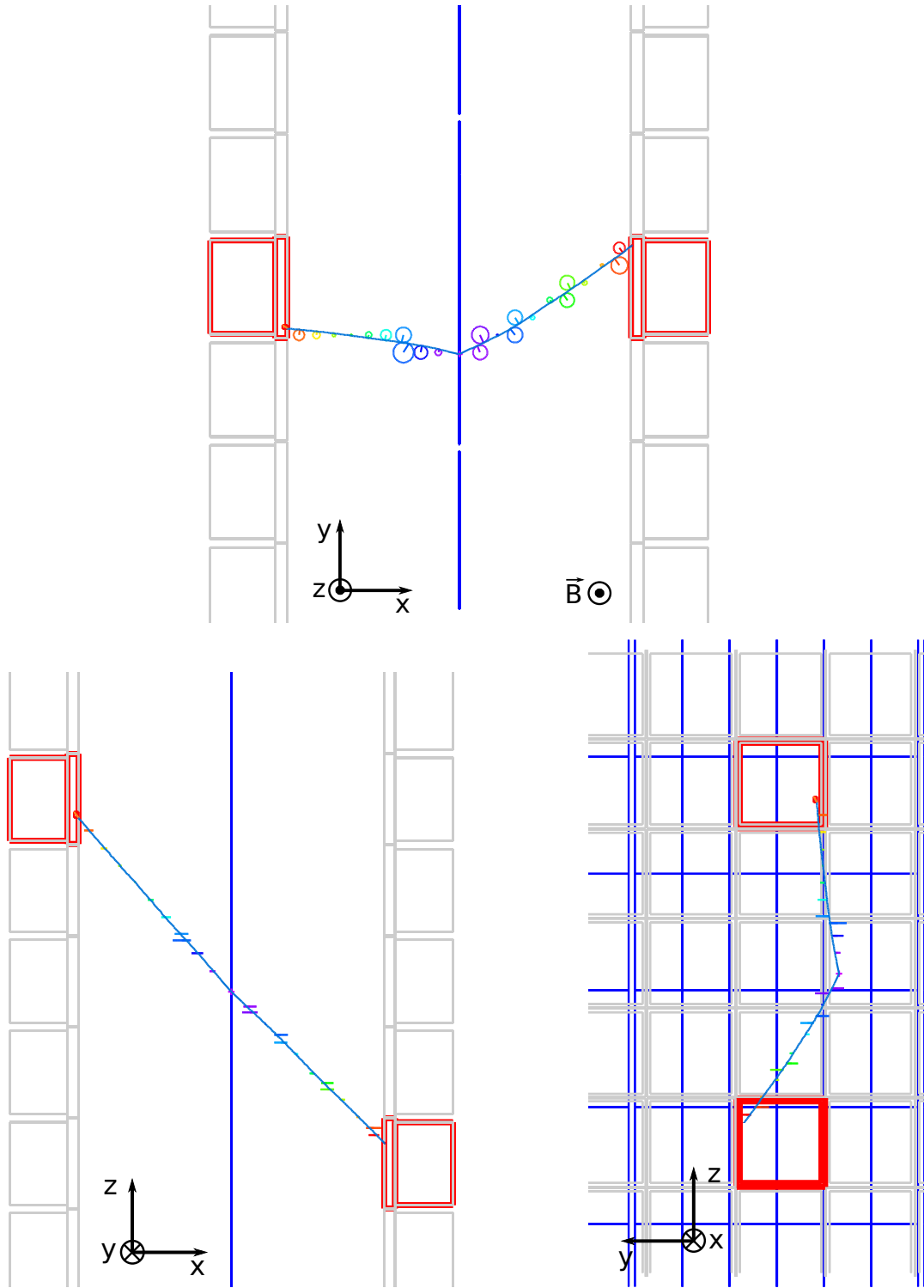
Figure 3.1 – Display of a simulated 0\nu\beta\beta event in the SuperNEMO demonstrator. (left) Top view. (middle) Side view. (right) Front view. The calorimeter PMTs, the side and top scintillator blocks and the tracker cells are not represented for sake of readability. The source is displayed in blue and the different source pads are distinguishable. The scintillators are displayed in gray. The two simulated electrons tracks are blue and the colored circles represent the tracker cells they have crossed.
