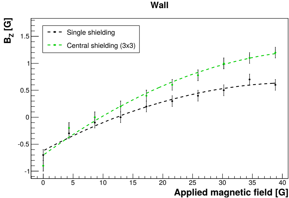
Figure 4.17 – Evolution of the magnetic field measured inside a shielding when subjected to an increasing magnetic field. The black curve represents this evolution for a single shielding. The green curve shows the same evolution in the central shielding of a 3 \times 3 configuration, where the shieldings are separated with 10 mm spacers.
