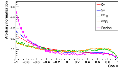
(d) Cosine of the angle between the electrons
