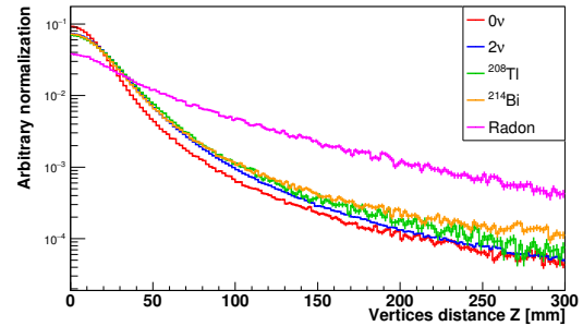
Figure 7.11 – Vertical ( Z ) source vertices separation distributions for the 0\nu\beta\beta process (in red) and the main backgrounds.
