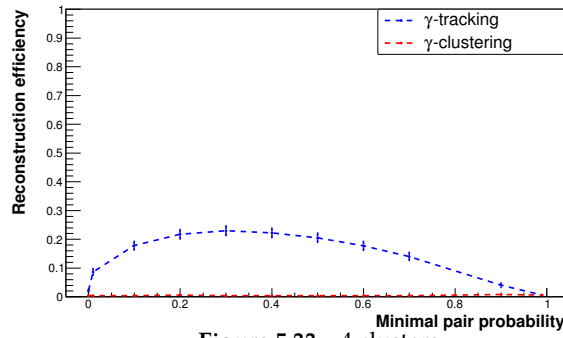
Figure 5.33 – 4 clusters
