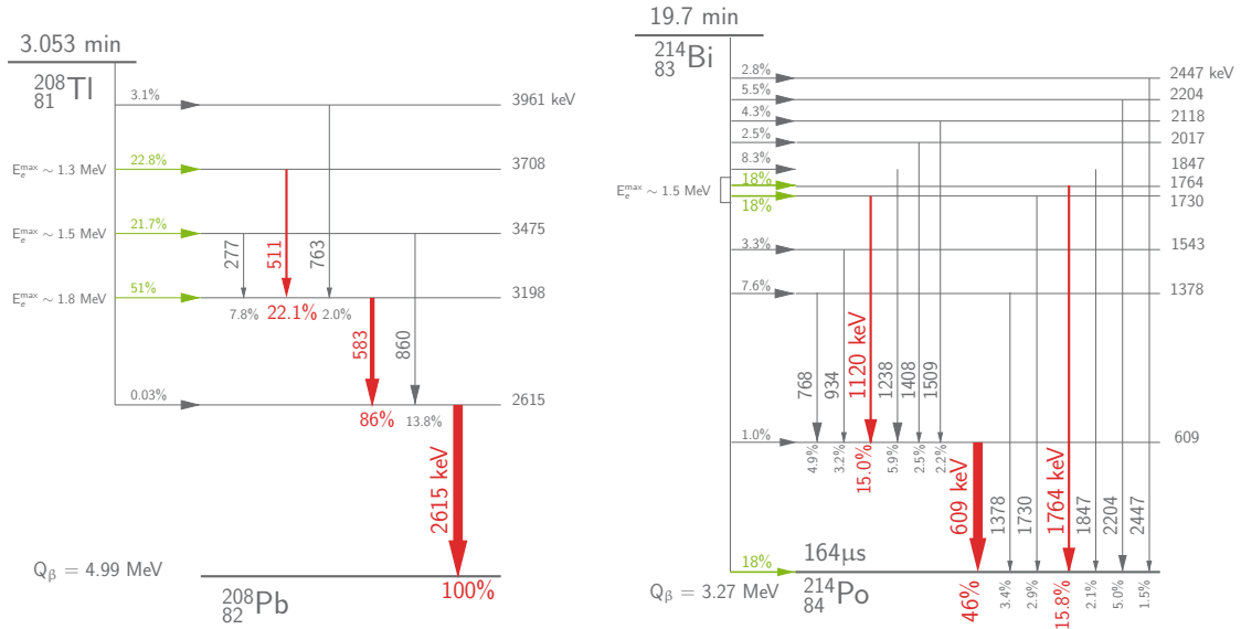
Figure 2.27 – Decay schemes of ^{208}\text{Tl} (left) and ^{214}\text{Bi} (right). The most frequently emitted \gamma 's, along with their percentage of occurrence, are highlighted in red.
