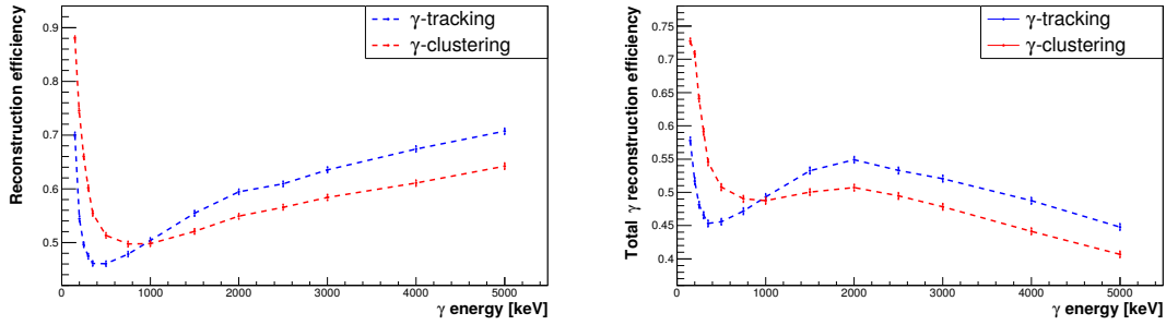
Figure 5.25 – Reconstruction efficiency (left) and total \gamma reconstruction efficiency (right) as a function of the 3 \gamma 's energies.
