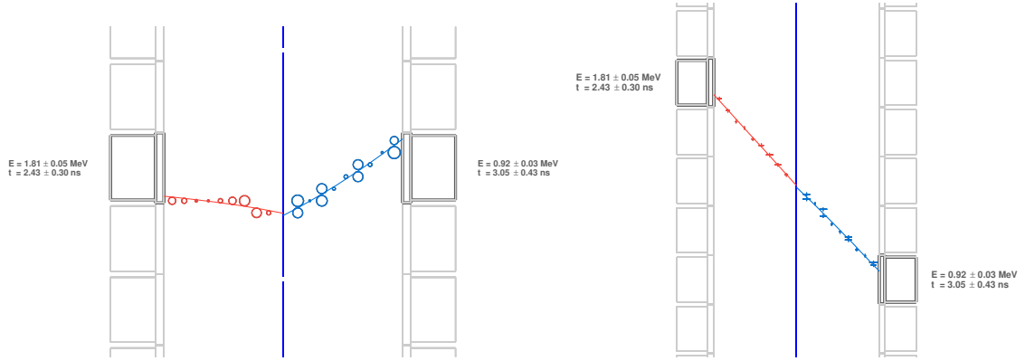
Figure 3.4 – Display of the same simulated event as in Figure 3.1 after application of the tracker trajectory fitting algorithm. (left) Top view. (right) Front view. Two helices are identified as the best fits for the two clusters.
