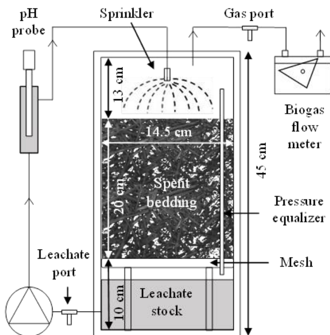
Figure 19: Experimental leach-bed reactor (LBR)
