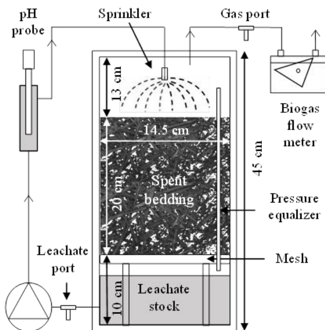
Figure 10 : Experimental leach-bed reactor
