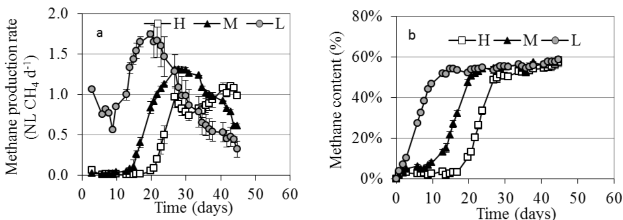
Figure 30 : Biogas parameters monitored during the digestion process considering three different fractions of easily-degradable substrate loaded in the LBRs: (H), medium (M) and low (L). (a) Methane production rates and (b) methane content in the biogas.
