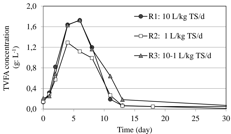
Figure 17 : Volatile fatty acids concentration in three LBRs with different internal leachate recirculation conditions
