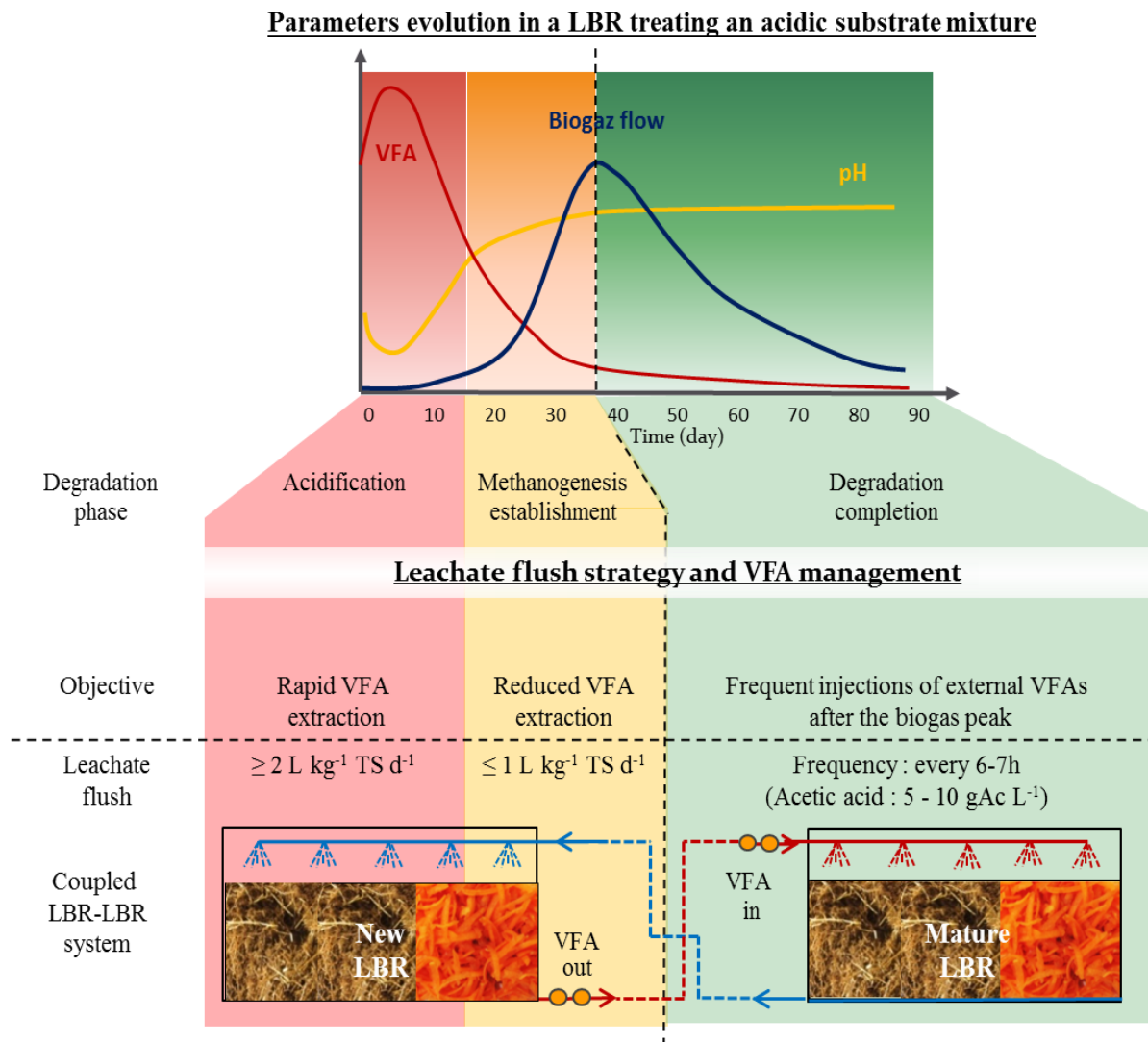
Figure 42 : Parameters evolution in a LBR treating an acidic mixture of spent cow bedding and an easily-degradable substrate; leachate flush and VFA management in relation to the phase of degradation; schematic functioning of a coupled LBR-LBR system: the new reactor from where VFAs are extracted and the mature reactor where VFAs are consumed
