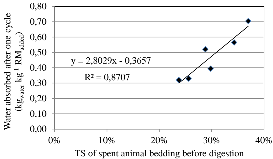
Figure 15 : Amount of water absorbed after one cycle by the bulk in relation with its total solids (TS) before digestion
