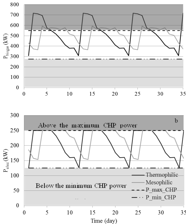
Figure 28 : Comparison of a simulated industrial plant operated in mesophilic and thermophilic conditions. The simulation, based on the data from run1, consider the treatment of 9,400 tons/year of spent cow bedding, the installation of a combined heat and power (CHP) unit of 250 kW el and the use of 4 digesters staggered in time with a batch duration of 44 days. (a) heat power contained in the cumulated biogas at the inlet of the CHP unit; (b) electrical power produced considering the CHP power working range: the maximum (P max_CHP ) and the minimum (P min_CHP )
