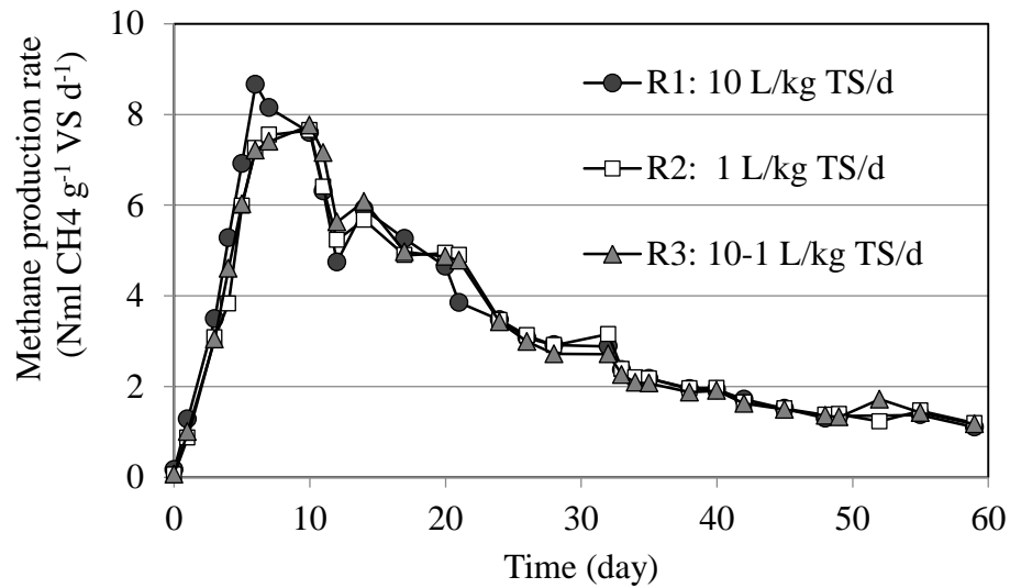
Figure 16 : Methane production rates of three LBRs with different internal recirculation conditions
