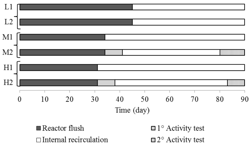
Figure 33 : Experimental planning and configuration. Three conditions are tested in duplicate: in L1–L2 a low leachate flush rate is applied (0.5 L kg -1 TS d -1 ), in M1–M2 a medium leachate flush rate is applied (1.0 L kg -1 TS d -1 ) and in H1– H2 a high leachate flush rate is applied (2.0 L kg -1 TS d -1 ). During the “reactor flush” period, a fresh leachate is pumped in and out every day while, during the “internal recirculation” period, the same leachate is recirculated through the bed. Additionally, M2 and H2 are used to carry out an activity test.
