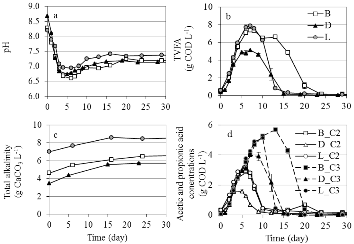
Figure 21 : Comparison of the leachate parameters analysed all along the digestion process of three different experimental loadings: spent cow bedding and water (B), spent cow bedding and leachate (L) and spent cow bedding and digestate (D). (a) pH; (b) total volatile fatty acid concentration; (c) total alkalinity; (d) acetic (C2) and propionic (C3) acid concentrations
