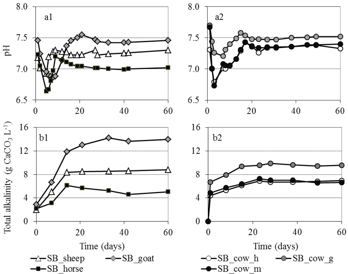
Figure 11 : Parameters monitored in the leachate during the digestion process in a LBR of six different spent animal bedding: (a1 - a2) pH and (b1 - b2) total alkalinity in g CaCO 3 L -1
