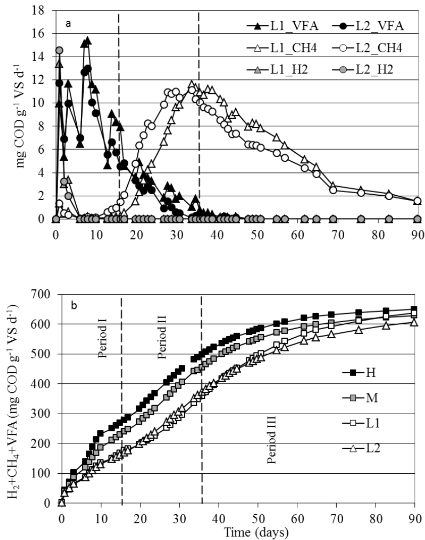
Figure 36 : Dynamic presentation of all the metabolites extracted or produced during the digestion process: (a) extraction rate of volatile fatty acids (VFAs), and production rate of methane ( CH_4 ) and hydrogen ( H_2 ) in conditions L1 and L2; (b) accumulated amounts of VFAs, CH_4 and H_2 over time. H and M refers to the mean value of H1- H2 and M1 - M2, respectively, during period I and period II while, they correspond to only H1 and M1, respectively, during period III
