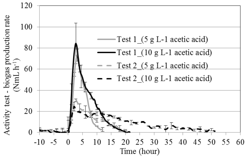
Figure 35 : Activity test: biogas production rate after injection of leachate containing acetic acid. 1 st injection is effectuated after the methane peak (after about 30 days) and 2 nd injection at the end of digestion (after about 80 days). Two acetic acid concentrations in the leachate were tested: 5 \text{ g L}^{-1} and 10 \text{ g L}^{-1} .
