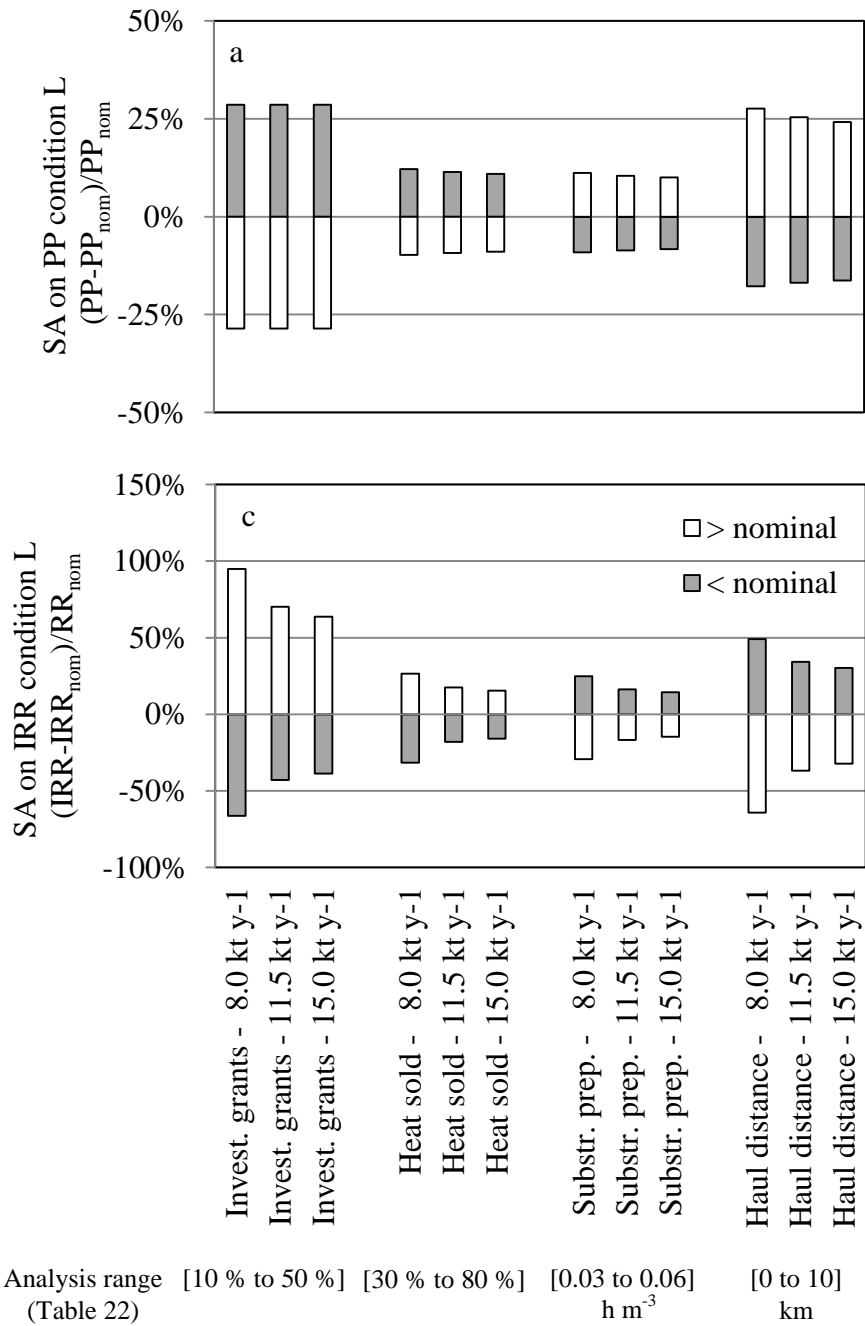
Figure 43 : Sensitivity analysis results: variability of the IRR and PP for three capacities: (8.0, 11.5, 15.0) kt y -1 . (a-b) Payback Period for condition D and L; (c-d) Internal Rate of Return for conditions D and L
