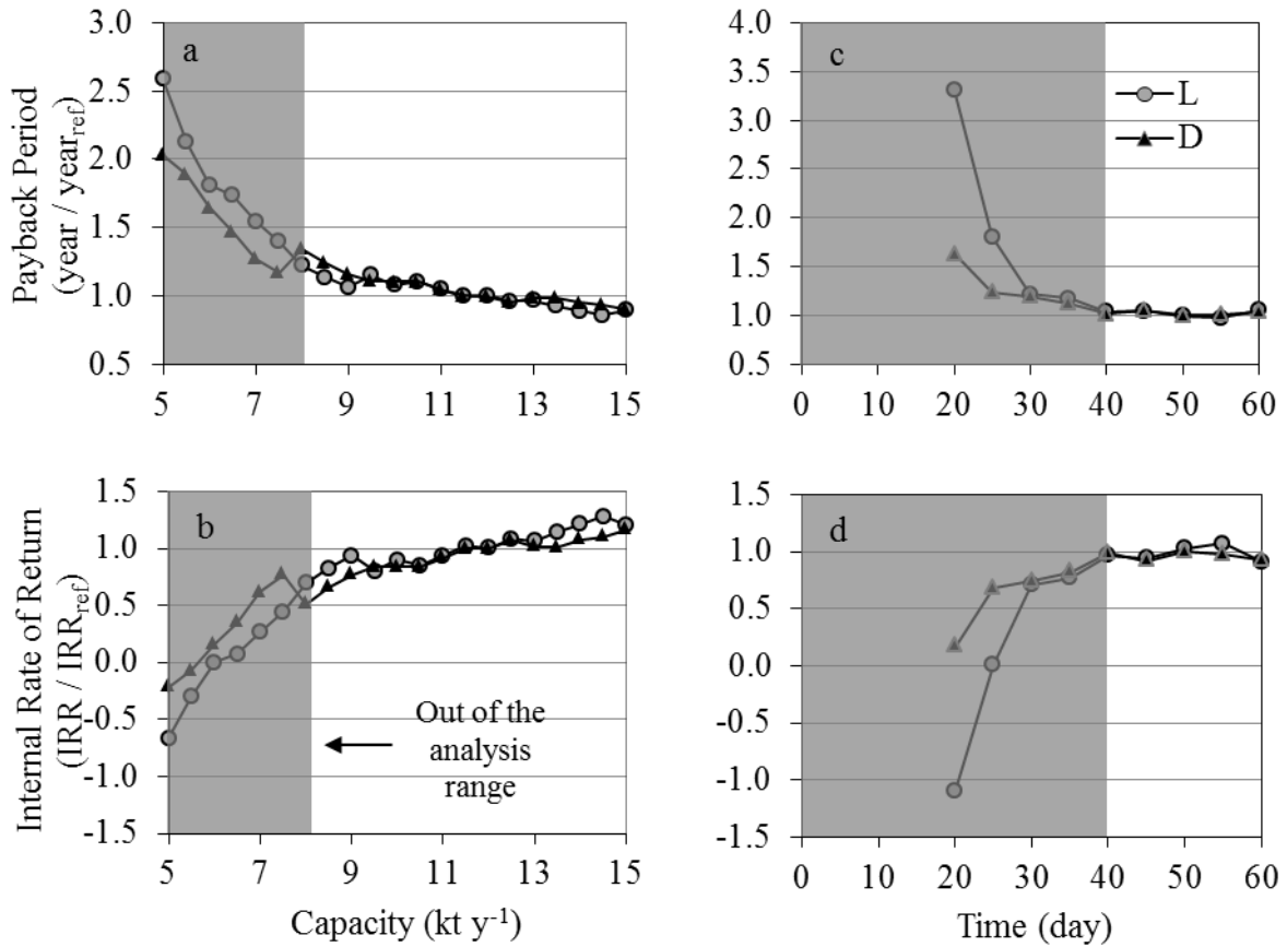
Figure 22 : Results of the economic simulation performed on an industrial site using a sequential LBR process considering a digester number varying from 4 to 9 and an electric cogeneration power ranging from 100 to 300 kW el . Evolution of the (a) Payback Period and Internal (b) Rate of Return in relation to the annual capacity. Evolution of the (c) Payback Period and (d) Internal Rate of Return in relation to the batch duration
