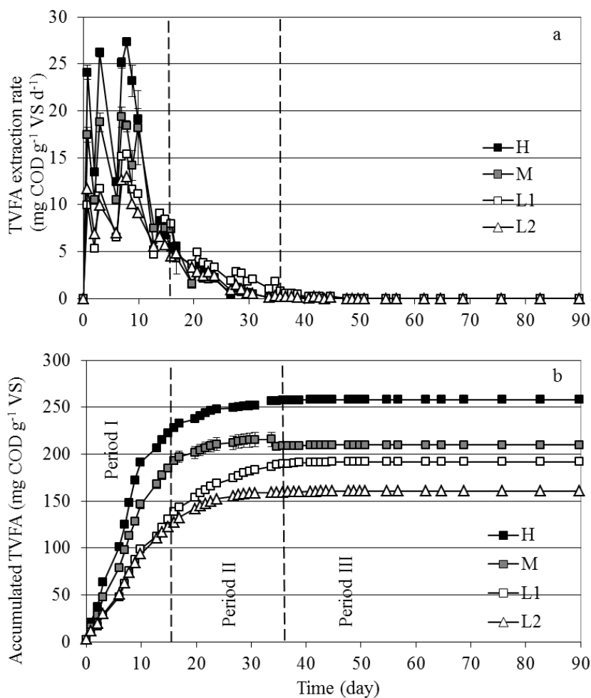
Figure 37 : Dynamic presentation of total volatile fatty acids (TVFA) extracted: (a) extraction rate of TVFA; (b) accumulated TVFA extracted over time. H and M refers to the mean value of H1- H2 and M1- M2, respectively, during period I and period II while, they correspond to only H1 and M1, respectively, during period III
