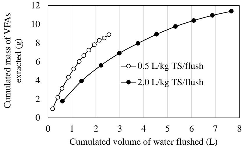
Figure 38 : Cumulated mass of VFAs extracted from a LBR after several flushes
