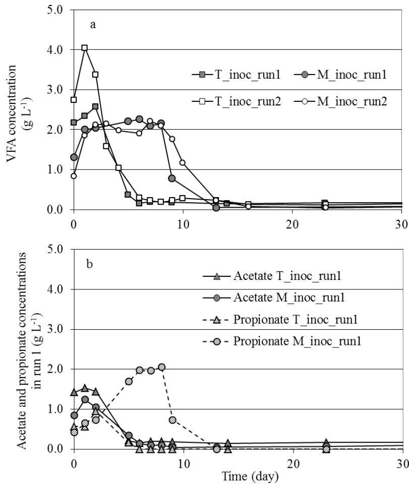
Figure 27 : Comparison of mesophilic (M_inoc) and thermophilic (T_inoc) conditions: (a) VFA concentration in run 1 and run 2; (b) acetate and propionate concentrations in run 1
