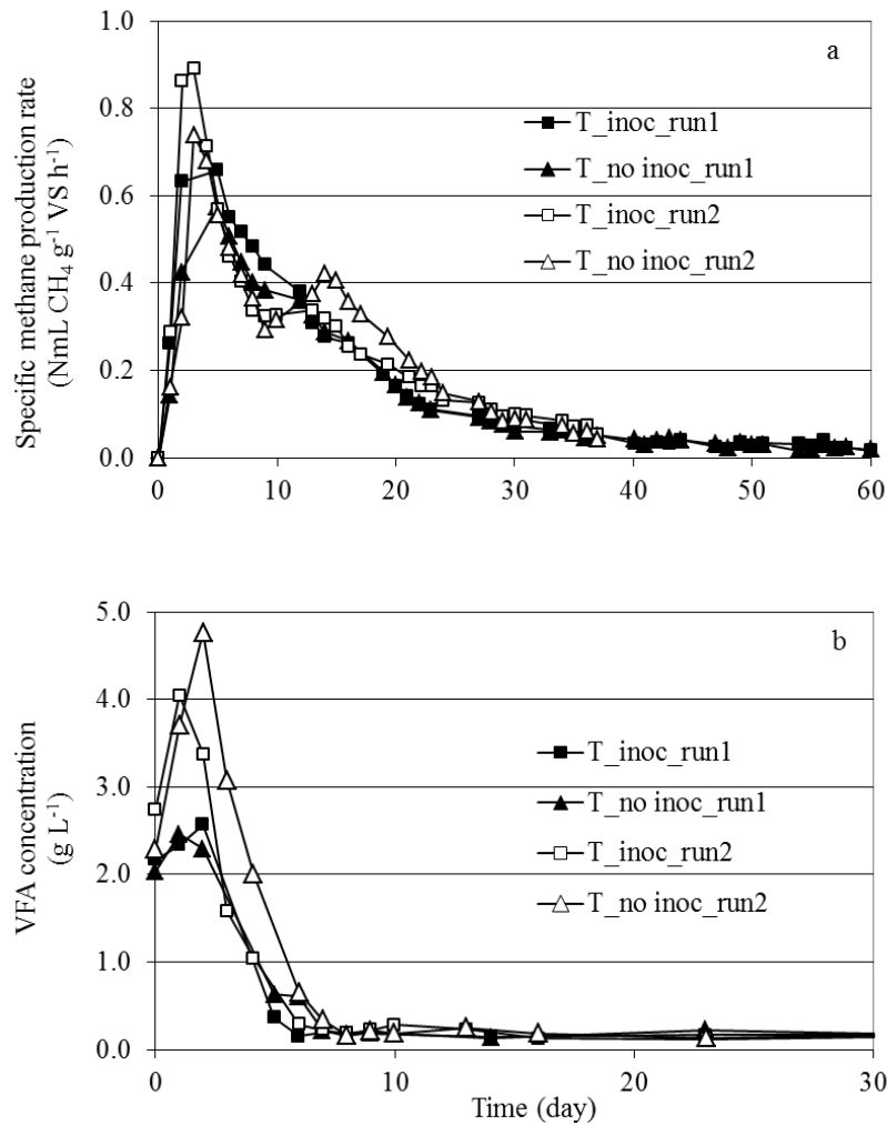
Figure 25 : Comparison of thermophilic conditions with (T_inoc) and without (T_no inoc) solid digestate, in run 1 and run 2: (a) specific methane production rate; (b) VFA concentration
