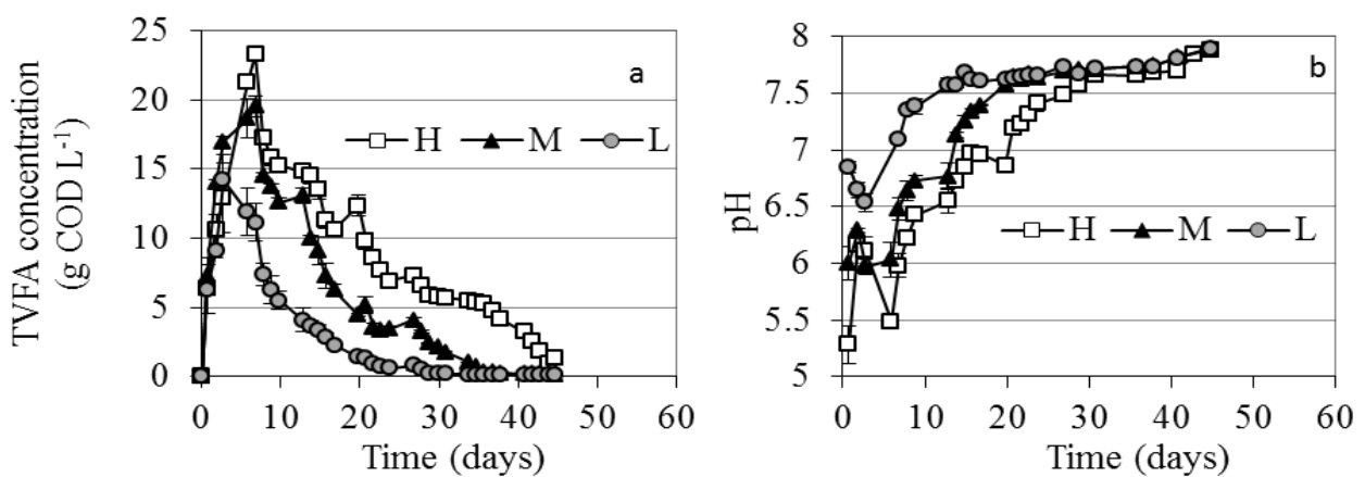
Figure 31 : Parameters monitored in the leachate during the digestion process considering three different fractions of easily-degradable substrate loaded in the LBRs: high (H), medium (M) and low (L). (a) Volatile fatty acids concentration and (b) pH of the leachate in LBRs with different fractions of easily-degradable substrate
