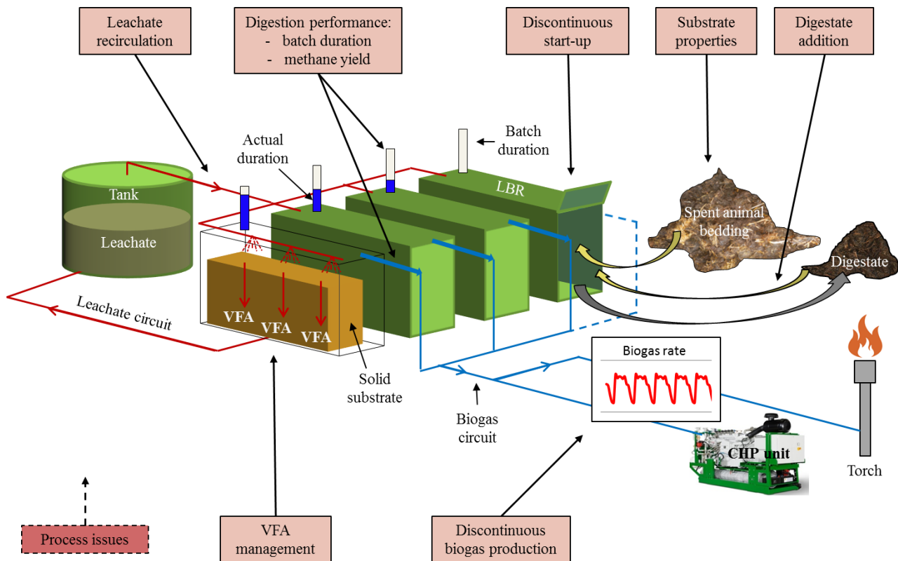
Figure 3: Operating principle of the Naskeo/Methajade sequential LBRs process
