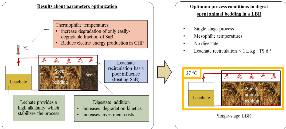
Figure 40 : Results of the parameters optimization and optimum process conditions to digest spent animal bedding in a LBR
