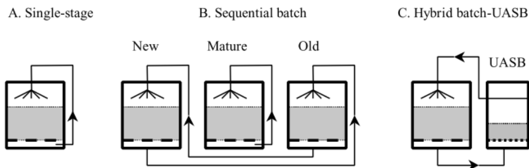
Figure 2: Existing LBR configurations (Vandevivere et al., 2003)
