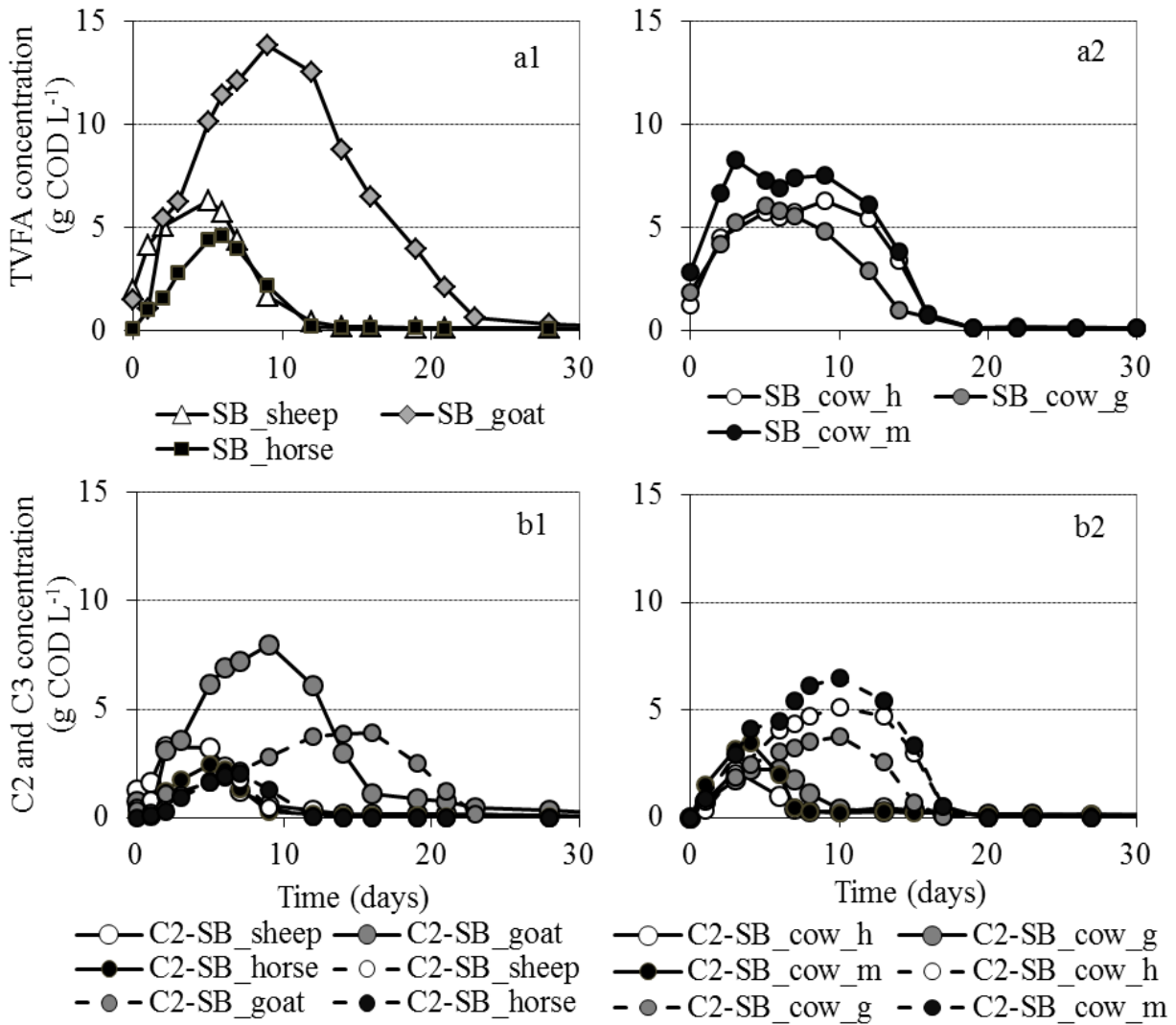
Figure 12 : Volatile fatty acids measured in the leachate during the digestion process in a LBR of six different spent animal bedding: (a1 - a2) total volatile fatty acids concentration in g COD L -1 , (b1 - b2) acetic (C2) and propionic (C3) acid concentrations in g COD L -1
