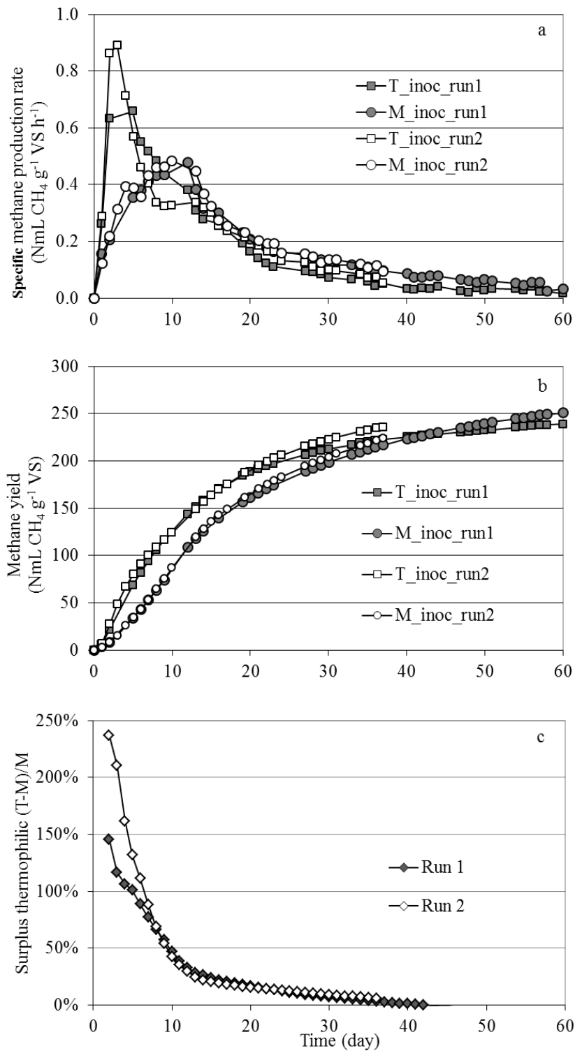
Figure 26 : Comparison of mesophilic (M_inoc) and thermophilic (T_inoc) conditions, in run 1 and run 2: (a) specific methane production rate; (b) methane yield; (c) additional methane yield in thermophilic conditions
