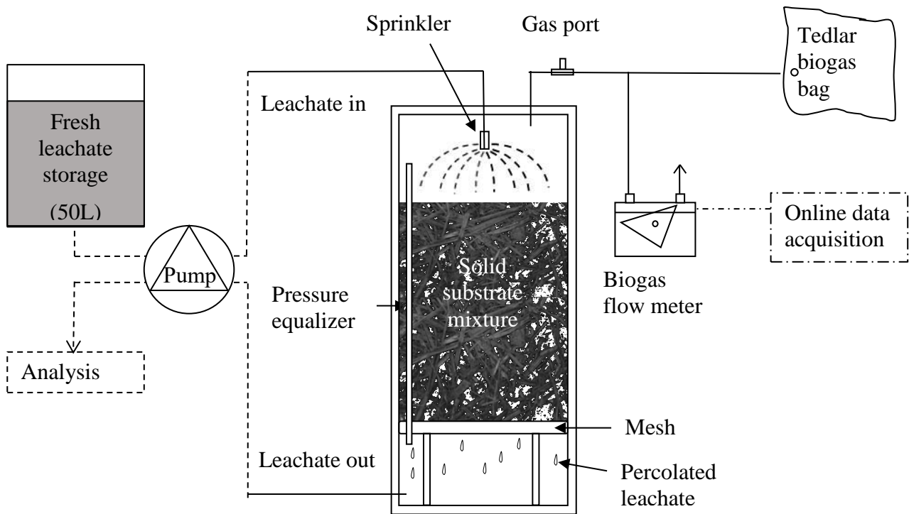
Figure 32 : Experimental design. Fresh leachate without volatile fatty acids (VFAs) is stored in a 50 L volume. A fixed amount of leachate is pumped into the leach-bed reactor (LBR) through a peristaltic pump. After percolation through the bed, the leachate enriched in VFAs is pumped out and analysed.
