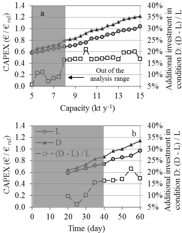
Figure 23 : Results of the economic simulation performed on an industrial site using a sequential LBR process considering a digester number varying from 4 to 9 and an electric cogeneration power ranging from 100 to 300 kW el . Evolution of the CAPEX in relation to (a) the annual capacity and (b) the batch duration
