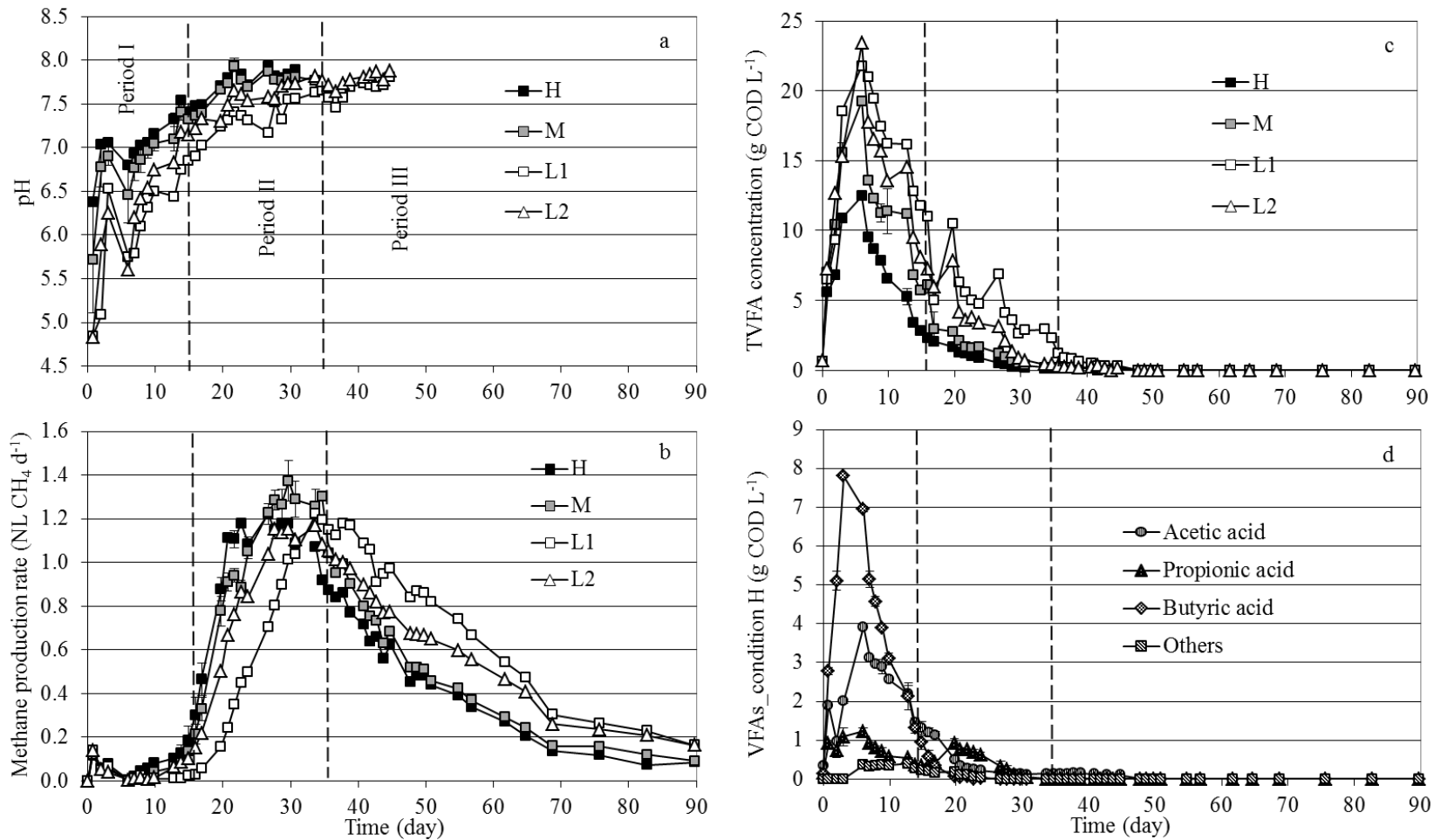
Figure 34 : Parameters measured during the digestion process: (a) pH; (b) methane production rate; (c) total volatile fatty acids (TVFA) concentration; (d) volatile fatty acids (VFAs) concentration (condition H). H and M refers to the mean value of H1- H2 and M1 - M2, respectively, during period I and period II while, they correspond to only H1 and M1, respectively, during period II
